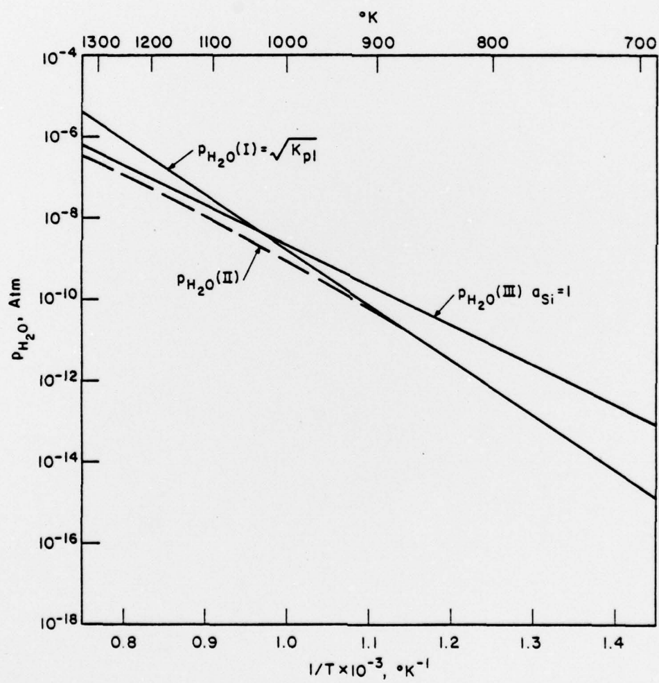
Fig. 12. Equilibrium partial pressures of H_2O for H_2 with very low H_2O content.
