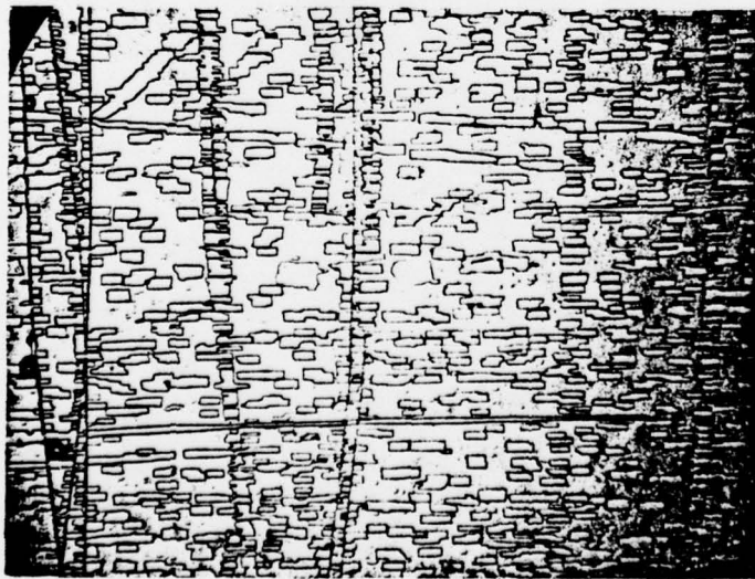
Fig. 5. Discontinuous hillock growth on an oxidized substrate, #30.
