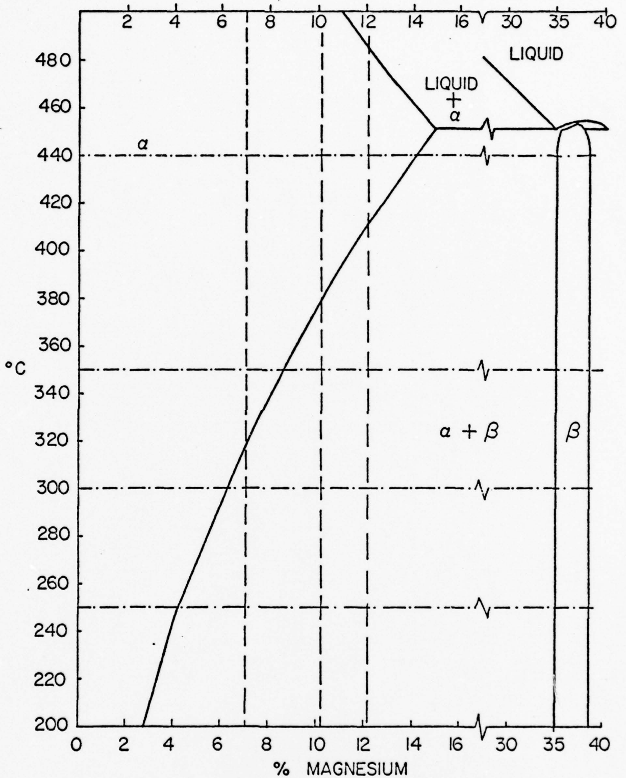
Fig. 1. A partial Aluminum-Magnesium phase diagram. Compositions and working temperatures are indicated by dashed lines and dot-dash lines, respectively, and represent a matrix of material compositions and processing temperatures.
