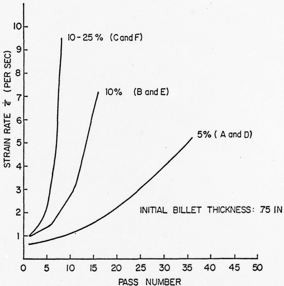
Fig. 4. This figure depicts the average strain rate resulting from rolling schedules used to process 7% Mg alloys. Rolling billets had an initial thickness of .75 inches. Curves were calculated assuming hot rolling conditions; the letters A, B and C refer to a 7% Mg alloy rolled at 300°C, and D, E, and F, at 250°C.
