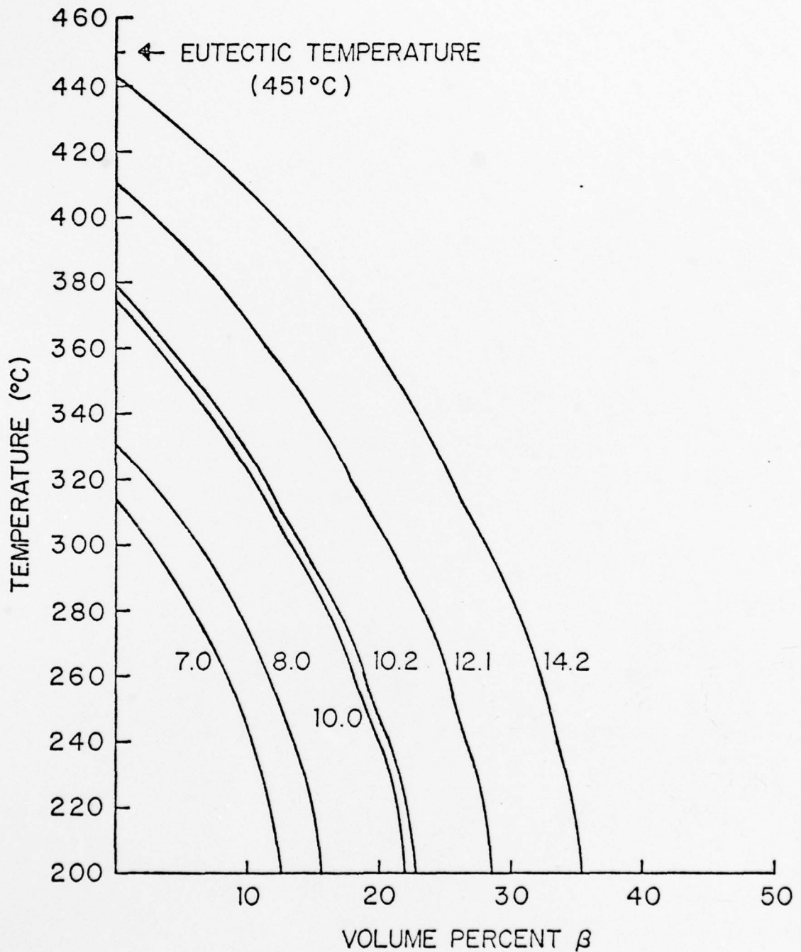
Fig. 3. These curves reflect the volume percentage of an Al-Mg alloy microstructure which would be Beta phase, or the intermetallic compound \text{Al}_3\text{Mg}_2 , if the system were at equilibrium.
