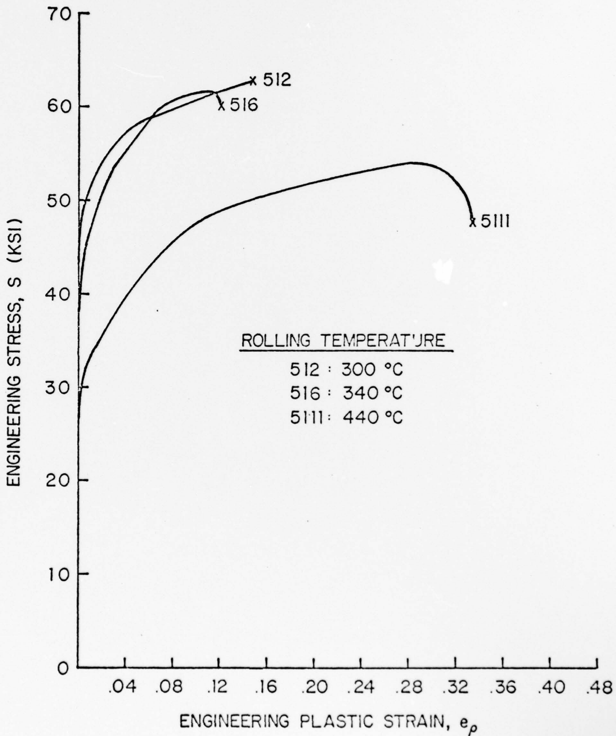
Fig. 17. This figure demonstrates the effect of rolling temperature on engineering stress-strain curves. All specimens are of the same composition and received essentially the same thermomechanical process with the exception of rolling temperature. Sample 5111 has a fully recrystallized microstructure.
