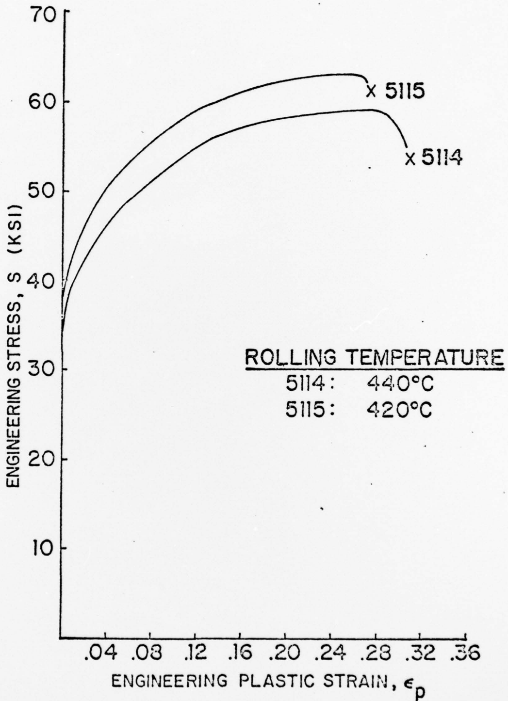
Fig. 24. Engineering stress strain curves for specimens 5114 and 5115. These curves illustrate the change in tensile properties due to rolling temperature. 5114 was finished at 440°C and 5115 was finished at 420°C.
