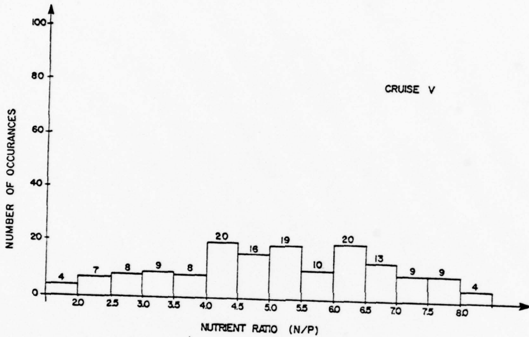
Figure 15. Cruise V nutrient ratio frequency chart for open ocean waters.
