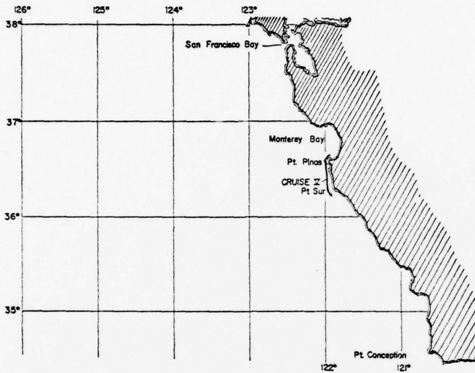
Figure 12. Cruise V ship's track.
