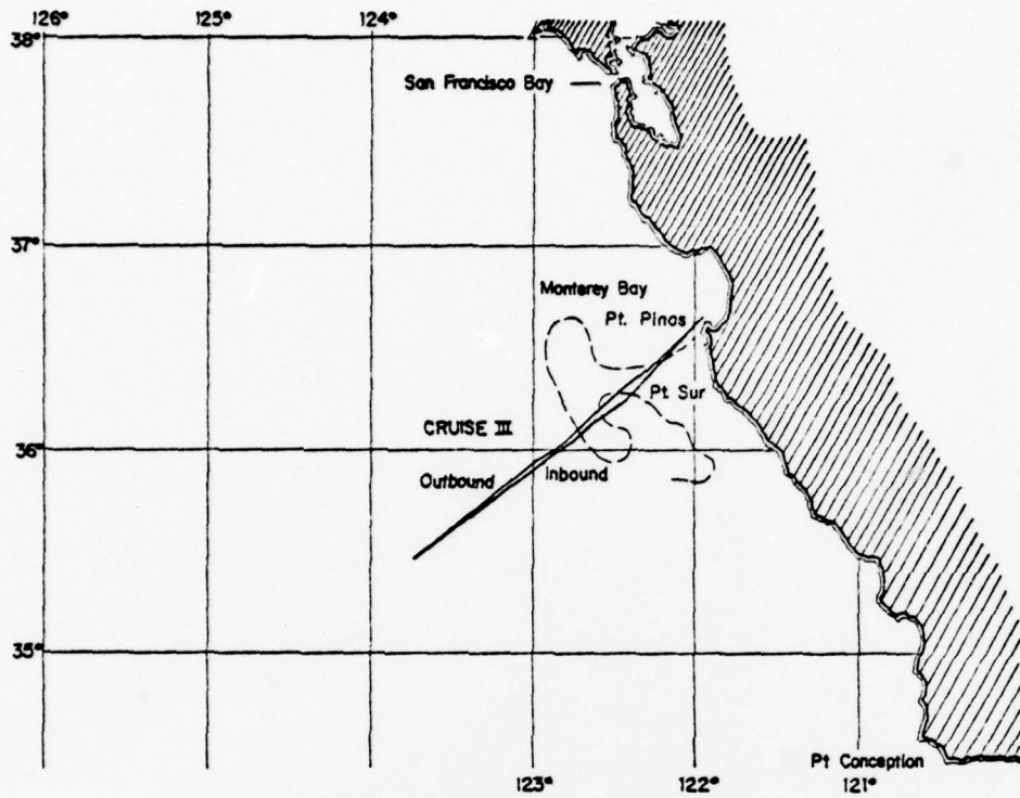
Figure 3. Cruise III ship's track (solid line) and outline of upwelling "plume" (dashed line).
