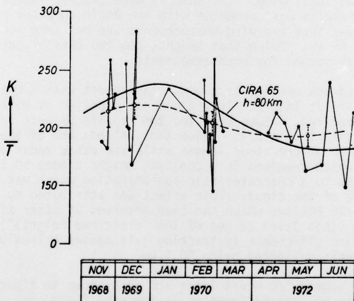
Figure 10. Comparison between mean values of temperature at noon derived from foil cloud data and CIRA 65 data. Dashed curve: freehand curve laid through our foil cloud data. White points with error bars: means of foil cloud data. (Height intervals of averaging correspond to fig 8.)
