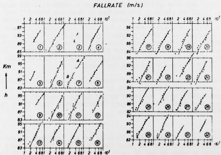
Figure 8. Variations of fall rate measurements performed over El Arenosillo, indicating turbulent motions (curve of best fit is entered into data points). The numbers indicate the chronological sequence.
