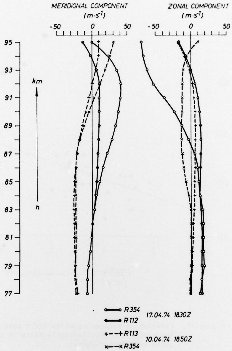
Figure 12. Wind measurements done with falling spheres over White Sands, Apr 74.
