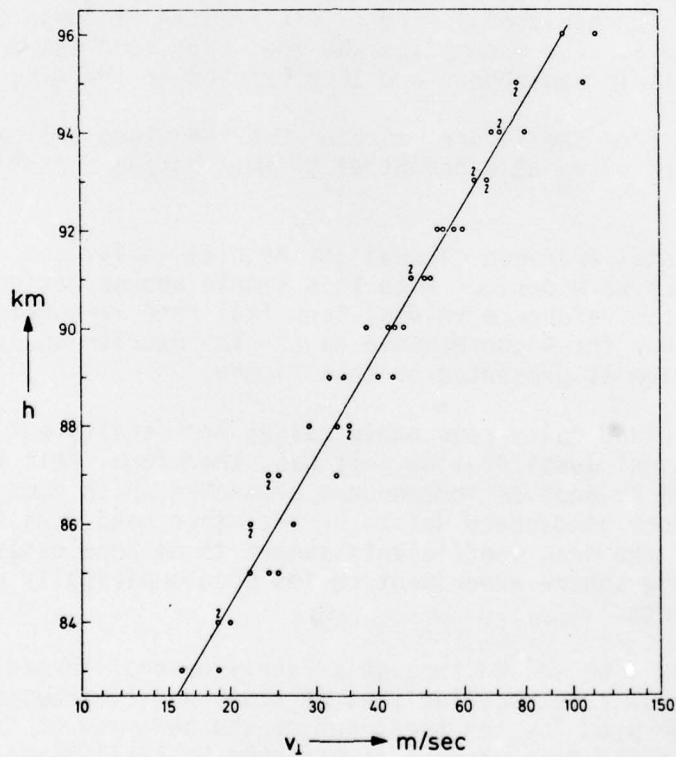
Figure 4. Variation of fall rate observed at 20.00 GMT on 4 consecutive days. Numbers in figure over or under points: number of identical values measured. El Arenosillo, Feb 70. Compare data scatter with those of fig 7.
