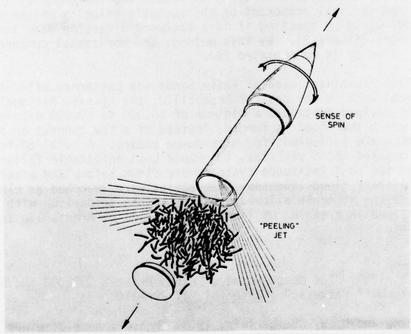
Figure 2. Method of foil cloud generation: the payload is separated from the rocket. After 2 s, gas vessels are opened. The foils are ejected from the canister; but two jets, oriented backwards at about 30 deg against the sense of spin, "peel off" the bunch of foils and help to separate them, creating at the same time a denser "core" which helps the radar operator to treat the target as a "point" target by reducing the receiver sensitivity. Backward ejection of foils compensates (at least partly) vertical and horizontal speed component of the rocket.
