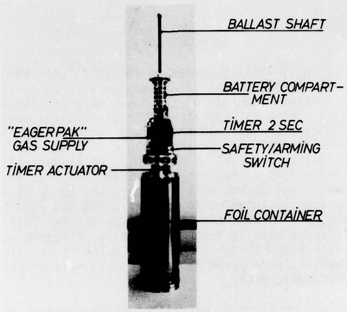
Figure 1. Foil cloud payload used on ARCAS vehicles at WSMR. Lightweight design: foil container is made from 0.2-mm thick aluminum sheet material, reinforced with profile stringers glued to the outside with epoxy resin. Holes were drilled into structure wherever possible to lighten structure. Weight 1.9 kg.
