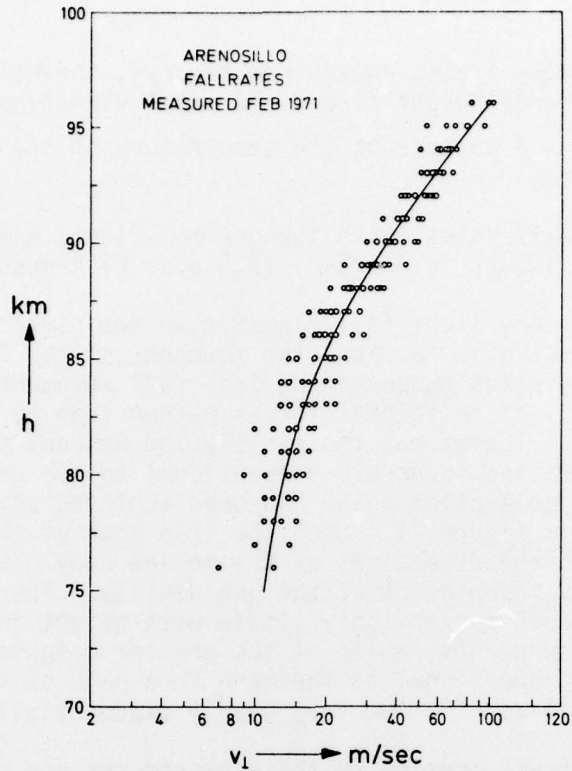
Figure 7. Compilation of measured fall rates done at noontime over El Arenosillo (Feb 71, 13 experiments).
