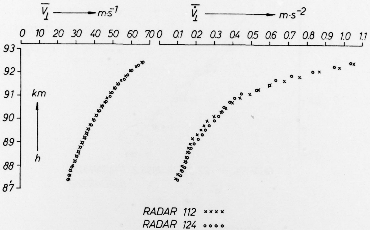
Figure 16. Descend speed and vertical deceleration of foil cloud measured with two independent radars (circles and crosses) (22 Apr 74, 19:06 Z.).
