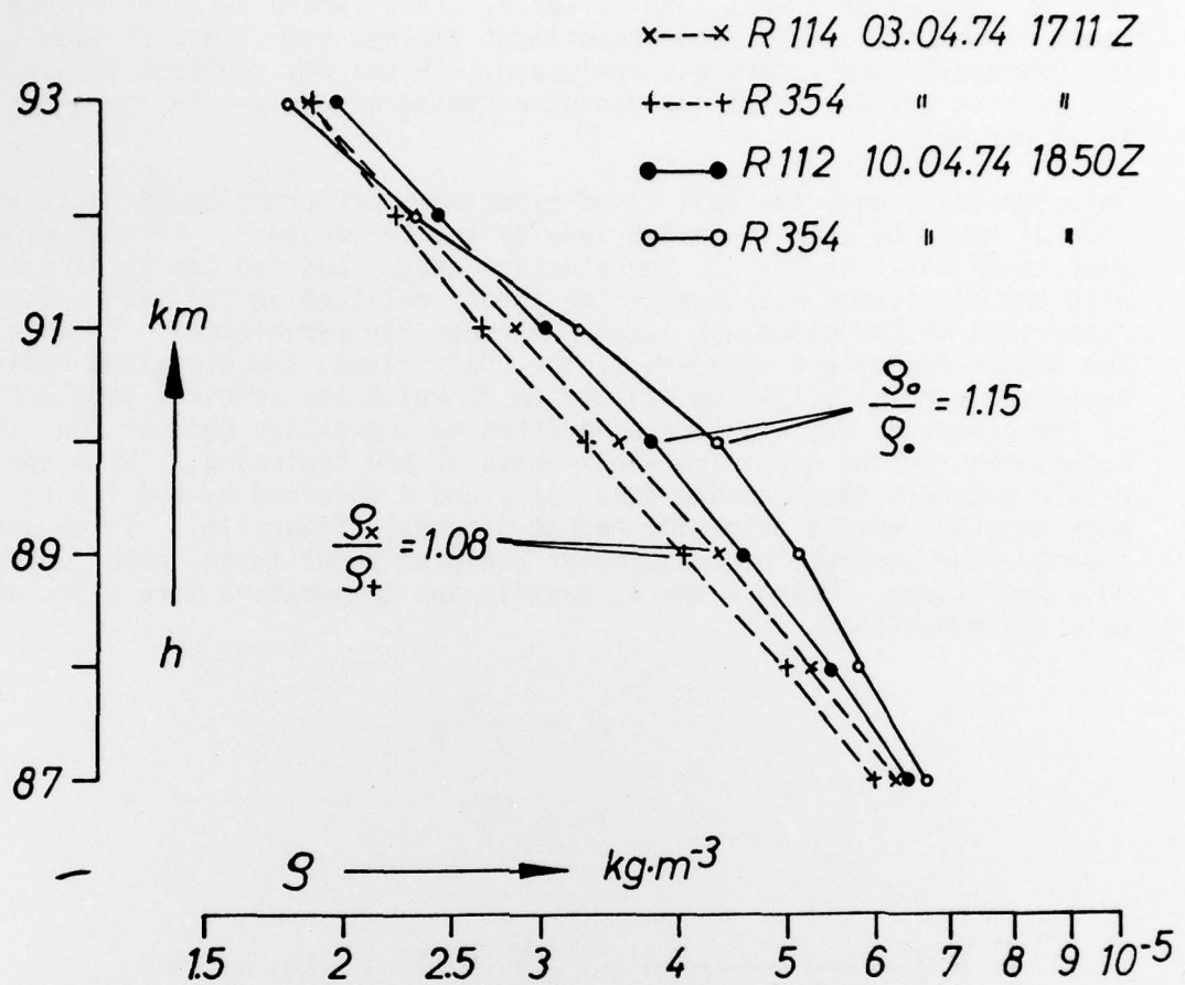
Figure 15. Results of air density measurements made with falling spheres over White Sands.
