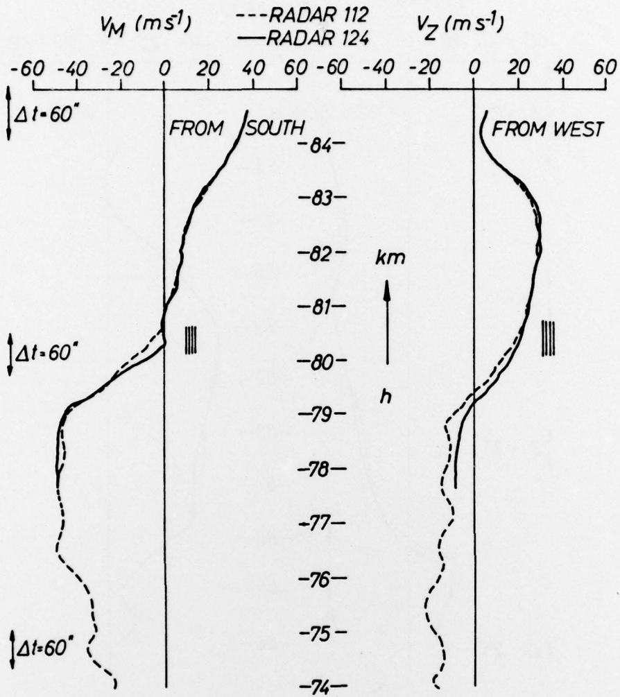
Figure 13. Wind measurement made over White Sands with foil cloud experiment (running means over 60 s. At 80.5 km probably zone of strong turbulence).
