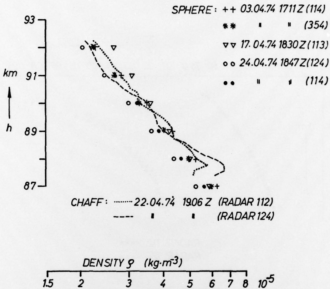
Figure 17. Comparison between density measurements done with spheres (points) and foil clouds (curves). Tracking performed simultaneously with two independent radars in all cases.
