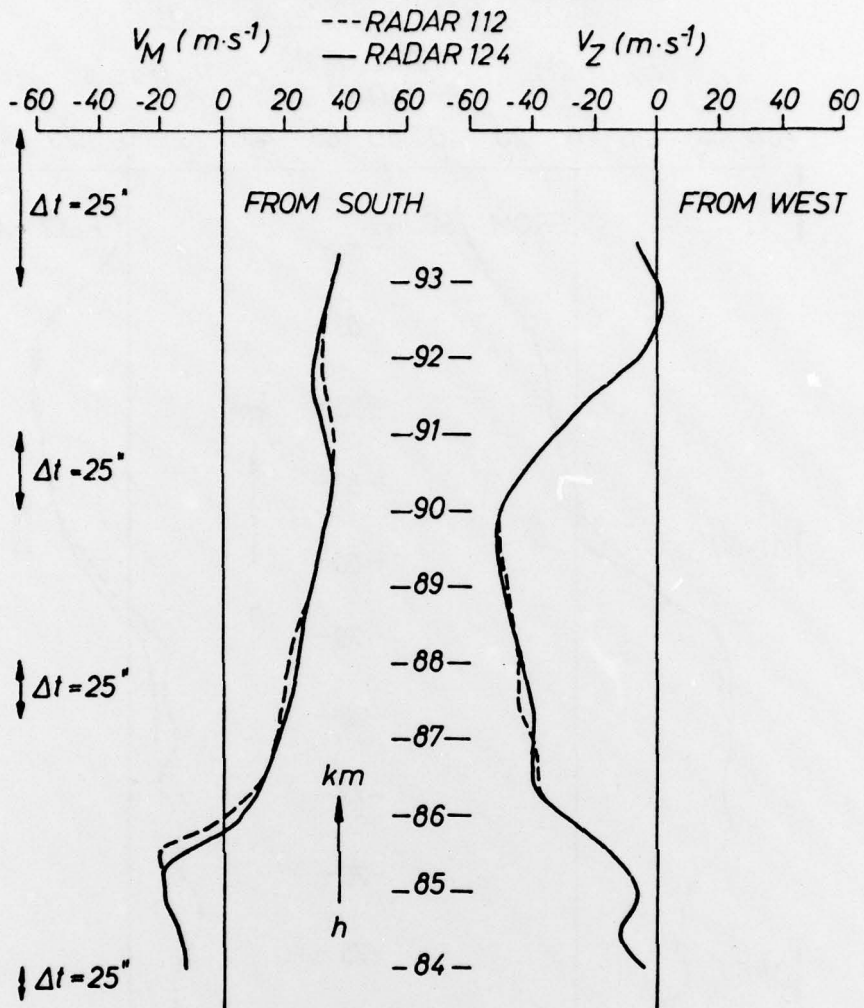
Figure 14. Wind measurement made over White Sands with foil cloud experiment (running means over 25 s tracking time). Cloud was ejected too high.
