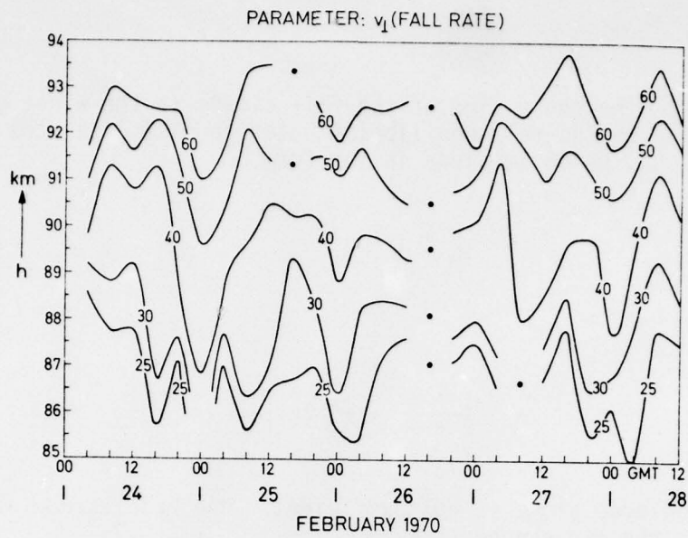
Figure 3. Variation of fall rate as a function of daytime observed on 4 consecutive days. Launches performed every fourth hour (00.00, 04.00, 08.00, 12.00, etc.) El Arenosillo, Spain.
