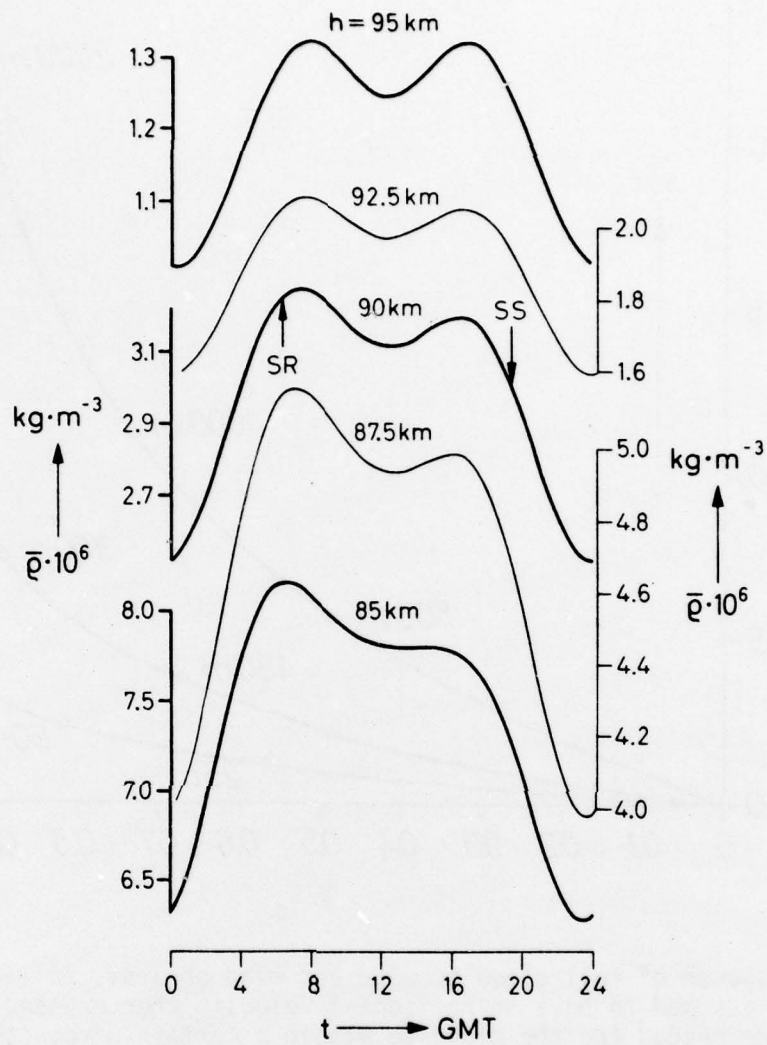
Figure 6. Fourier synthesis of diurnal variation of air density over E1 Arenosillo, derived from measurements on 4 consecutive days (launch every fourth hour, starting with 00.00 GMT).
