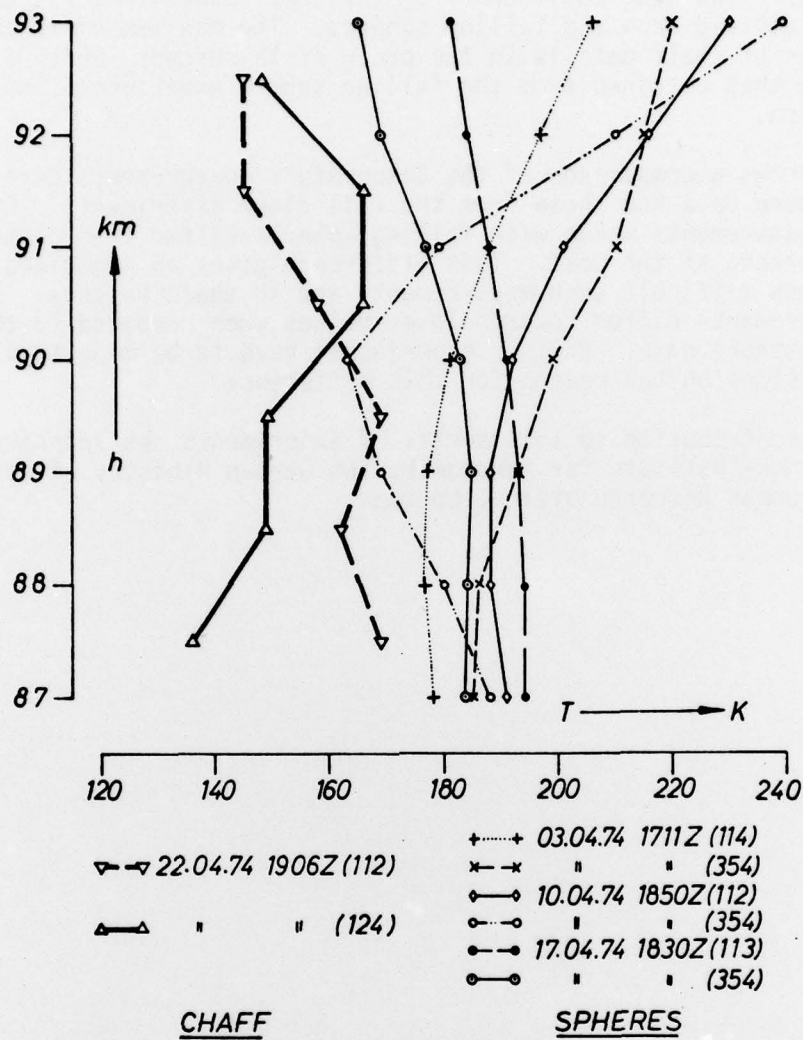
Figure 18. Comparison between temperature analysis of foil cloud and falling sphere data.
