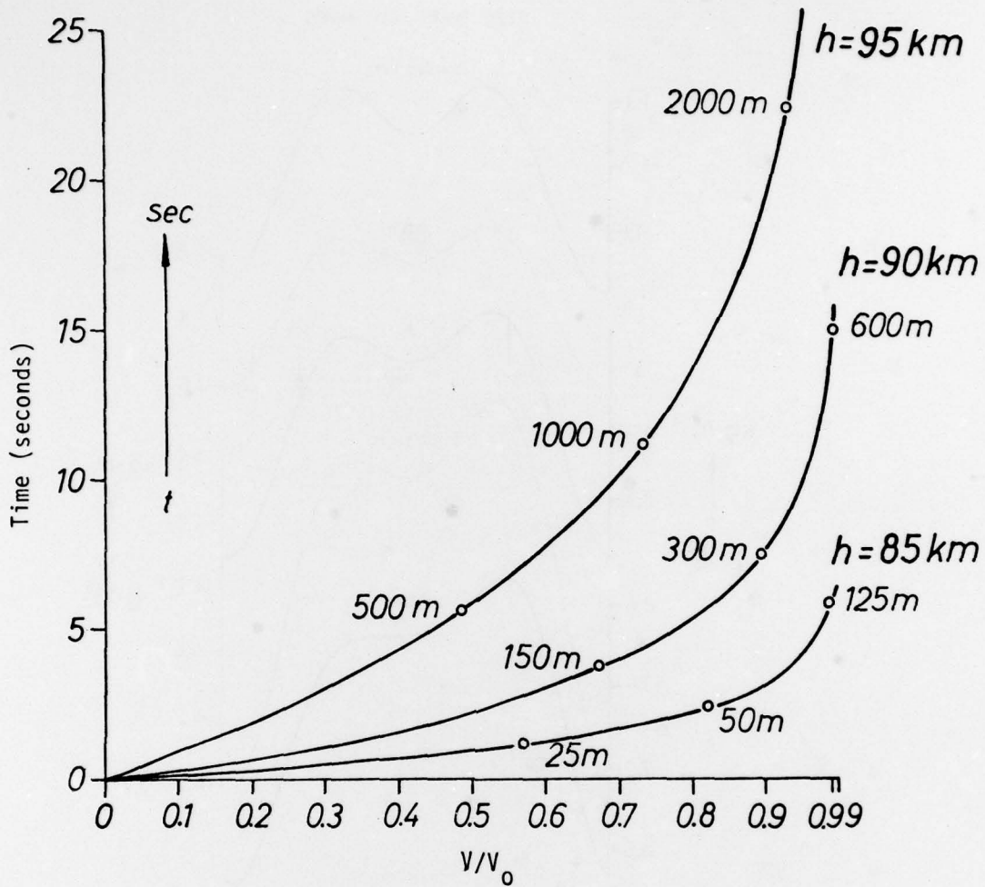
Figure 5. Response of foil cloud to wind and wind shears: falling cloud is assumed to have no horizontal velocity when exposed to wind. Time needed for the cloud to attain a certain percentage of actual windspeed present is shown for three different heights (85, 90, and 95 km), together with the heights traveled in the different height levels.
