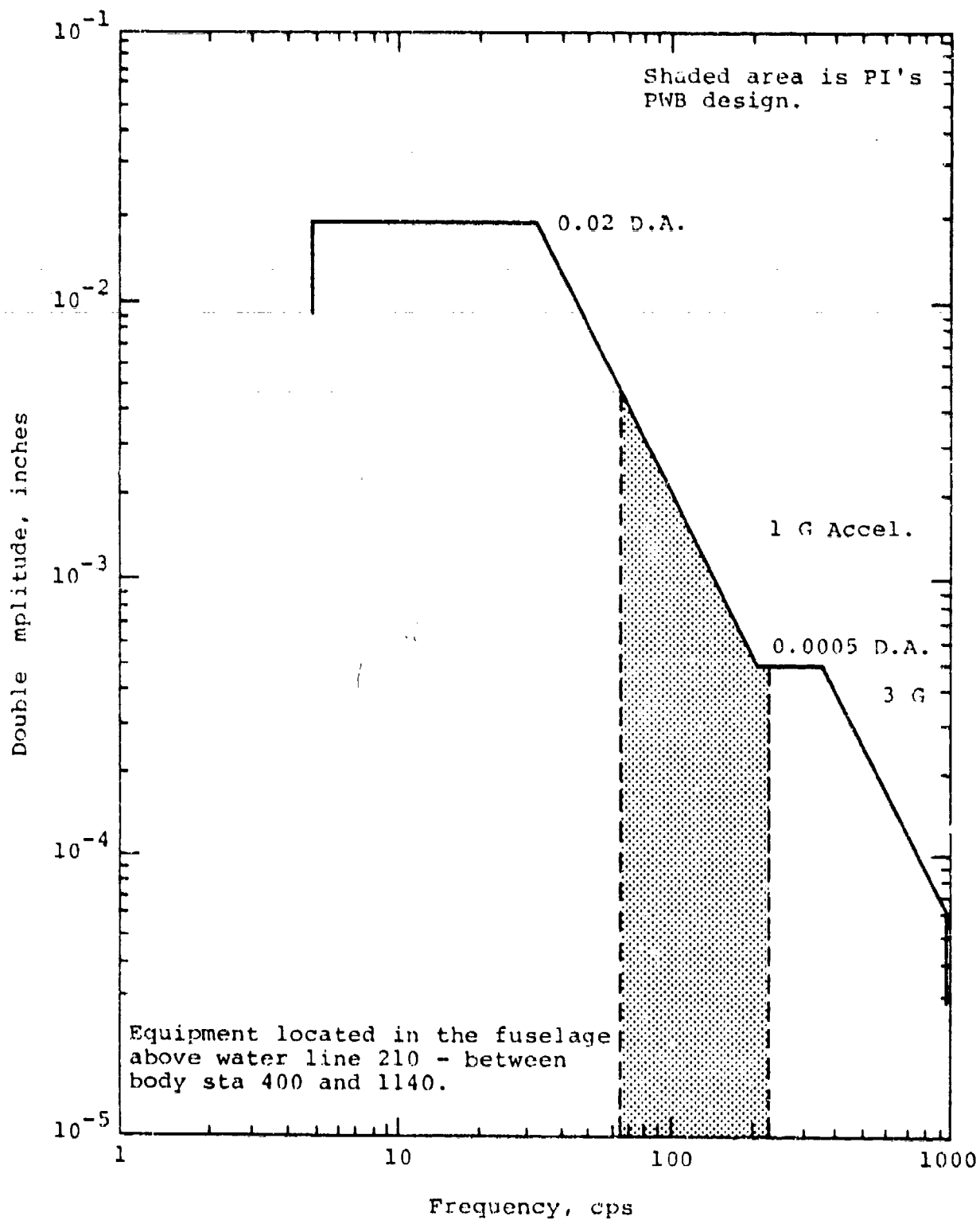
Figure B-2. Vibrational input system.
