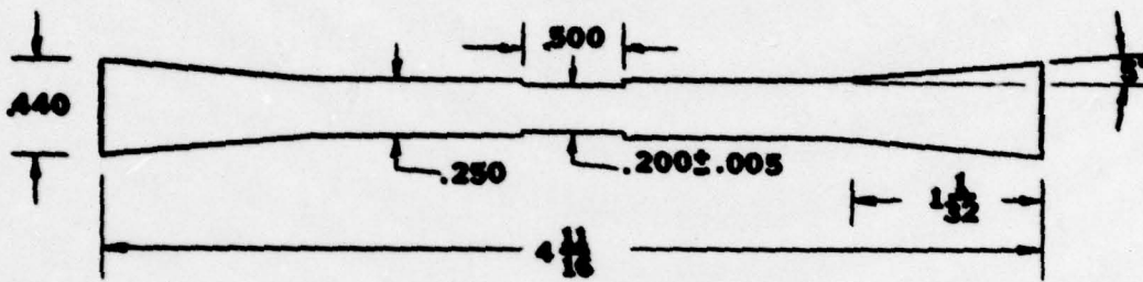
A. Specimen Design
