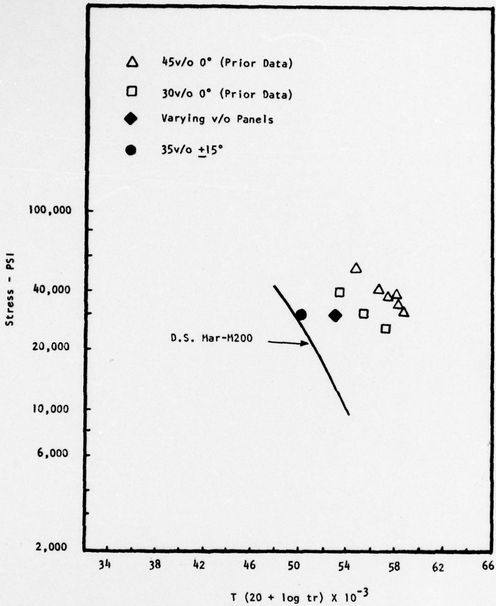
Figure 11. Larson-Miller Parameters for Varying Volume and Angle-Plied Panels.
