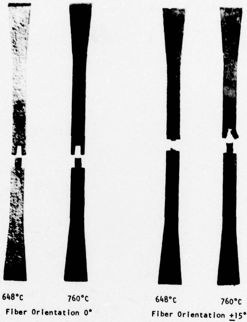
Figure 12. Fracture Mode in W-1ThO 2 /FeCrAlY Double Notch Shear Specimen with Different Fiber Orientations.
