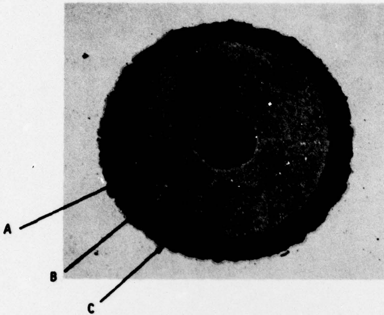
Figure 15. Hafnium Carbide-Coated SiC in FeCrAlY 400X
