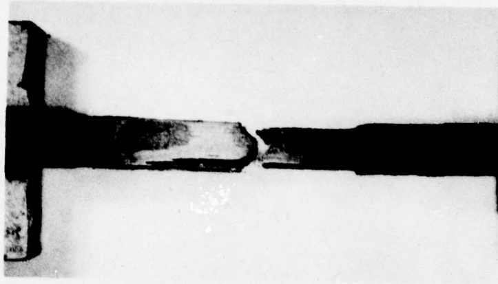
A. Grip and Gage Section at 1800F, Failed at Shoulder
