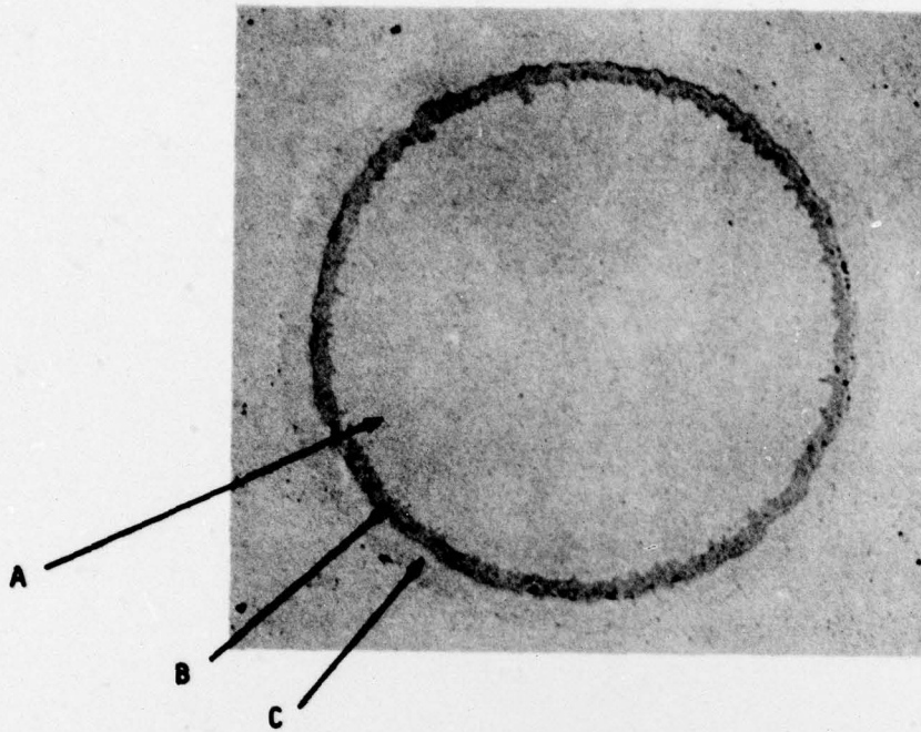
Figure 16. Hafnium Carbide (Over Tantalum Carbide)-Coated W in FeCrAlY. 400X
