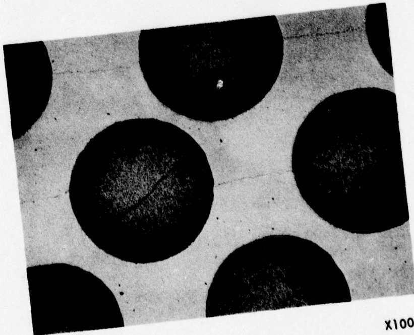
Figure 2. Initial Trials on W/MA 956E Composite. The top photomicrograph shows lack of consolidation and the bottom poor matrix-matrix bonding; both show fiber damage.
