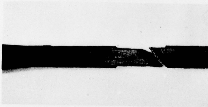
B. Grip at ~1100F, Gage at 1800F; Failed in Gage Section (Second Failure During Disassembly)
