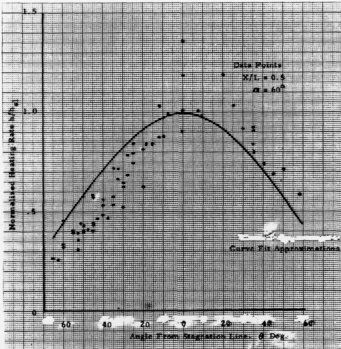
Figure 5 Cylinder Off-Stagnation Line Heating Rate Normalized by Stagnation Line Heating Rate
