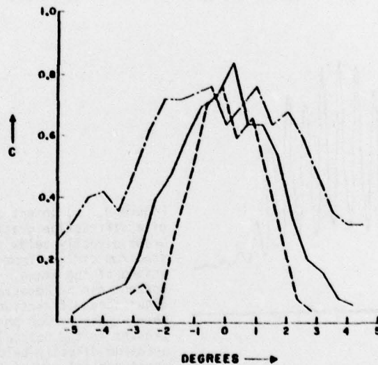
Figure 8. Correlation magnitude of first harmonic vs. angular misalignment in detection plane for three amplitude gratings. In each case the grating is oriented vertically in the transmitter aperture. Zero degrees orientation indicates a scan in the detection plane horizontally. Since the spatial extent of the first harmonic is essentially the same for all the gratings, the sensitivity to angular alignment of the detection plane is proportional to the distance of the harmonic from the origin. Hence detections with the highest frequency gratings are most sensitive to angular alignment. ···· shows data from 39 lines/cm grating, — from 78 lines/cm grating, and - - - from 118 lines/cm grating.
