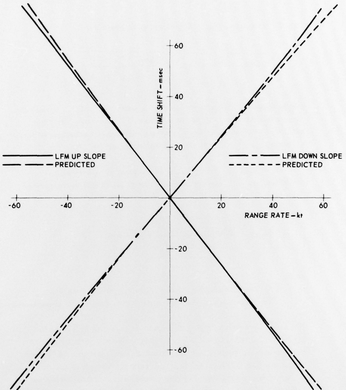
FIGURE 13 TIME SHIFT OF MAXIMUM CORRELATION AS A FUNCTION OF RANGE RATE T = 160 \text{ msec} W = 440 f_0 = 5000 \text{ Hz}
