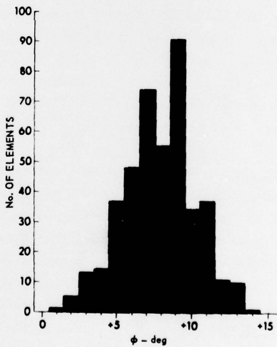
FIGURE 2 HISTOGRAMS OF Z AND \phi OF BARE TRANSDUCER AT 5.0 kHz
