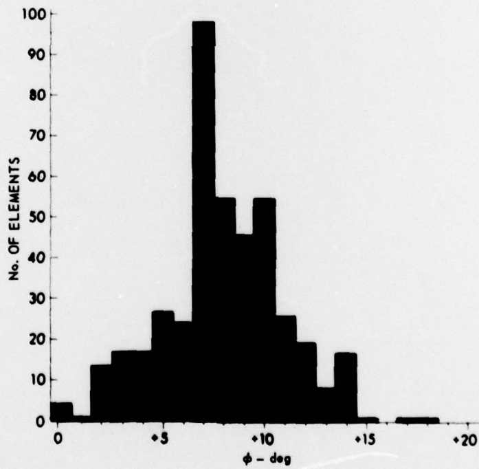
FIGURE 4 HISTOGRAMS OF Z AND \phi OF TRANSDUCER AT 5.0 kHz ABOARD USS VOGELGESANG
