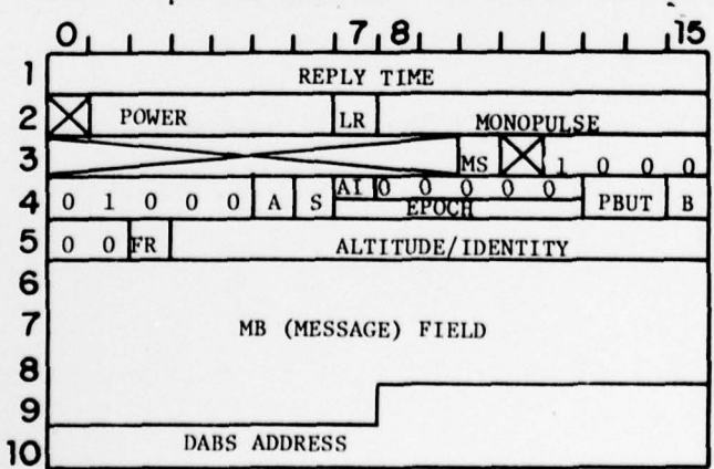
COMM-B REPLY (112 BITS)
