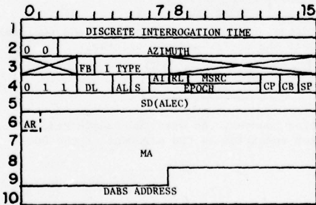
COMM-A INTERROGATION (112 BITS)
