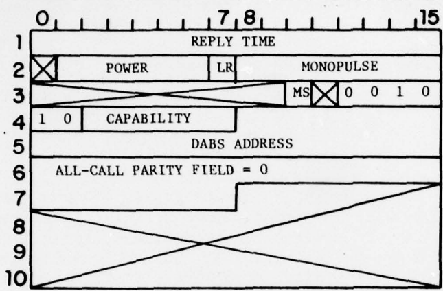
ALL-CALL REPLY (56 BITS)
