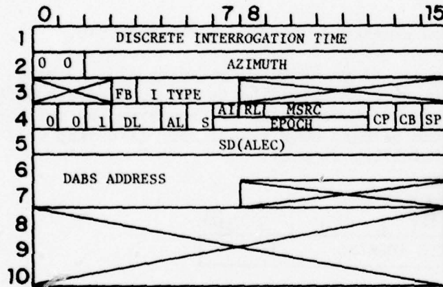
SURVEILLANCE INTERROGATION (56 BITS)
