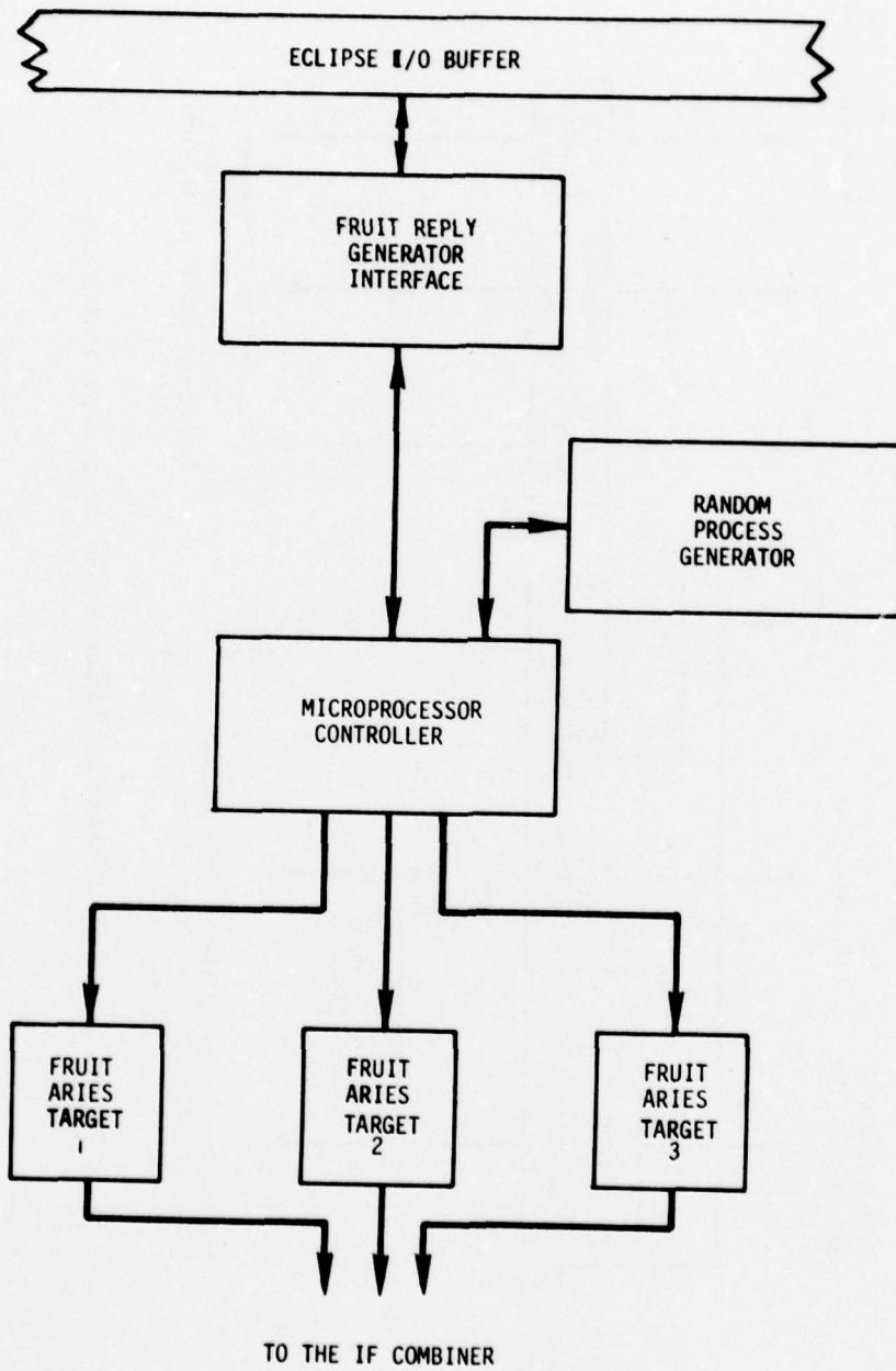
Fig.4.1. Fruit Reply Generator Components.
