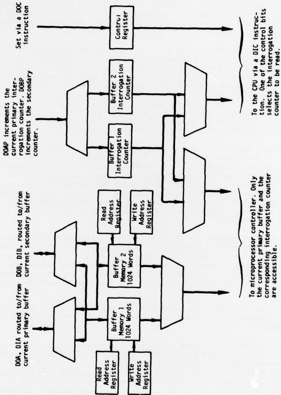
Fig. 3.2. Block Diagram of the CRG Interface.
