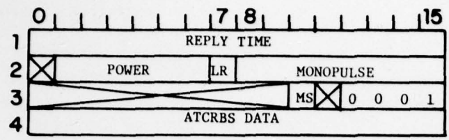
ATCRBS REPLY
