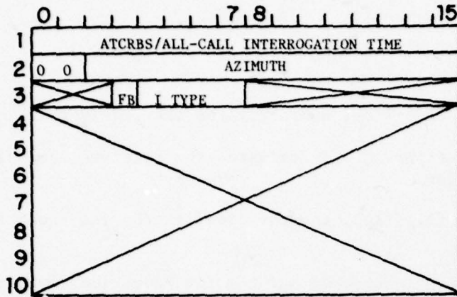
ATCRBS/ALL-CALL INTERROGATION
