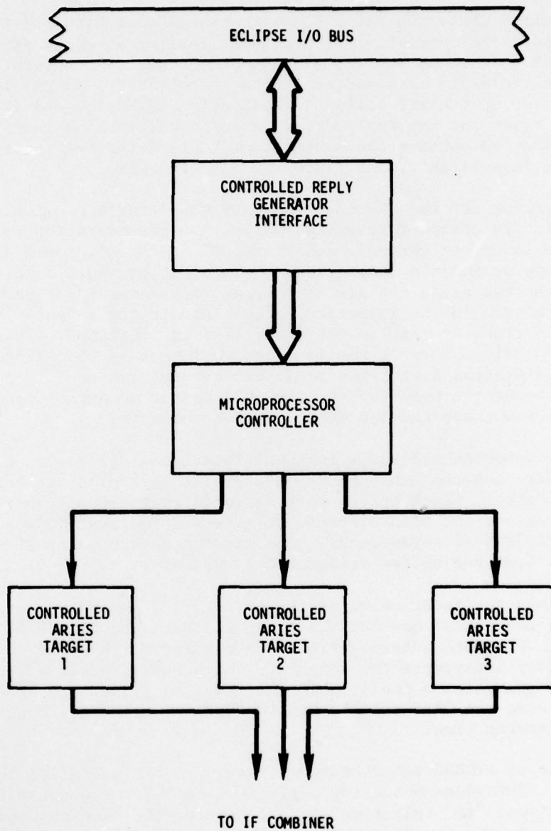
Fig.3.1. Controlled Reply Generator Components.
