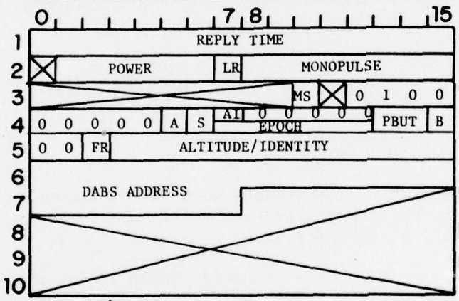
SURVEILLANCE REPLY (56 BITS)
