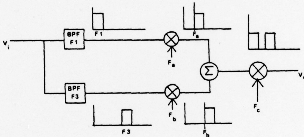
FIGURE 16 SYSTEM CONCEPT
