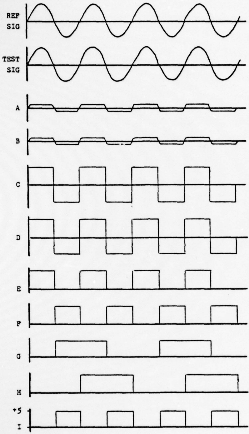
FIGURE 11 - TIMING DIAGRAM FOR PHASE DETECTOR CIRCUIT
