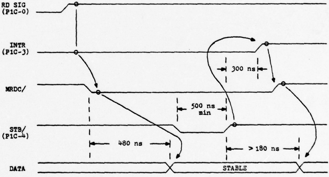
(b) TIMING DIAGRAM FOR 8255
