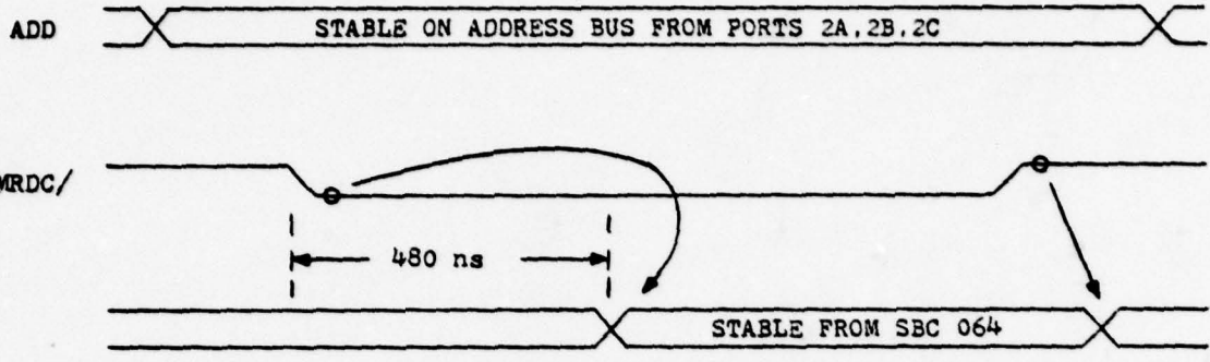
(a) TIMING DIAGRAM FOR SBC 064
