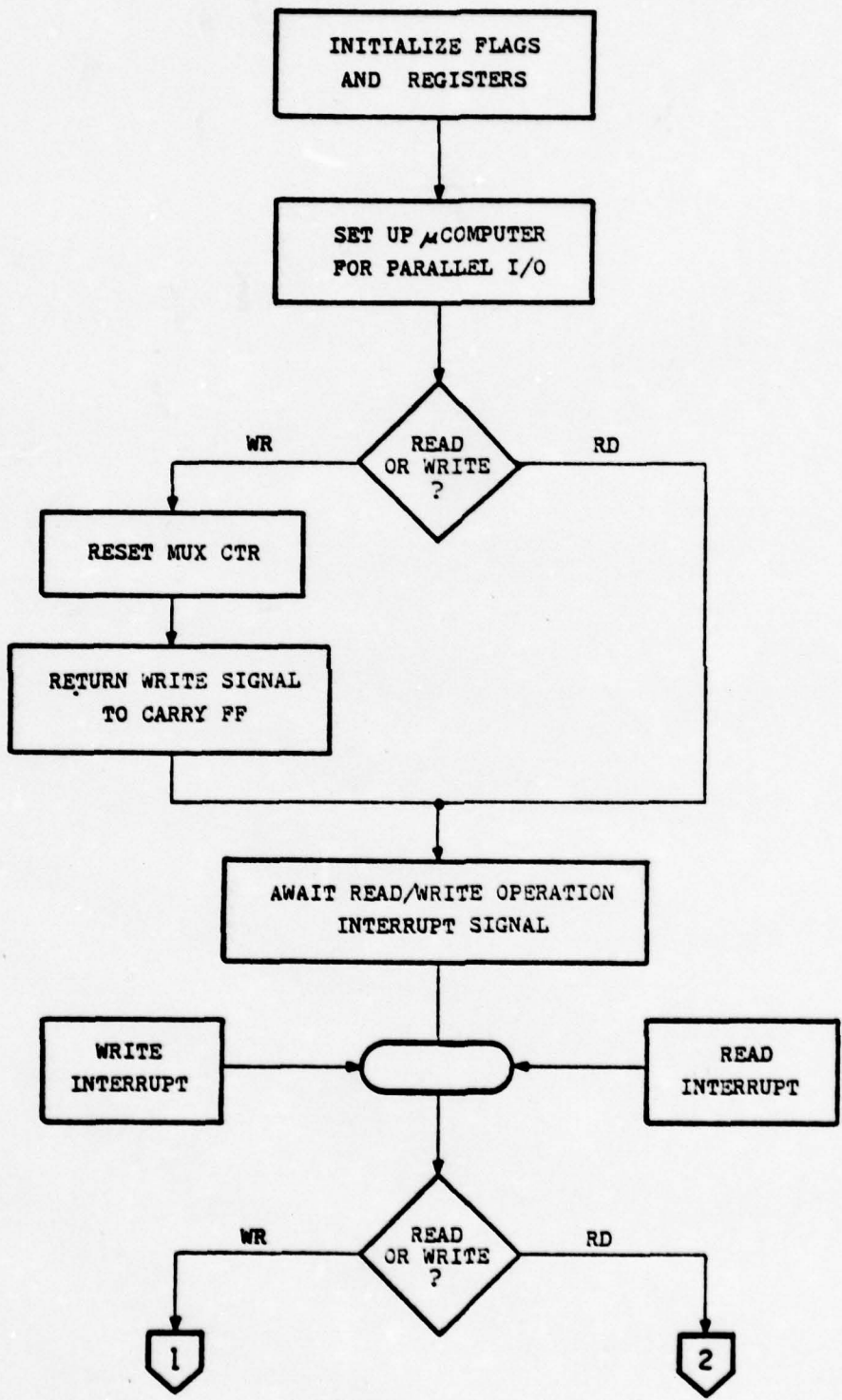
FIGURE 17 - POWER UP SEQUENCE ALGORITHM
