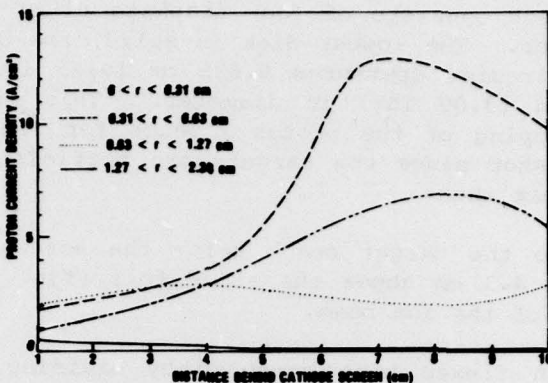
Figure 2. Map of proton flux in focussing triode geometry with input flux normalized to 1 \text{ A/cm}^2 .
