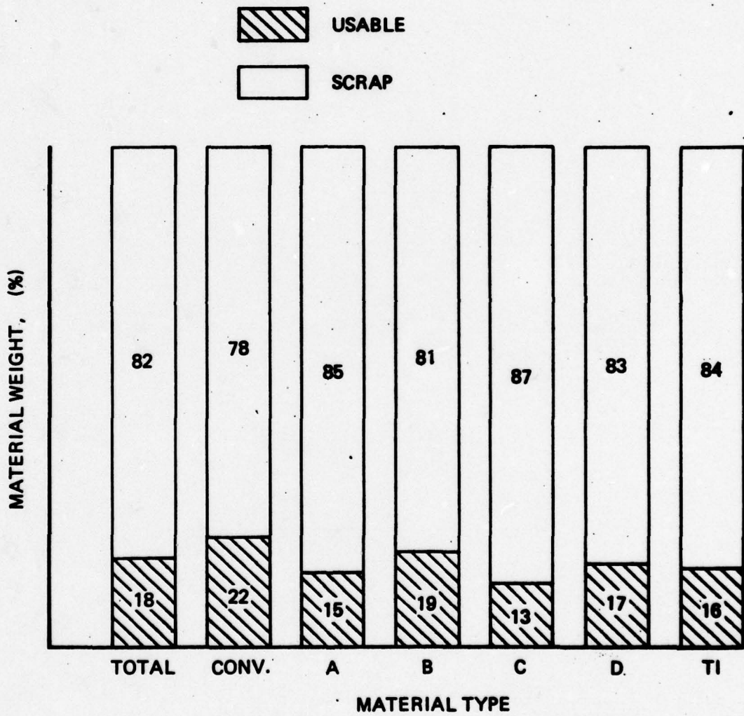
Figure 2-3 Manufacturing Efficiency
