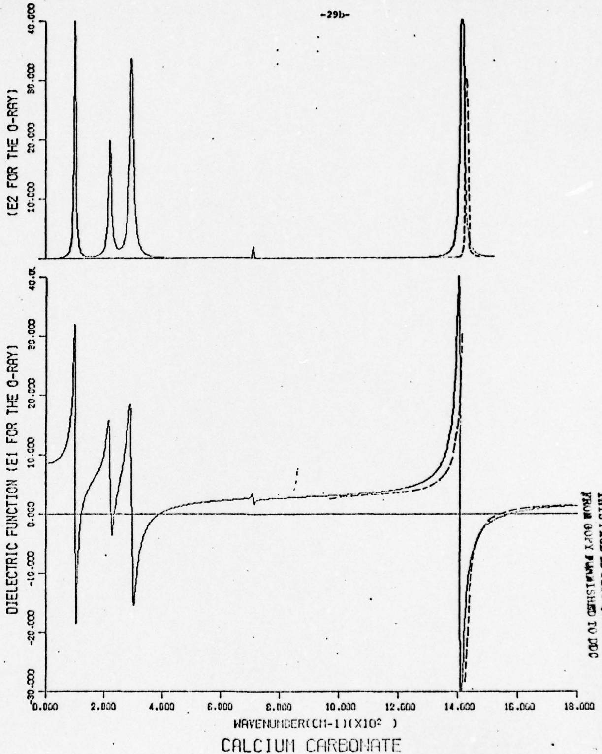
Figure 15: Results for calcium carbonate of the inversion of powder extinction data to infer dielectric functions (dashed curve) compared with dielectric functions derived from single crystal measurements (solid curve from the reference in Table 11).
