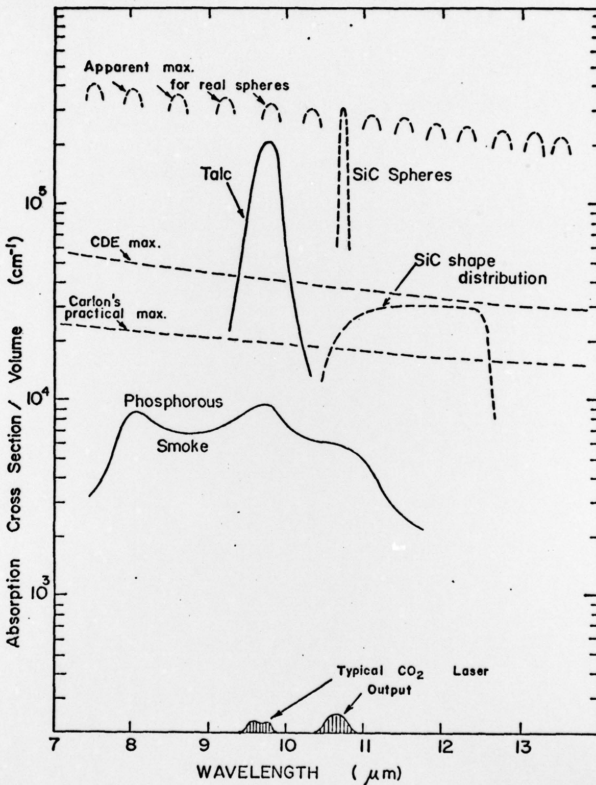
Figure 20: Volume-normalized extinction for a collection of several highly absorbing materials and for several practical limits discussed in the text.
