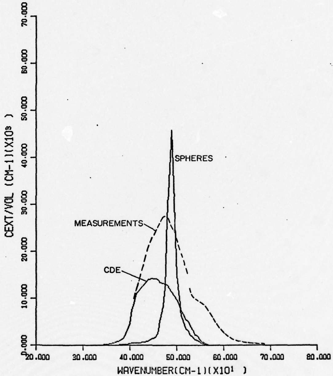
Figure 13: Comparison of measured extinction (dashed curve) for NiO powder in KBr with calculations for spheres and for a distribution of ellipsoidal shapes (CDE) in the Rayleigh approximation.
