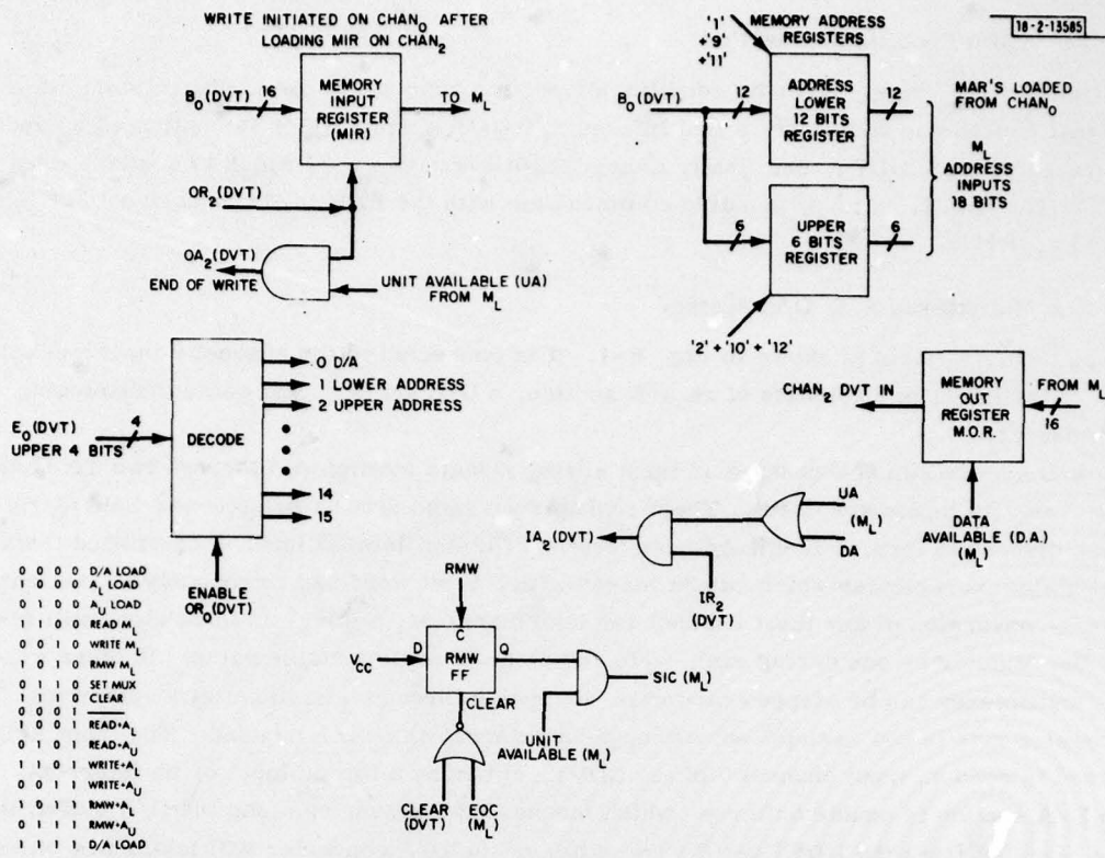
Fig. E-5. Large memory interface (M L ) channel 0 decoder.
