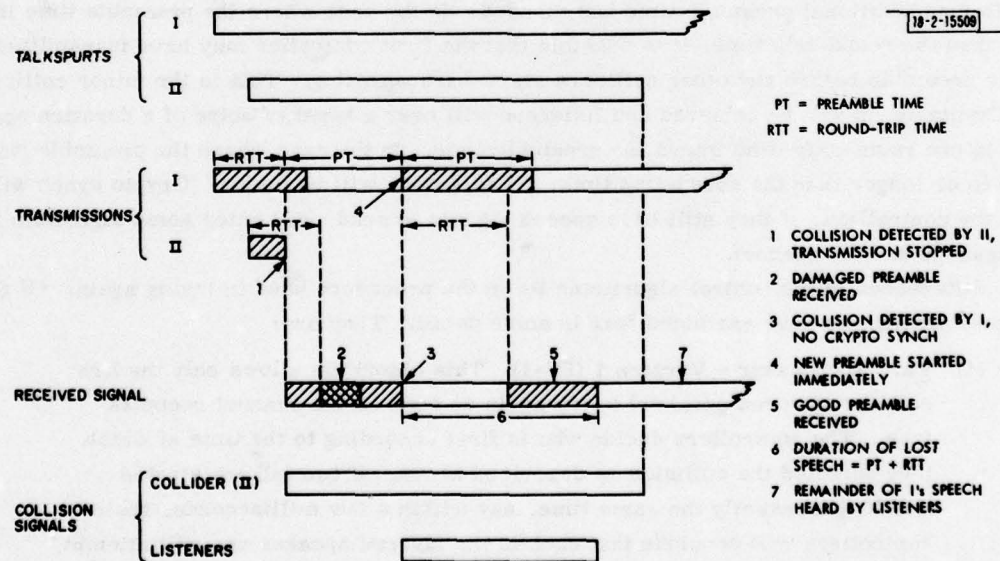
Fig. 2-4. SCDC collision-handling algorithm FS-2. Favored speaker (I) proceeds immediately.
