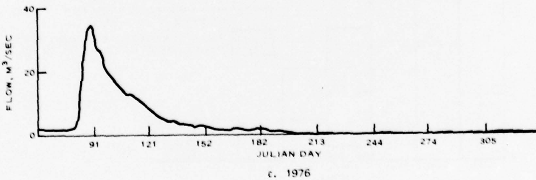
Figure 24. Mean daily discharge at Twin Valley
