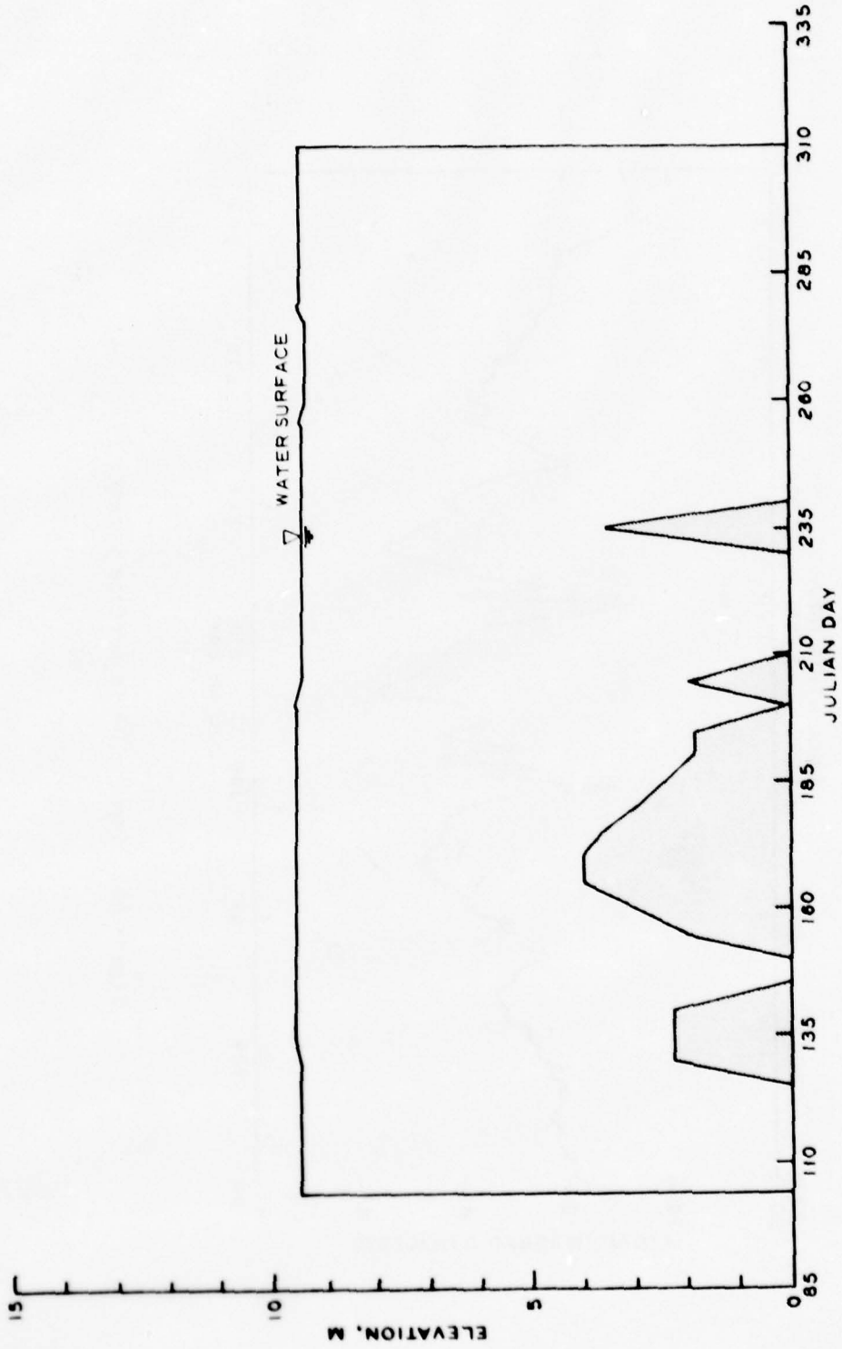
Figure 41. Zone of anoxia (DO < 2 mg/l), 1971
