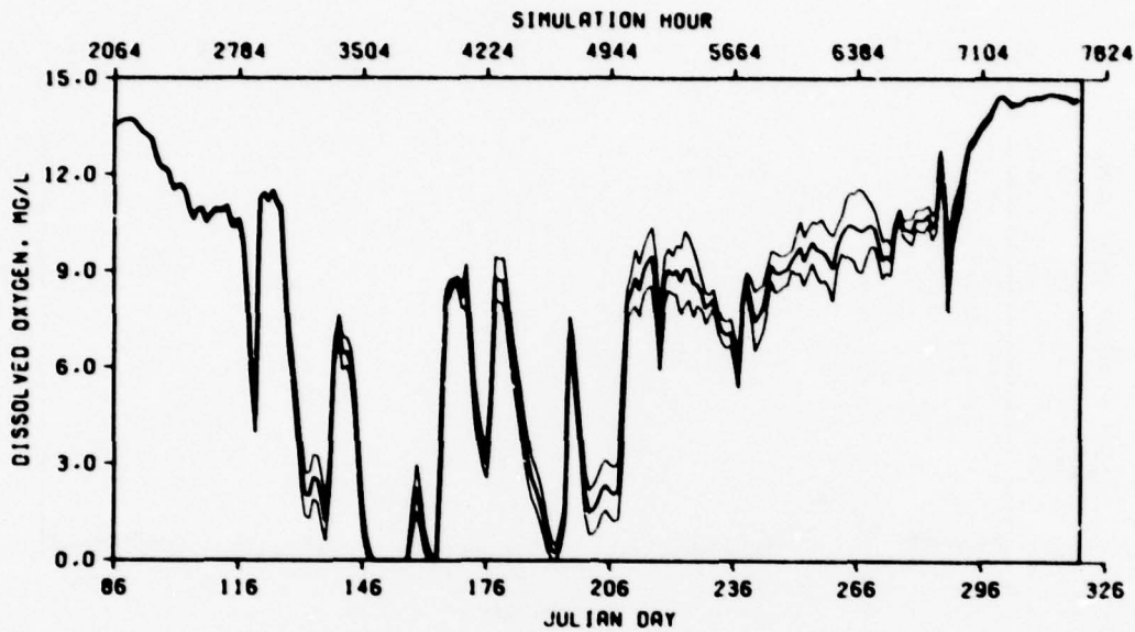
Figure 100. Mean and 95 percent confidence interval of DO in the bottom metre with a minimum of release of 0.42 \text{ m}^3/\text{sec} , 1976
