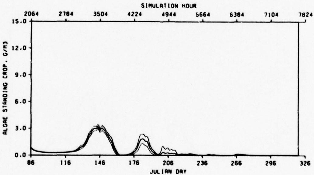
Figure 101. Mean and 95 percent confidence interval of ALGAE 1 in the euphotic zone with a minimum of release of 0.42 \text{ m}^3/\text{sec} , 1976
