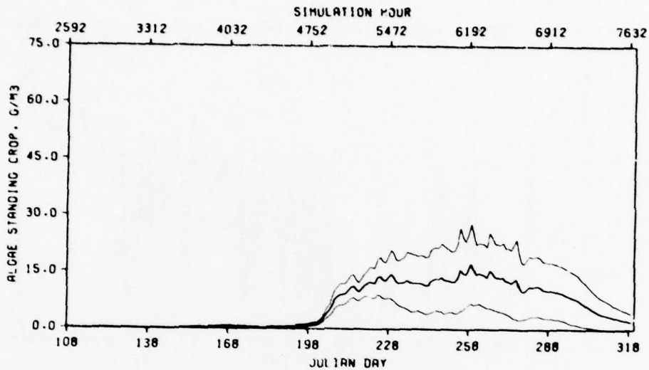
Figure 108. Mean and 95 percent confidence interval of ALGAE 2 in the euphotic zone with a maximum release of 48 m 3 /sec, selective withdrawal, 1975
