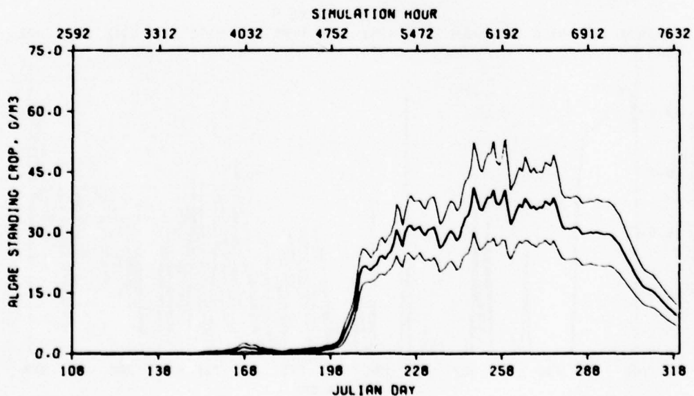
Figure 105. Mean and 95 percent confidence interval of ALGAE 2 in the euphotic zone with a maximum release of 48 m 3 /sec, 1975
