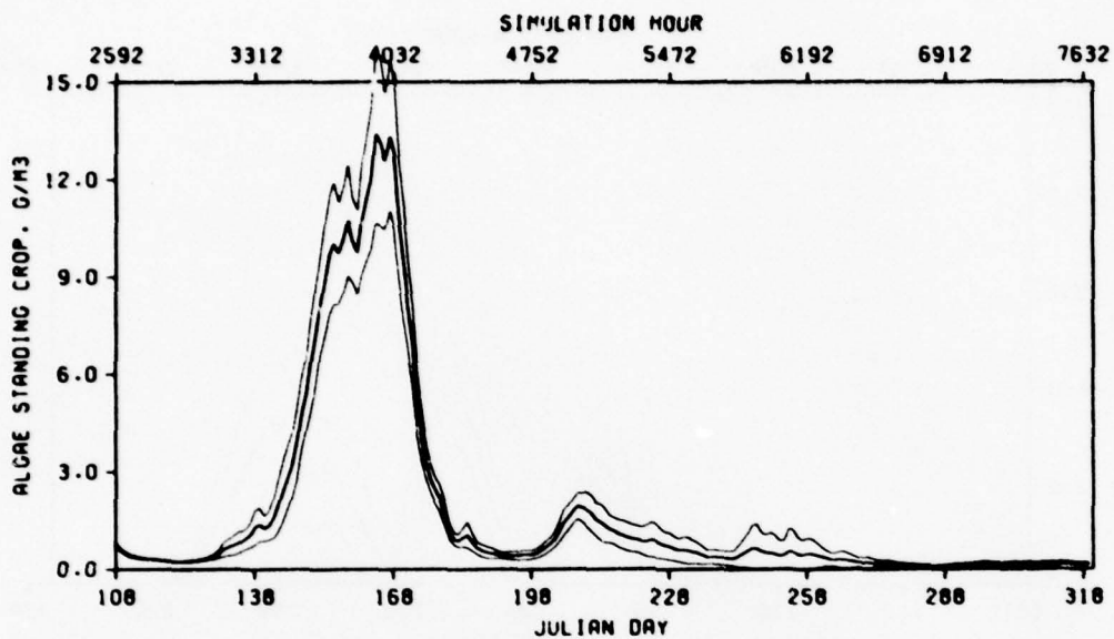
Figure 104. Mean and 95 percent confidence interval of ALGAE 1 in the euphotic zone with a maximum release of 48 m 3 /sec, 1975
