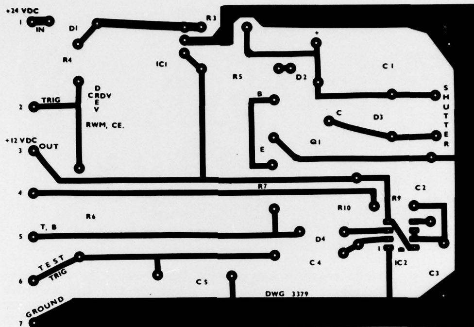
FIGURE 5 - Circuit board foil pattern. Scale is full size.
