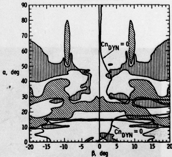
Figure 3-8.- Stability plot and sideslip trim for aileron deflection of 10°.
