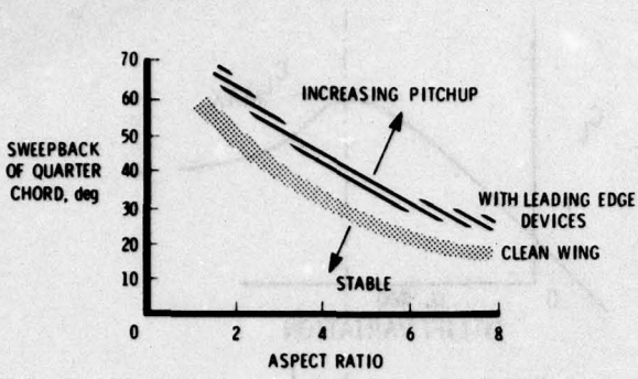
Figure 2-6.- Wing pitchup boundaries.
