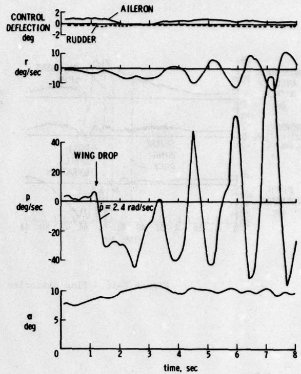
Figure 2-13.- Wing drop and wing rock. M = 0.77
