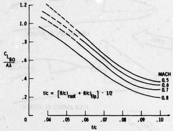
Figure 2-25.- Variation of buffet parameters with thickness ratio for aircraft without maneuver devices.
