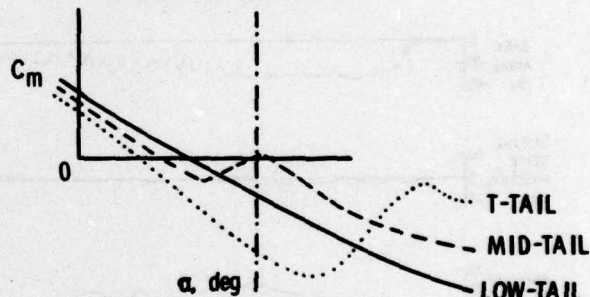
(c) PITCHING-MOMENT VARIATION
