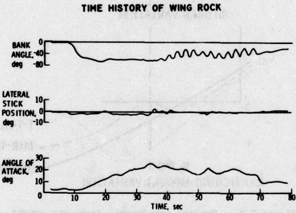
Figure 2-8.- Flight record of fighter encountering wing rock.
