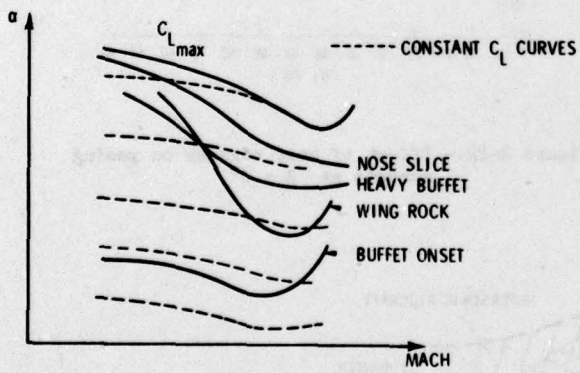
Figure 3-1.- Typical engineering maneuver boundaries
