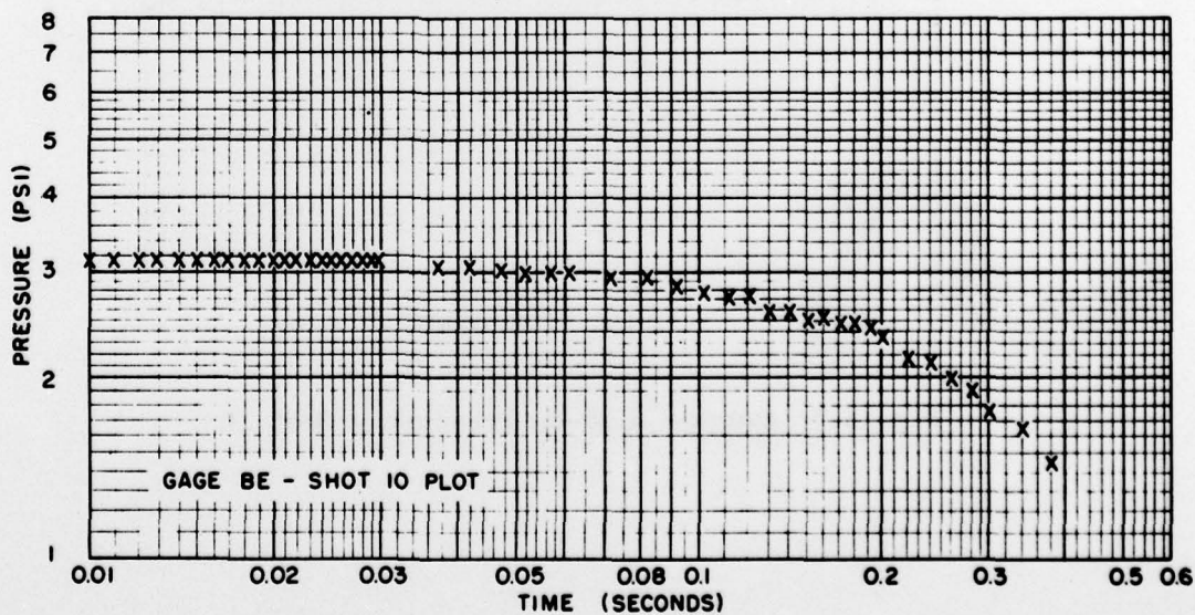
Fig. 5.6 Fitting Free-Field Records to Idealized Curve-Shot 10
