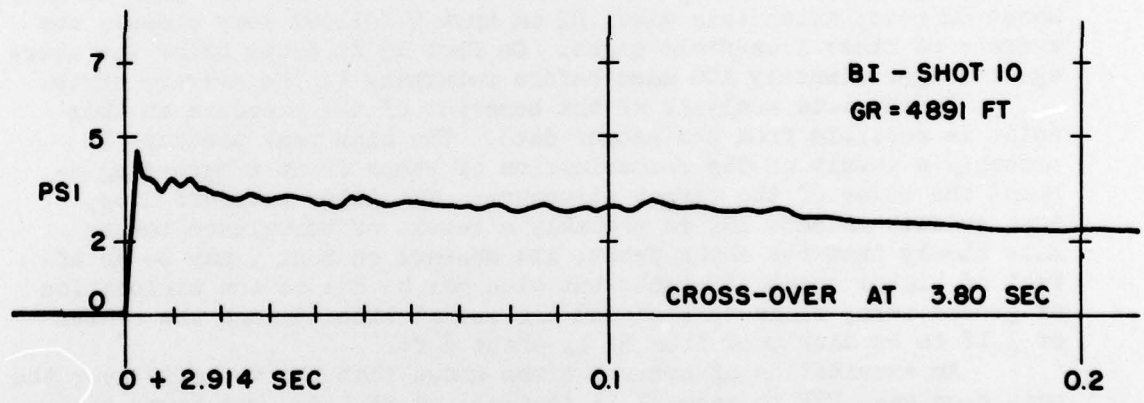
Fig. 5.8 Gage BI Records - Shots 9 and 10
