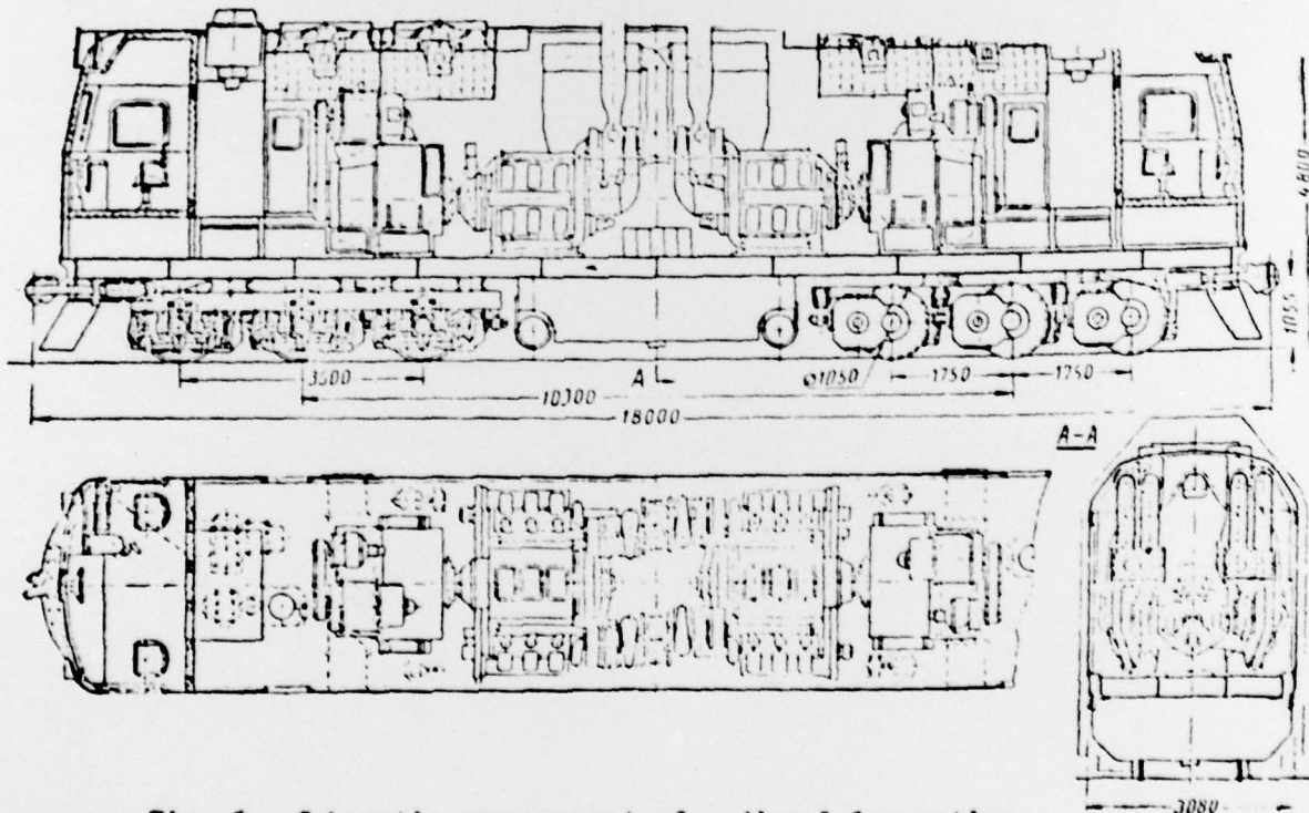
Fig. 8. Schematic arrangement of a diesel locomotive, 6000 hp in a section using X-shaped D49 engines
