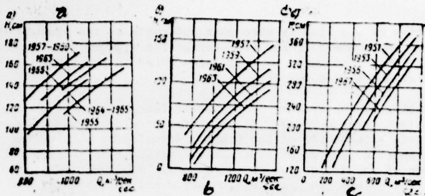
Figure 6. Annual variation of Q = f(H) curves for the reaches below Gor'kov (a), Novosibirsk (b), and Tsimlyansk (c) dams.
