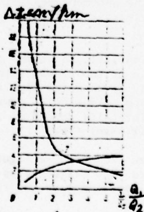
Figure 11. Graph of the relationship Z = f(Q_1/Q_2) based on observations on the Don (1) and Severskiy Donets (2) sectors above their confluence.
