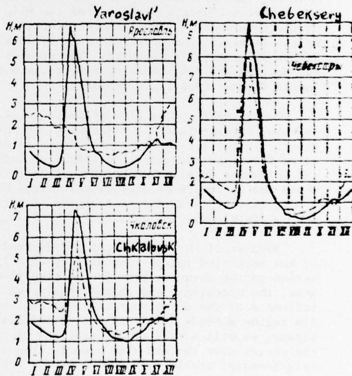
Figure 5. Graphs of mean water level on different hydraulic sections of the Volga below Rybinsk HES (dashed line 1916-1940; solid line - 1941-1953).
