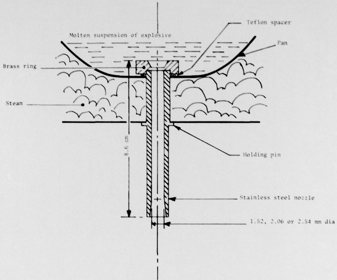
FIGURE 3 - Nozzle assembly
