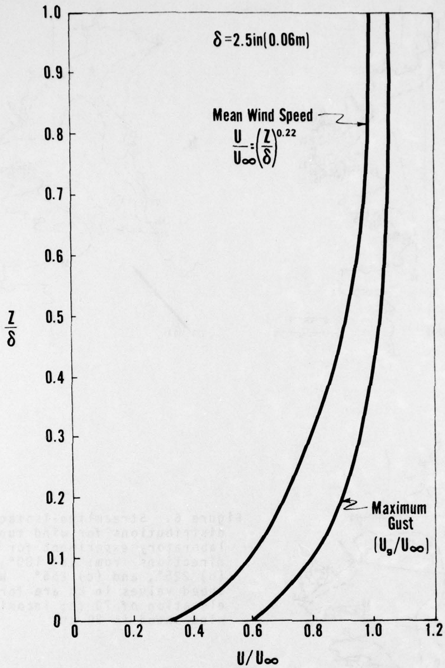
Figure 5. Mean wind speed and maximum gust profiles of the approach flow. U is the mean wind speed at level z , U_\infty is the mean wind speed at the top of the boundary layer at height \delta , and U_g is the maximum gust wind value.
