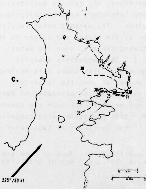
Figure 12. Streamline-isotach distributions in kt and for an elevation of 70 ft for: (a) dynamic model output for Tropical Storm Olga, 0000 GMT 24 May 1976; (b) synoptic composite for data from 225° (range from 218° to 232° based on 41 observations and analyzed only where data were available and (c) comparable laboratory analysis from Figure 6b.
