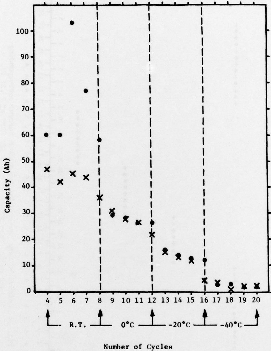
Fig. 4: Variation of capacity with cycles (LVC of 14.25 V). ● Charge accepted during 2 hrs charging (14.25 V, 20 A). x Capacity of the accumulator at 285/300 A. End of discharge 6 V.
