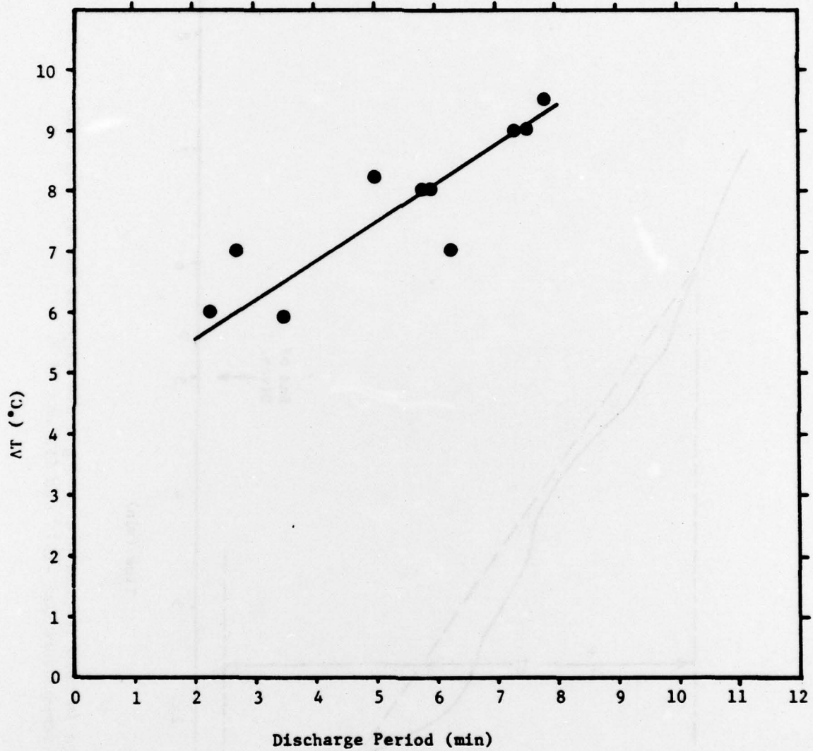
Fig. 8: \Delta T of the acid versus period of discharge at a constant cranking current of 285 A (LVC = 16 V).
