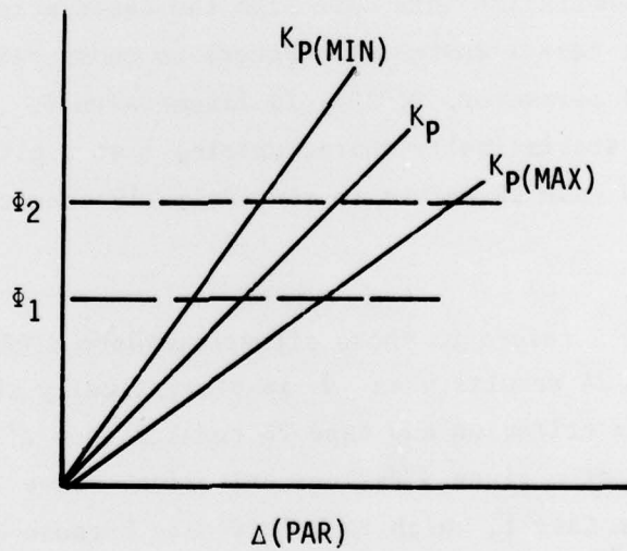
Figure F-1. Illustration of case 2 where the change in the electrical parameter \Delta(\text{PAR}) is linear with neutron fluence \phi : (a) case 1A, characterizing \phi at two given \Delta(\text{PAR}) failure levels, and (b) case 1B, characterizing \Delta(\text{PAR}) at two given \phi failure levels. K_P is an arbitrary constant of proportionality relating \Delta(\text{PAR}) and \phi .
