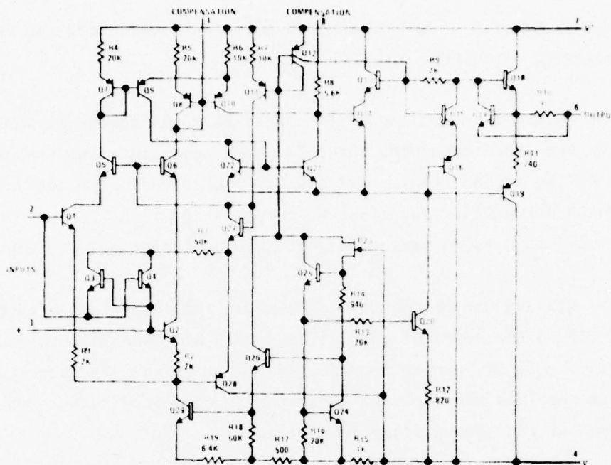
Figure D-3. Type LM108A operational amplifier.
