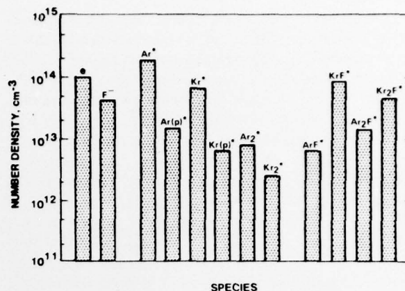
Fig. 8. Particle concentrations corresponding to the conditions of Fig. 7 at a time 0.4 μs after discharge initiation.
