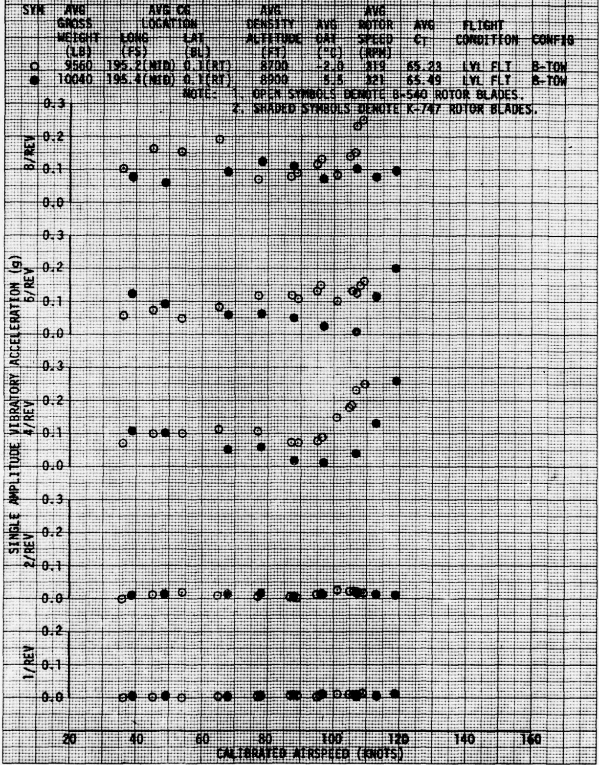
FIGURE 61 VIBRATION CHARACTERISTICS YAN-1R USA S/N 70-15936 PILOT INSTRUMENT PANEL LONGITUDINAL
