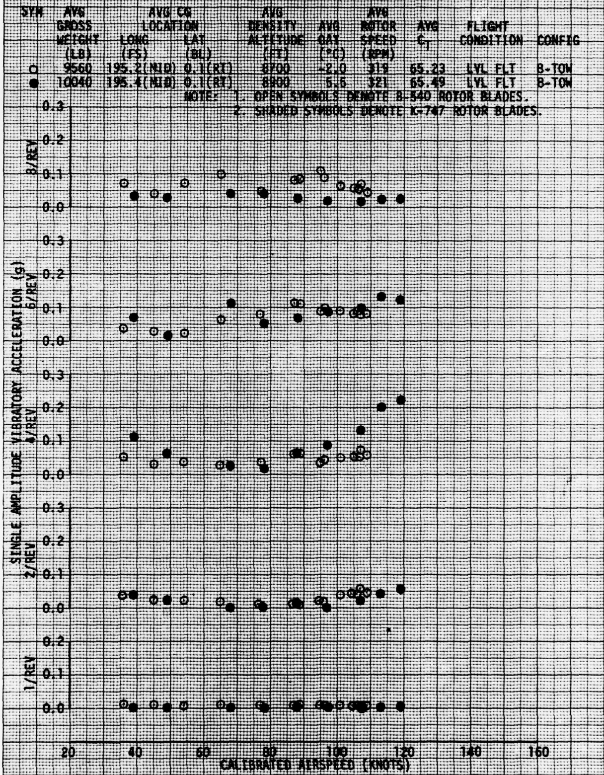
FIGURE 62 VIBRATION CHARACTERISTICS YAN-1B USA S/N 70-15936 PILOT INSTRUMENT PANEL LATERAL
