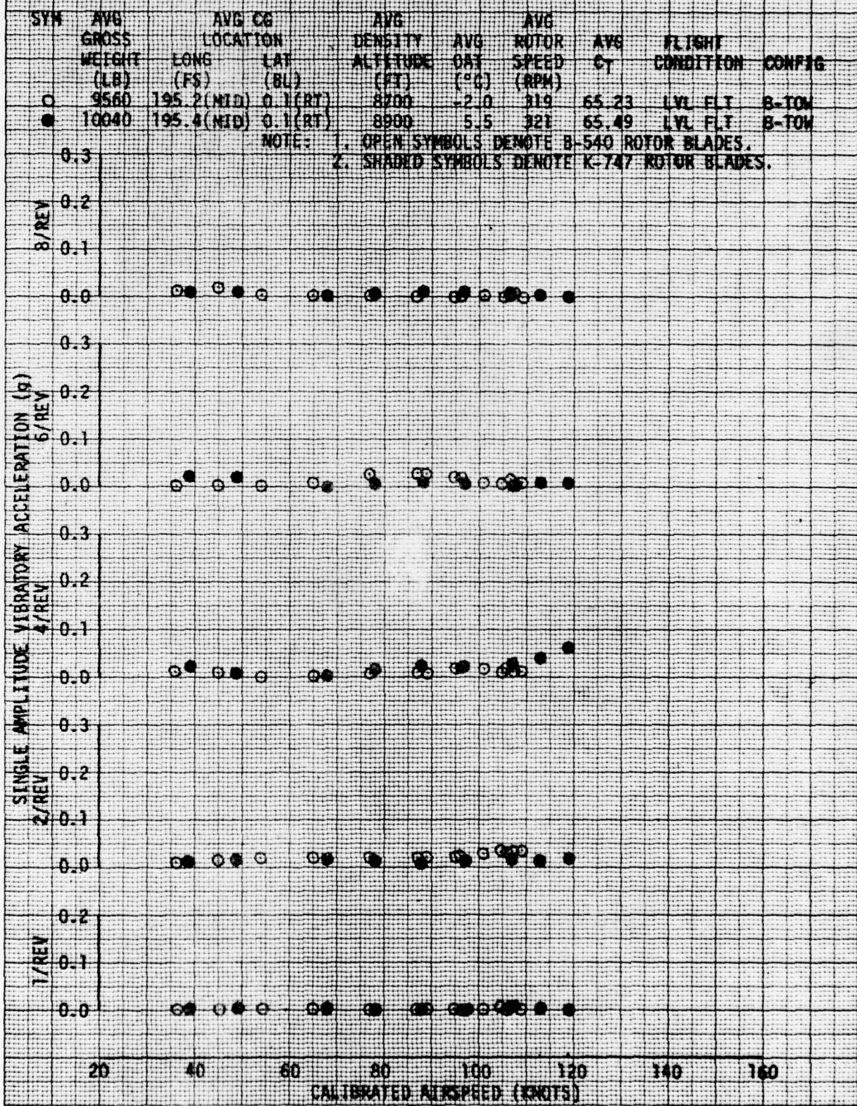
FIGURE 5B VIBRATION CHARACTERISTICS YAM-TR USA S/N 70-15936 COPILOT SEAT LONGITUDINAL
