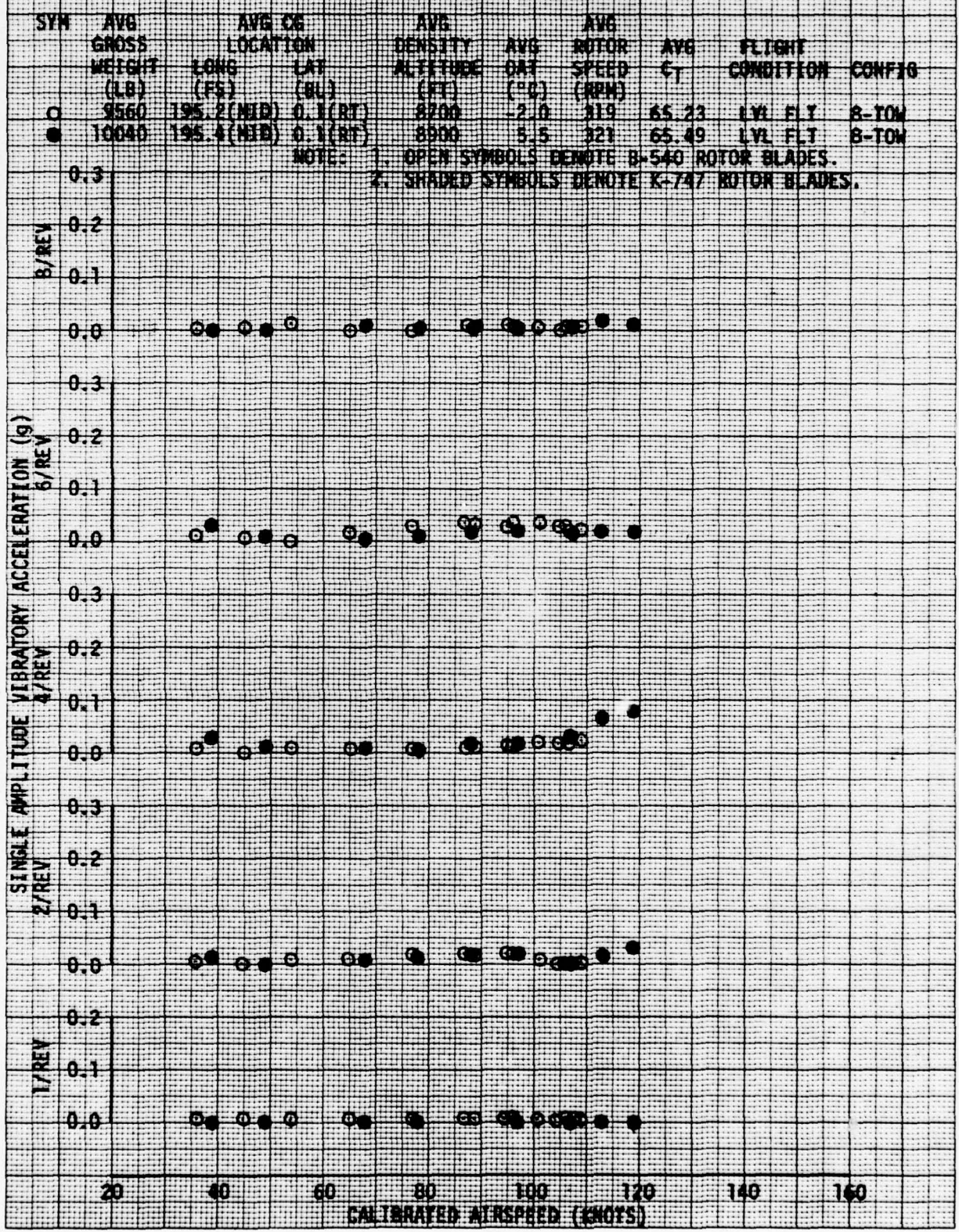
FIGURE 59 VIBRATION CHARACTERISTICS YAN-TR USA S/N 79-15936 COPILOT SEAT LATERAL
