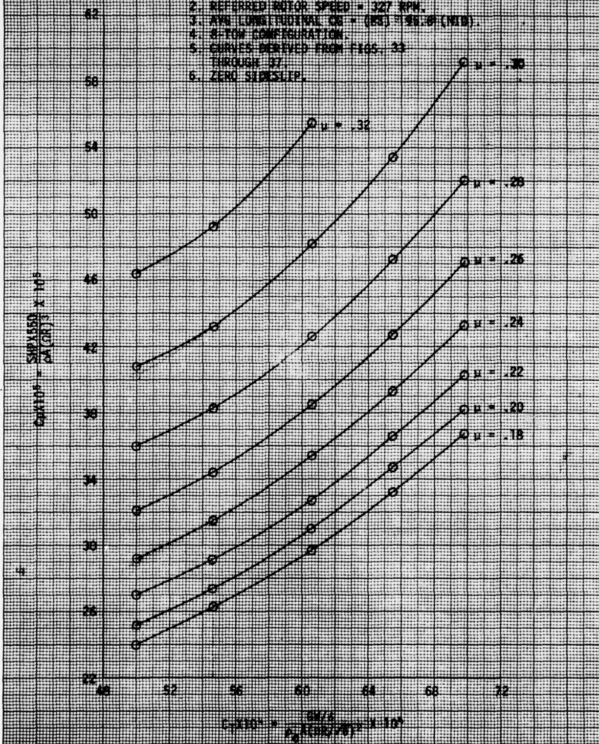
FIGURE 24 NONDIMENSIONAL LEVEL FLIGHT PERFORMANCE YAH-12 USA S/N 70-15936
