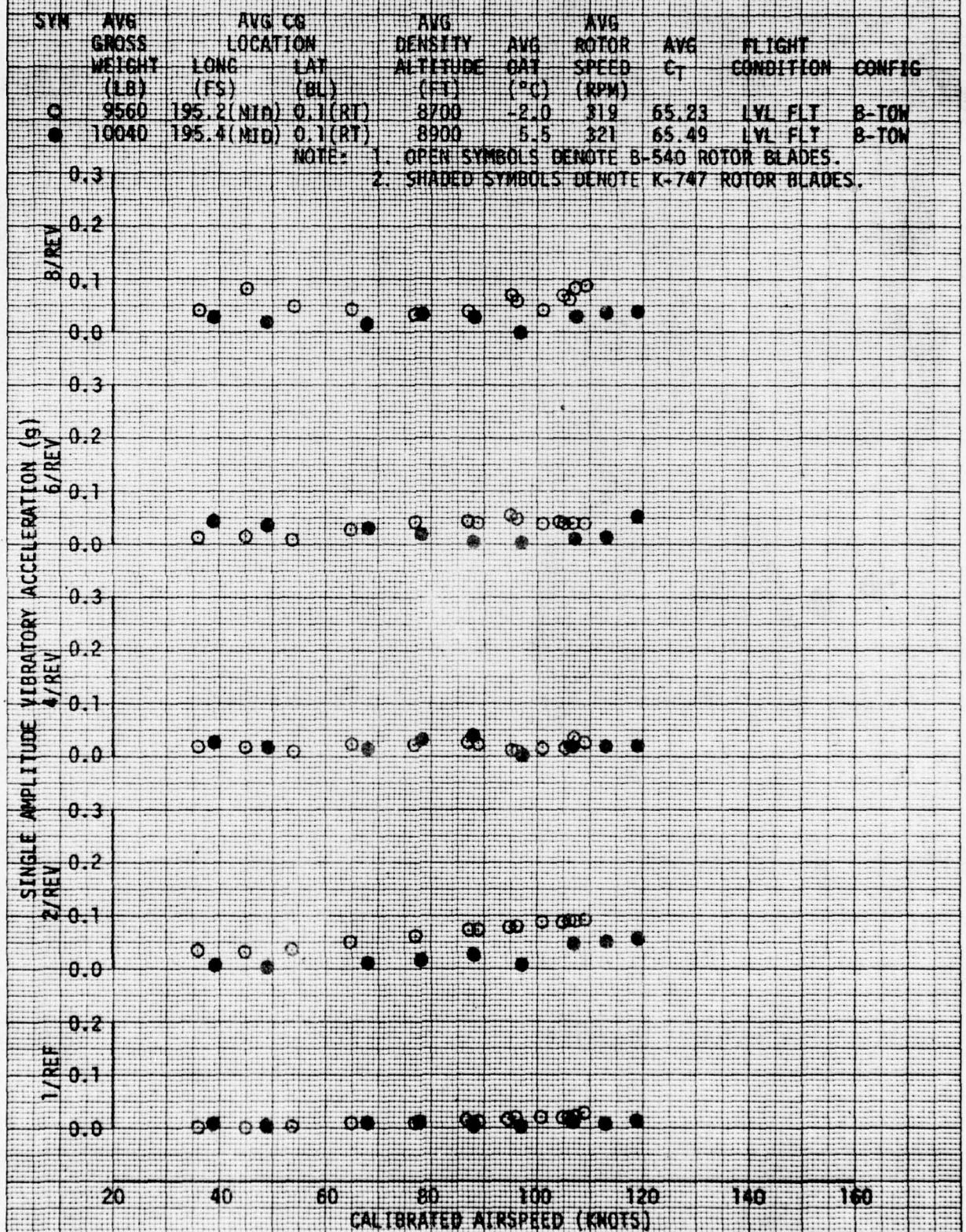
FIGURE 60 VIBRATION CHARACTERISTICS YAH-1R USA S/N 70-15986 COPILOT SEAT VERTICAL
