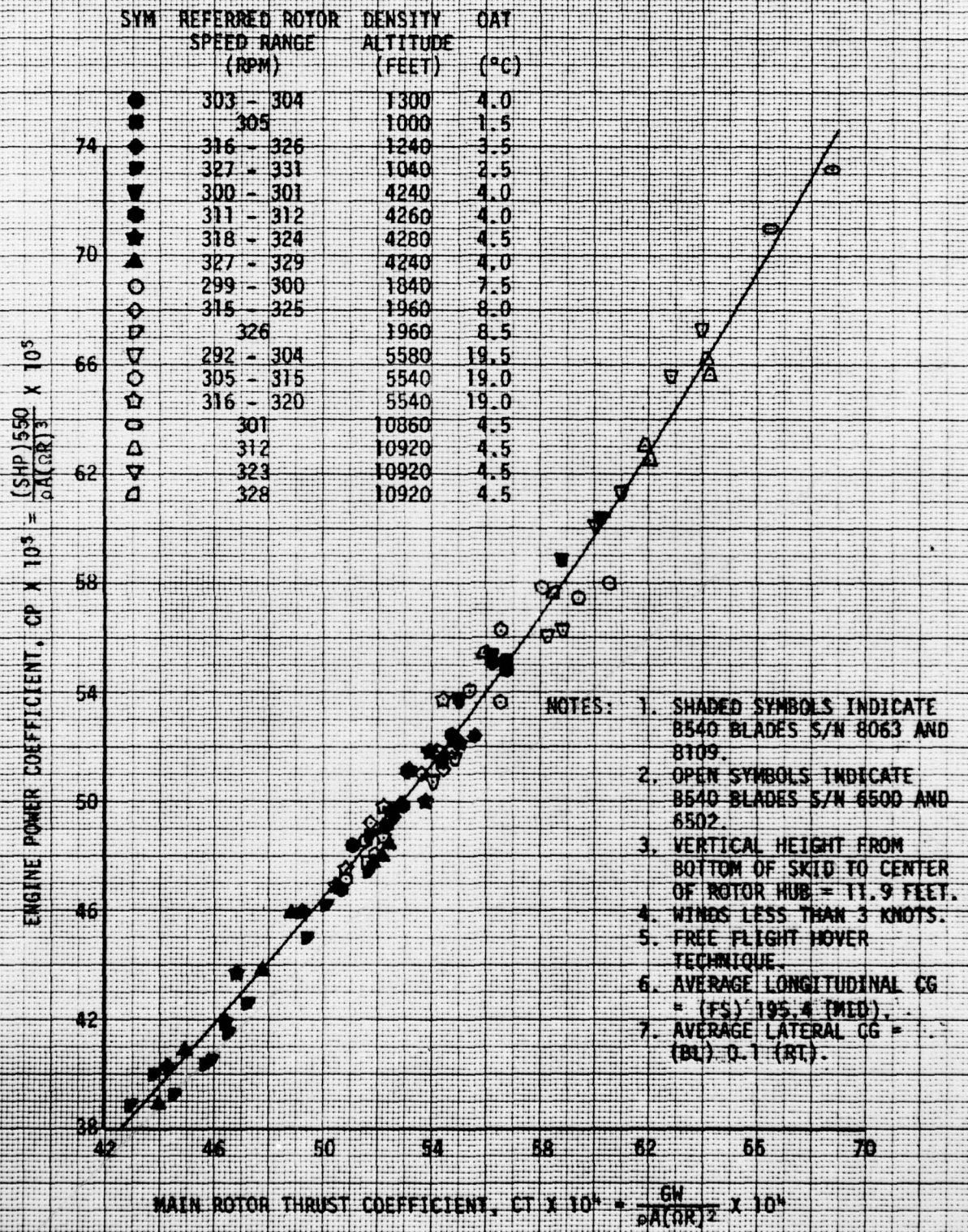
FIGURE 5 OUT-OF-GROUND EFFECT NONDIMENSIONAL HOVERING PERFORMANCE YAH-FR USA S/N 70-15936 ENGINE T53-L-703 S/N LE16124Z SKID HEIGHT = 100 FEET
