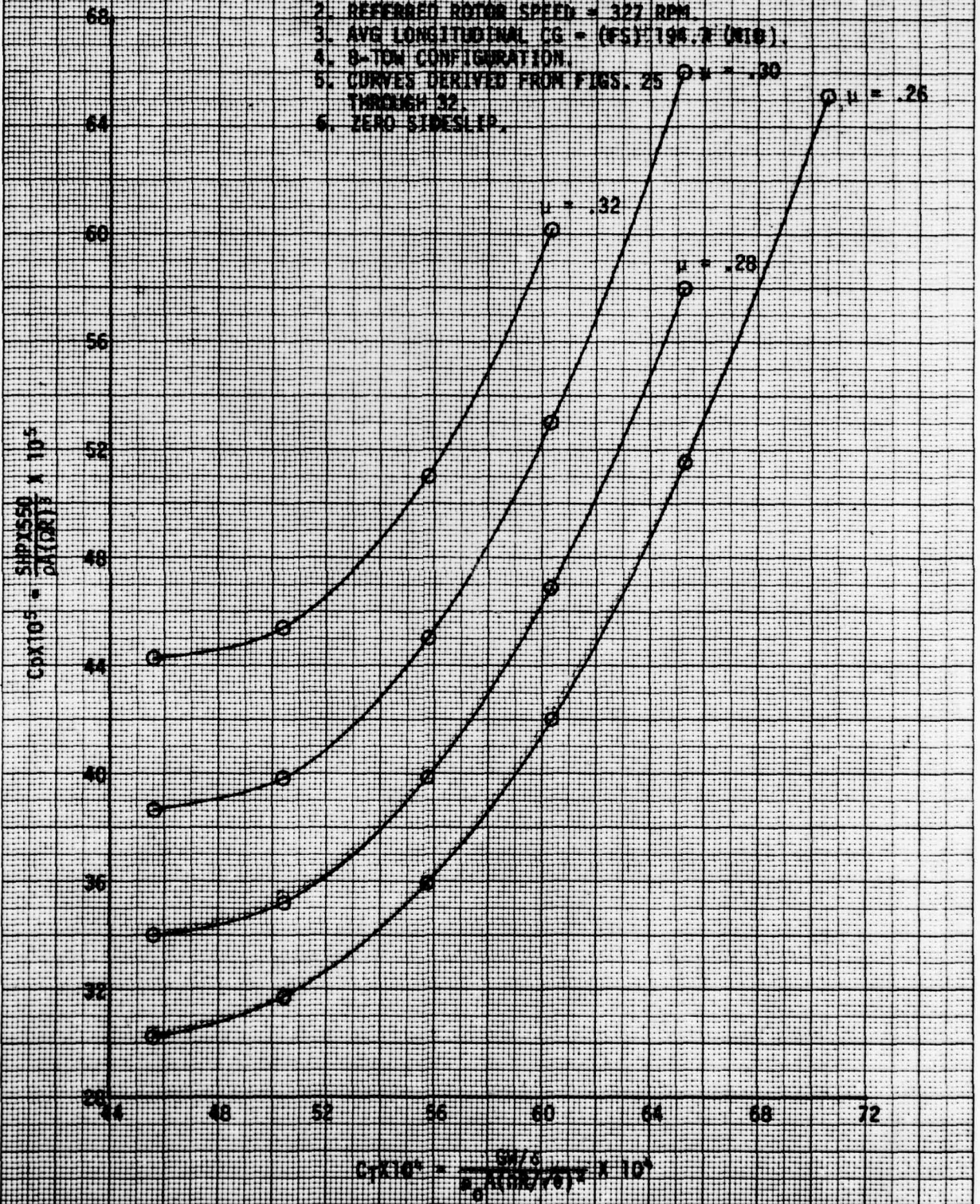
FIGURE 22 NONDIMENSIONAL LEVEL FLIGHT PERFORMANCE YAH-1B USA S/N 70-15936
