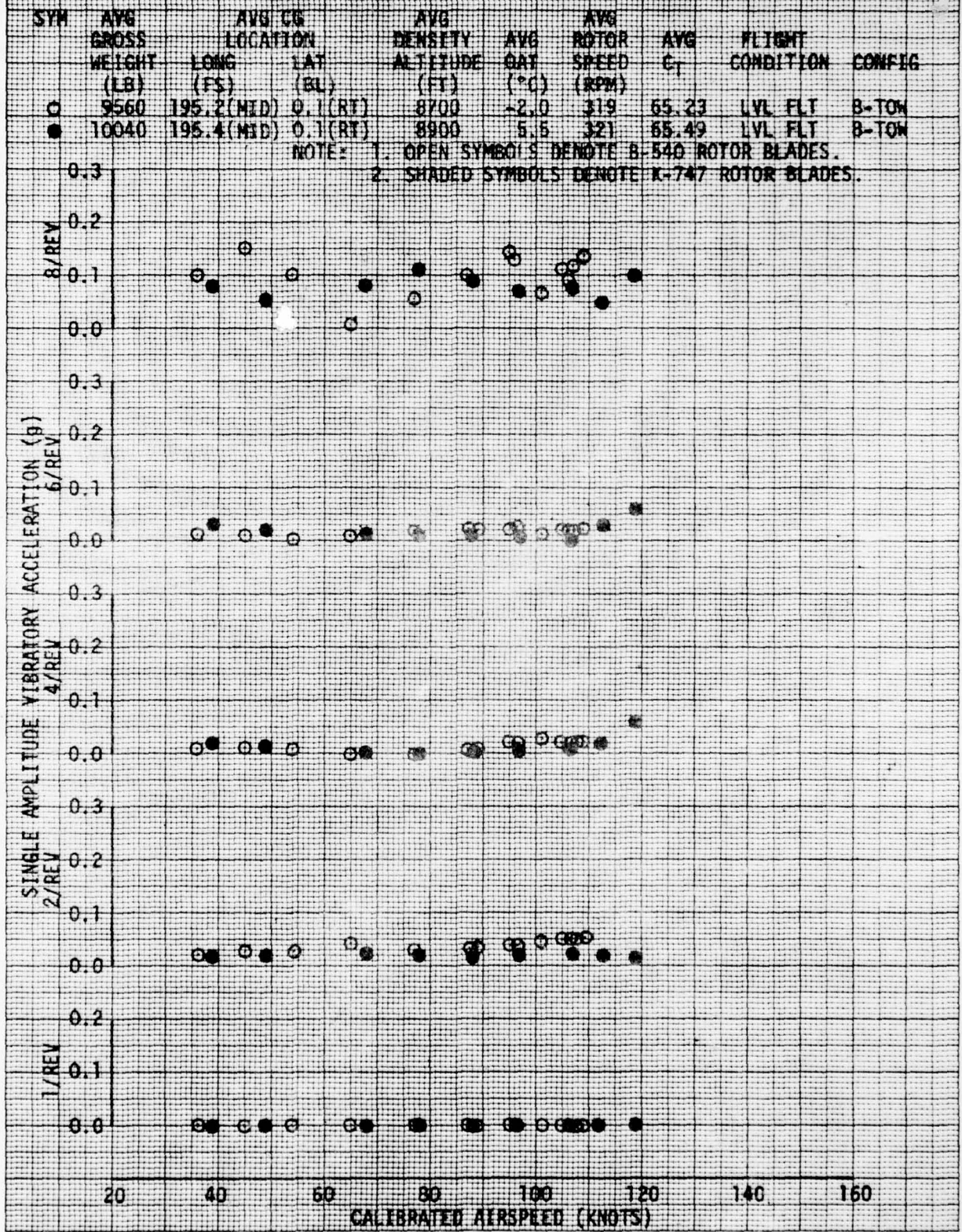
FIGURE 58 VIBRATION CHARACTERISTICS YAH-1R USA S/N 70-15936 PILOT SEAT LONGITUDINAL
