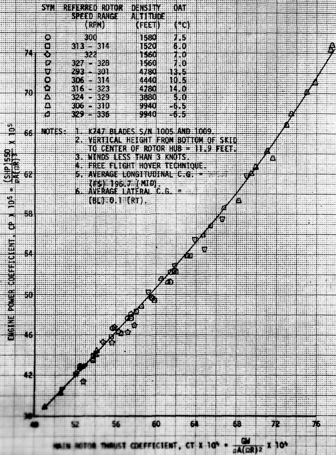
FIGURE 4 IN-GROUND EFFECT NONDIMENSIONAL HOVERING PERFORMANCE YAH-IR USA S/N 70-15936 ENGINE TB3-L-703 S/N LE15124Z SKID HEIGHT = 5 FEET
