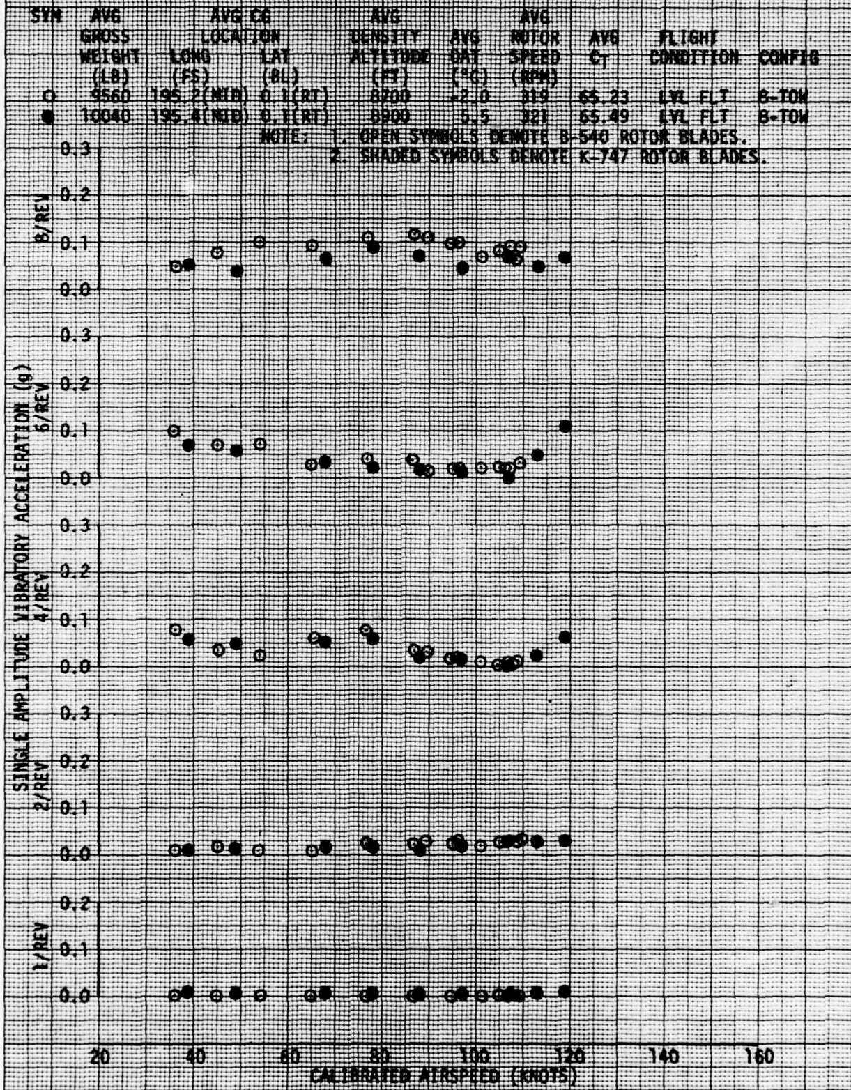
FIGURE 57 VIBRATION CHARACTERISTICS T-28C USA S/N 70-15936 PILOT SEAT VERTICAL
