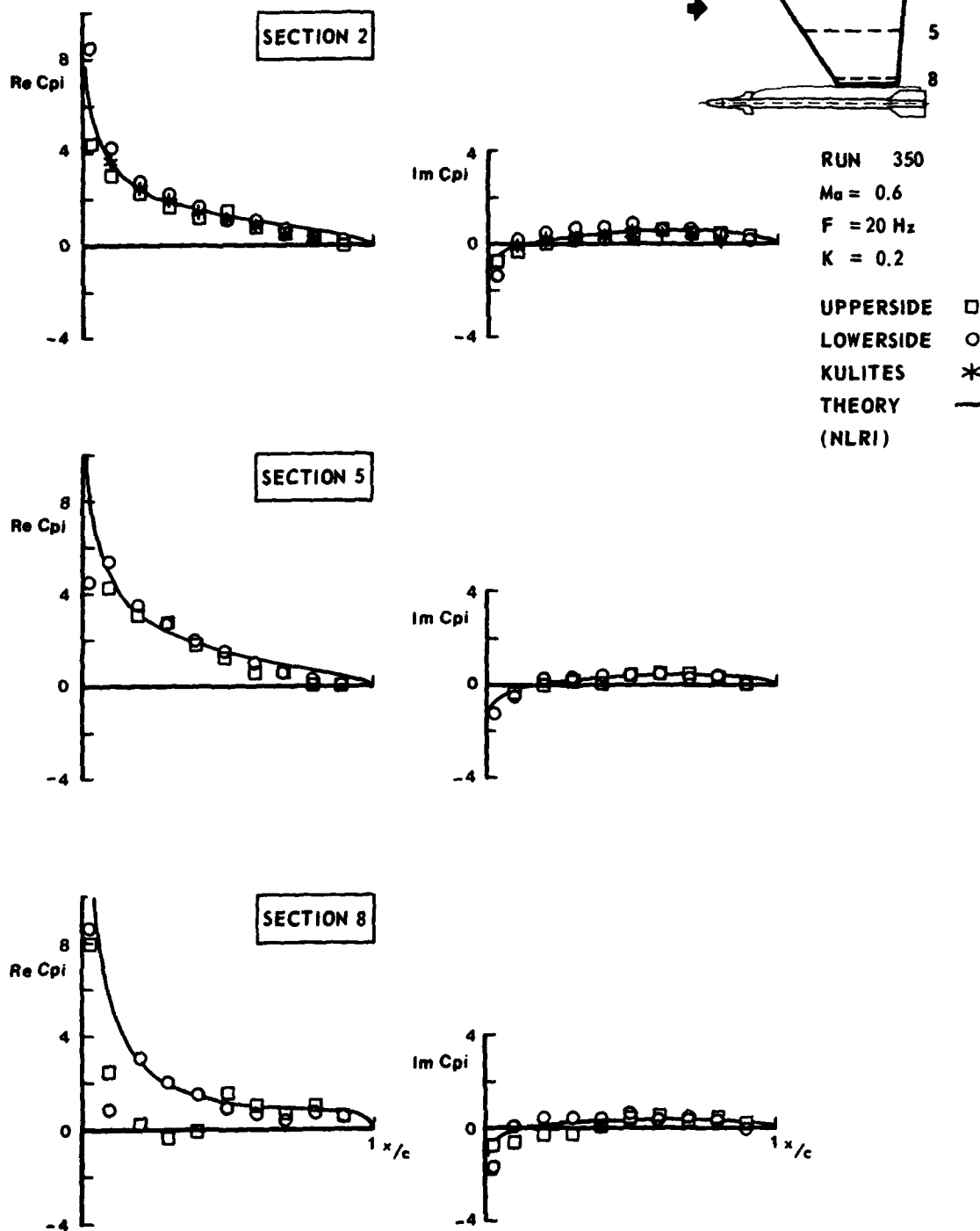
Fig. 14 Comparison of experimental and theoretical (NLRI-method) unsteady pressure distributions on the wing with complete tipstore at Ma = 0.6
