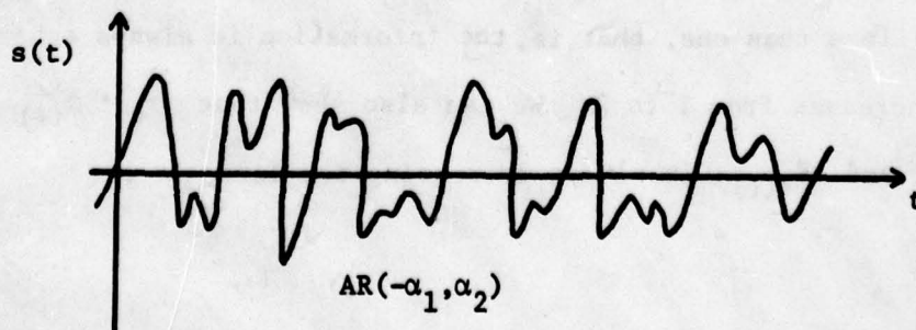
Figure 2.11 AR(2) processes with opposite sign for \alpha_1 .
