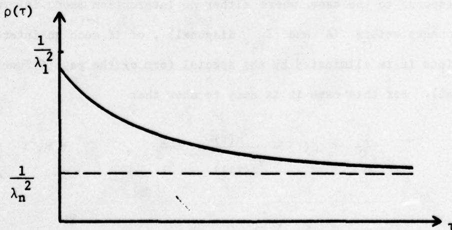
Figure 2.4. \rho(\tau) for diagonal A and M (or A and \Sigma_{\infty} ).
