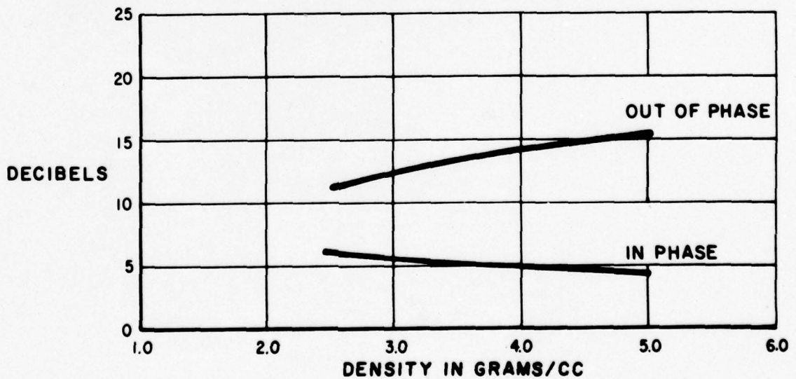
COMPOSITE BOTTOM REFLECTION COEFFICIENT
