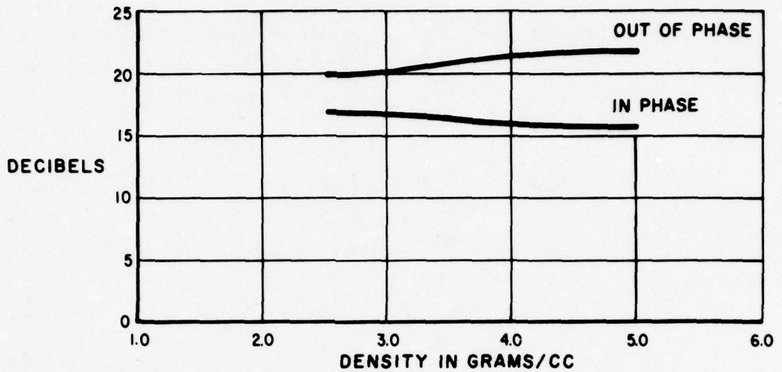
RATIO OF DIRECT PULSE TO TOTAL REFLECTED PULSE
