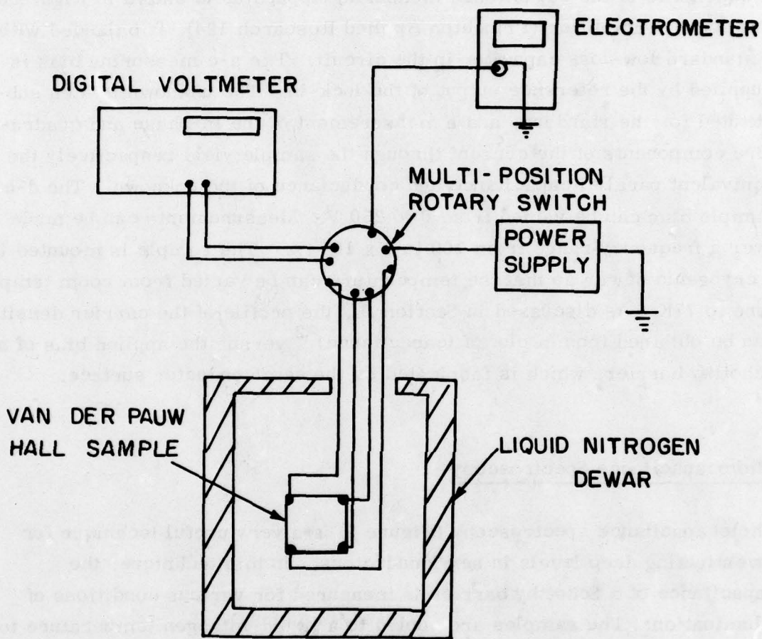
Figure 7. Schematic of Hall Apparatus
