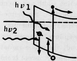
Figure 40. Schematic of the Photocapacitance Technique
