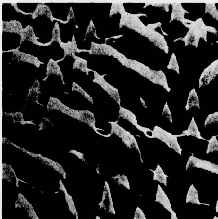
Figure 5. A-77-205 \gamma / \gamma' - \alpha (Ni Mo Ta Al) before testing C4499
