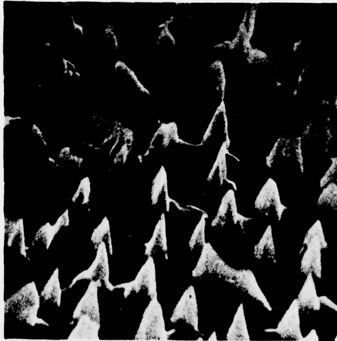
Figure 6. A-77-205 \gamma/\gamma' - \alpha (Ni Mo Ta Al) after testing C4848
