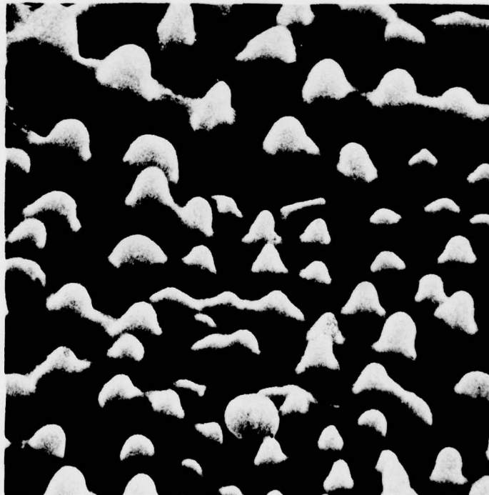
Figure 7. A-77-205 \gamma/\gamma' - \alpha (Ni Mo Ta Al) after testing showing area of arcing C4847
