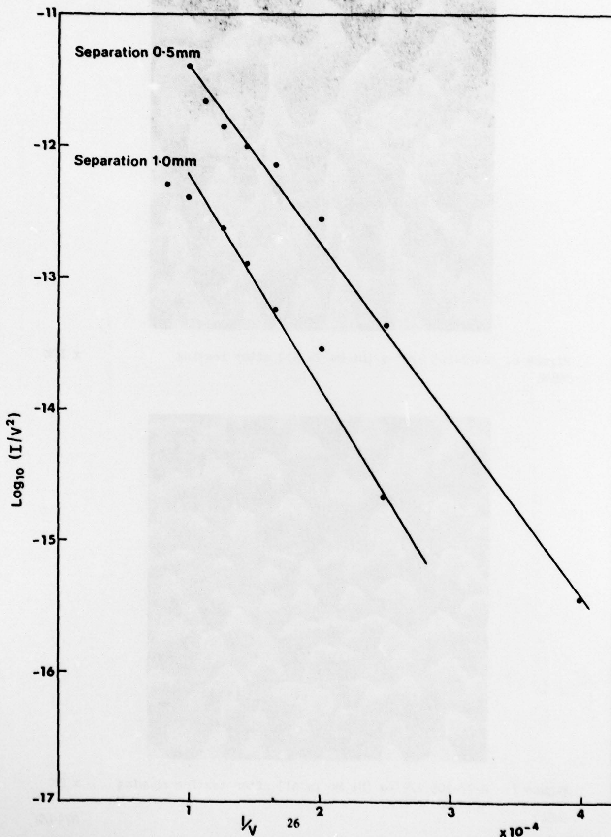
Figure 8 Fowler-Nordheim Plots with Materials A77-205 as the Cathode and at the Anode-to-Cathode Separations Shown
