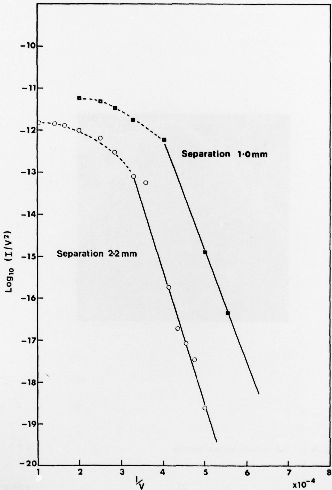
Figure 10 Fowler-Nordheim plots for TaC cathode at the anode to cathode separations shown.
