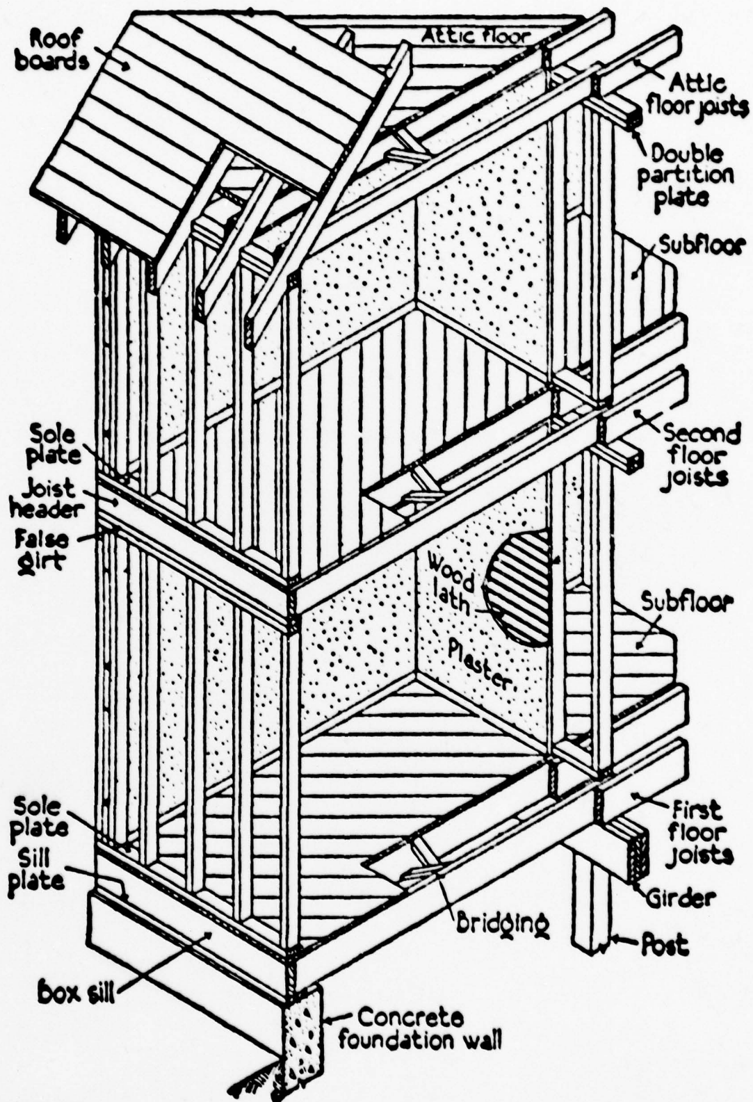
FIGURE 5. PLATFORM FRAME CONSTRUCTION 14
