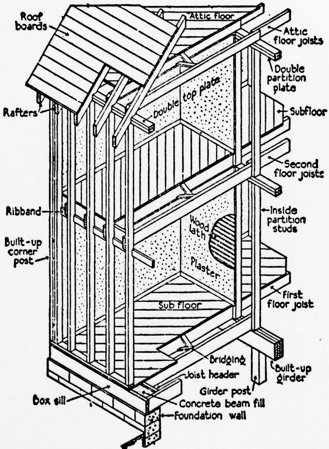
FIGURE 4. BALLOON FRAME CONSTRUCTION 13
