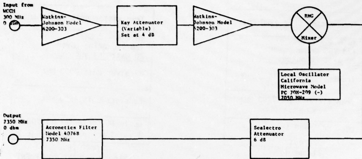
FIGURE 20 SENSOR TRANSMITTER 7350 MHz
