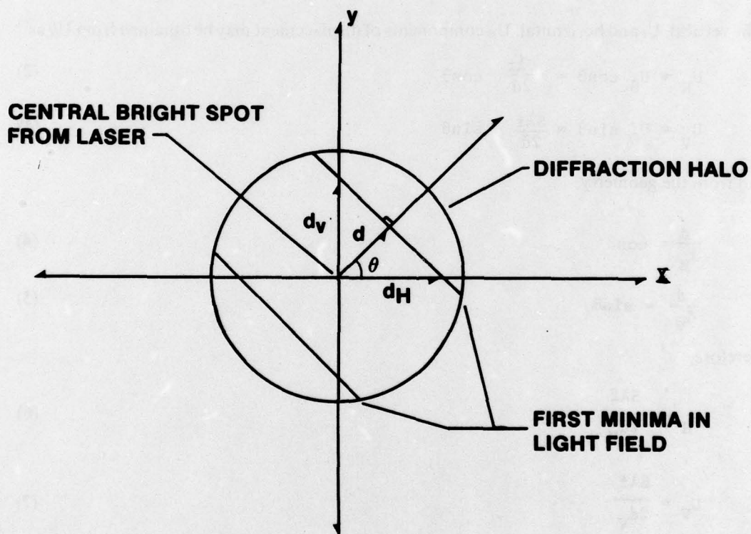
Figure 2. Diffraction halo geometry.
