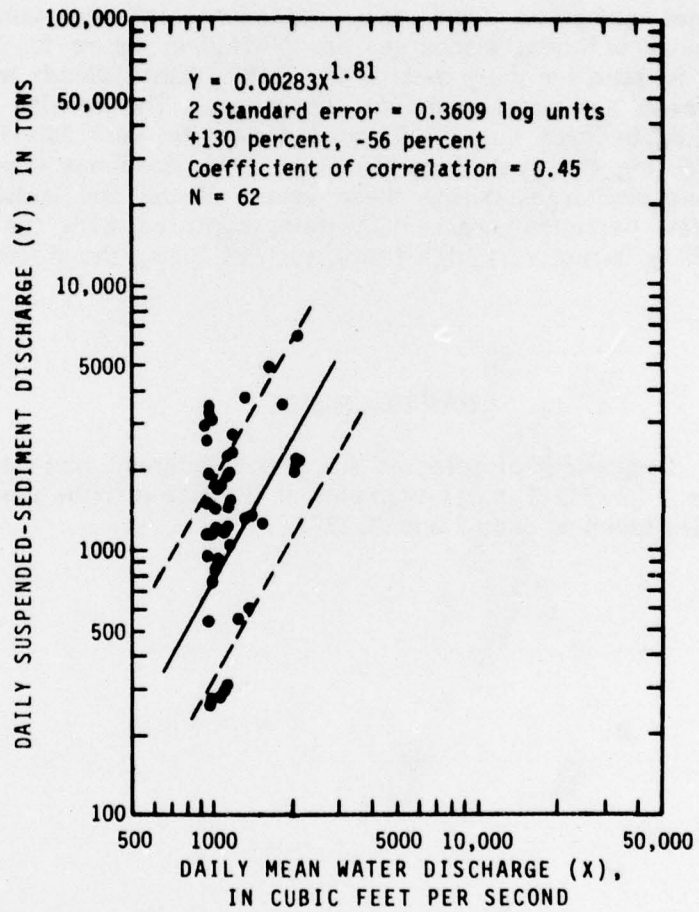
FIGURE 4. —Relation of daily suspended-sediment discharge to daily mean water discharge during periods of glacial melt (August 1974 and 1975) at station 12097850 (White River below Clearwater River, near Buckley).
