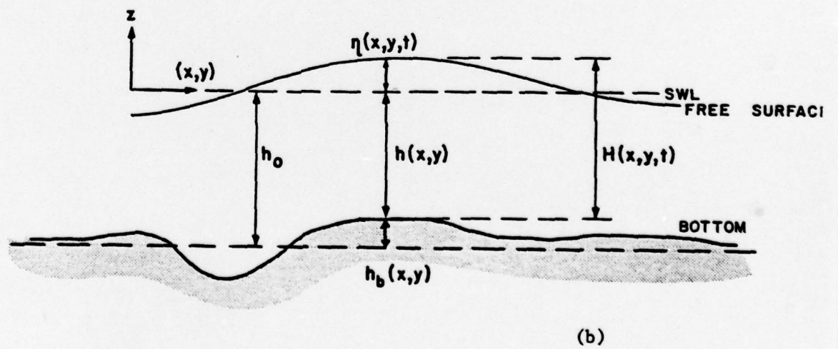
Figure 1.3 Definition Sketch (a) Bay-Inlet-Ocean System (b) Surface and Bottom Variations.
