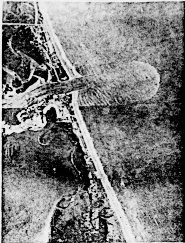
Figure 1.1a Starting Tidal Jet At Fort Pierce Inlet, Florida
