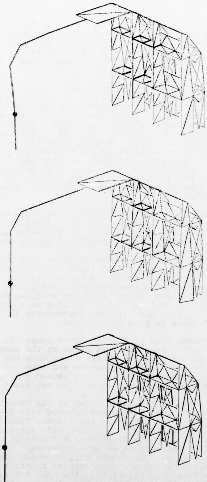
a. At 0 msec (undeformed). b. At 8.2 msec (near peak crew displacement). c. At 14.6 msec (near peak equipment displacement).
