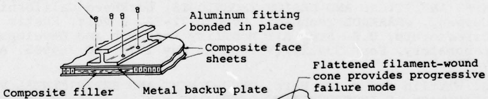
Hybrid joint
