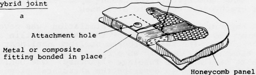
Hybrid or all composite joint
