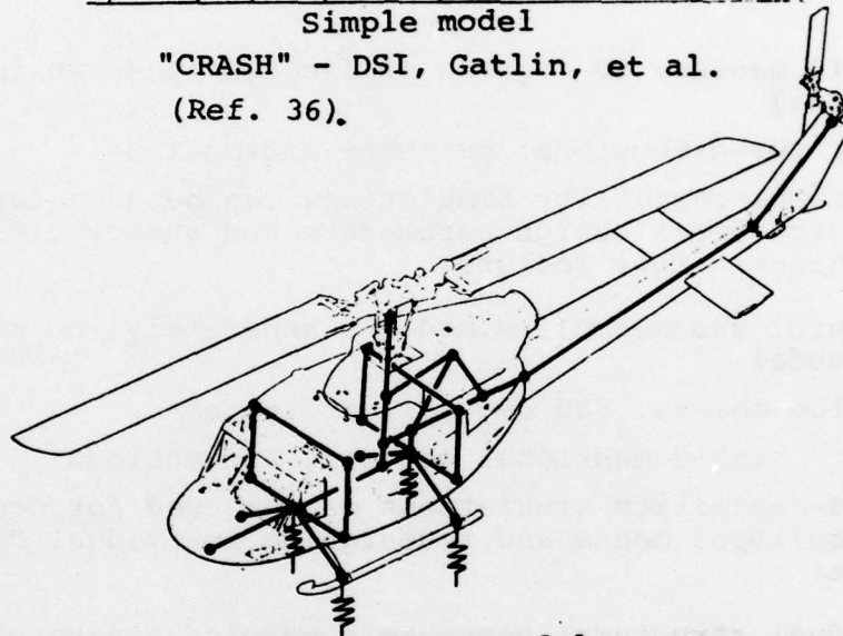
Intermediate model
