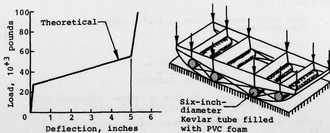
(b) Composite (Station 71.62)
