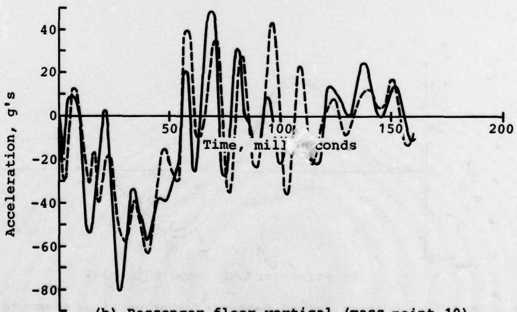
Figure A-33. Comparisons of pilot and passenger floor vertical responses for 30 fps vertical impact on rigid surface for metal and composite airframes with landing gear up.
