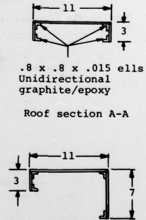
Doorpost section B-B
