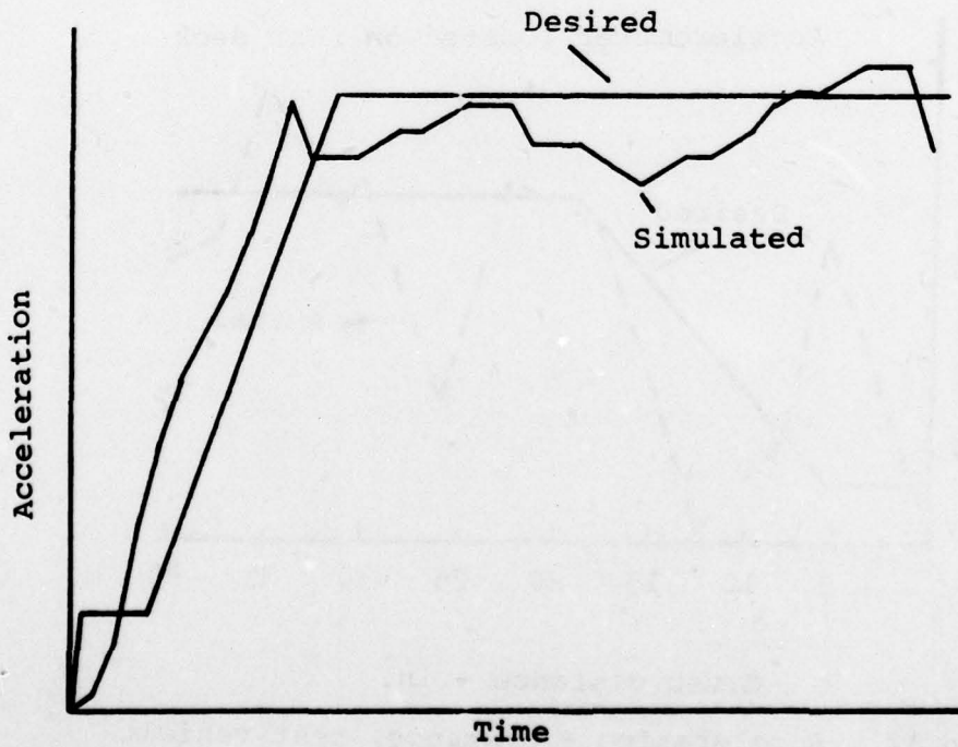
Figure 10. Simulated crash characteristics - 50 mph (Reference 13).
