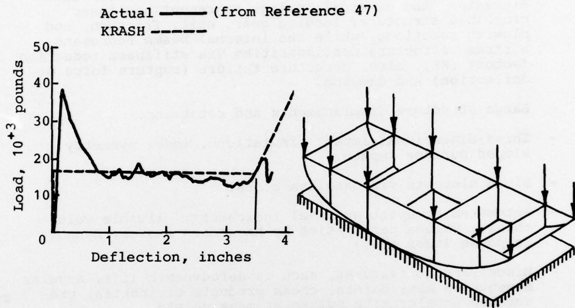
(a) Metal (Station 71.62)
