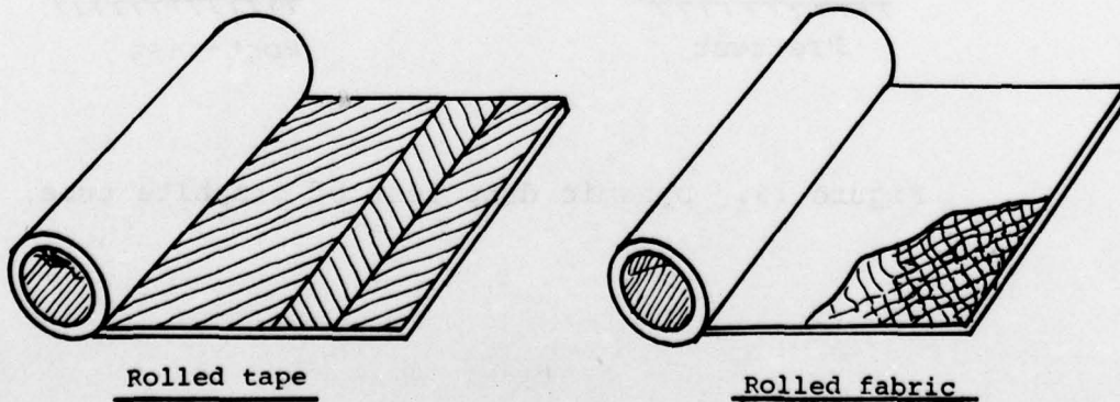
Figure 20. Test specimen construction techniques.
