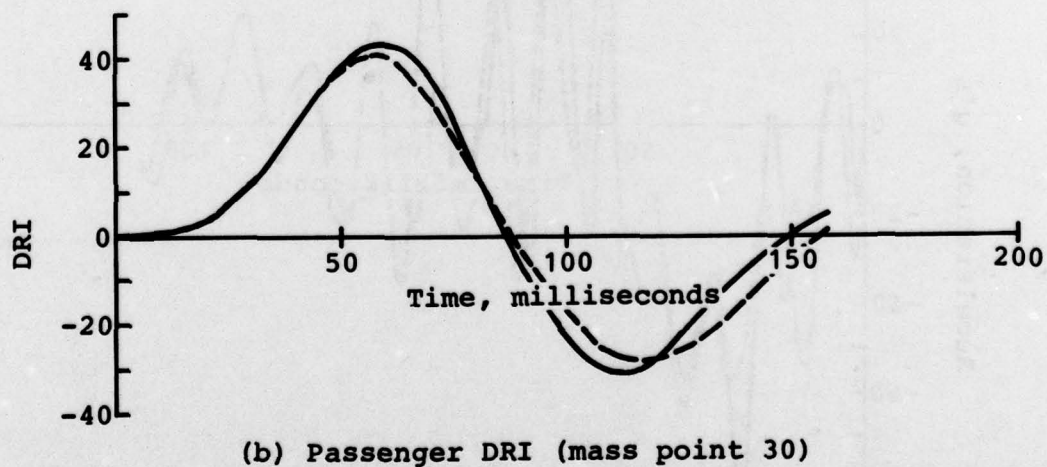
Figure A-32. Comparisons of passenger seat vertical response and DRI for 30 fps vertical impact on rigid surface for metal and composite airframes with landing gear up.
