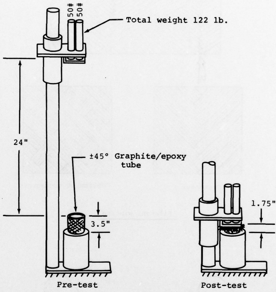
Figure 19. Dynamic drop test of graphite tube.
