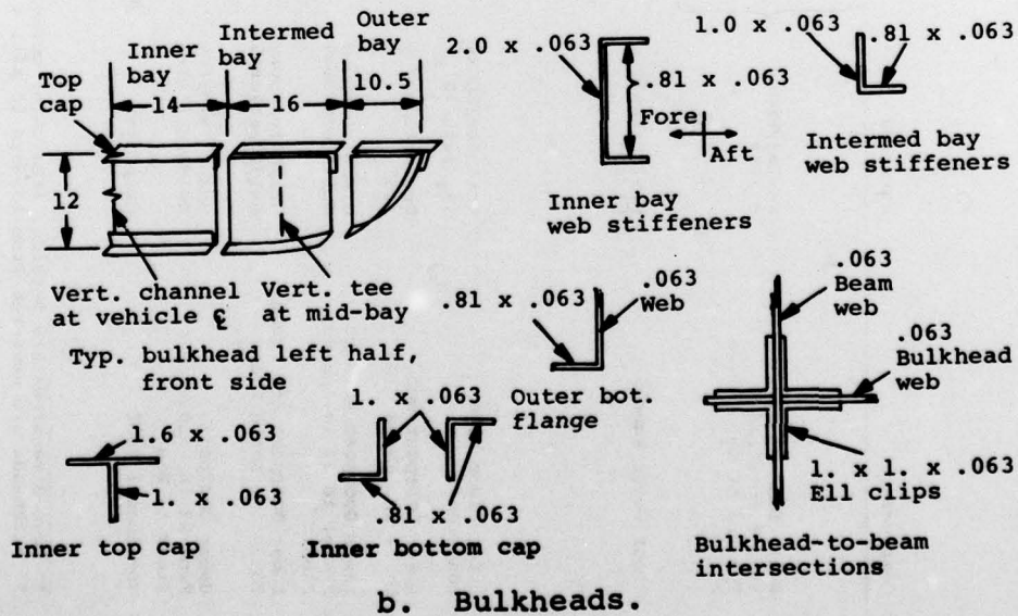
Figure B-1. Actual baseline fuselage section details.
