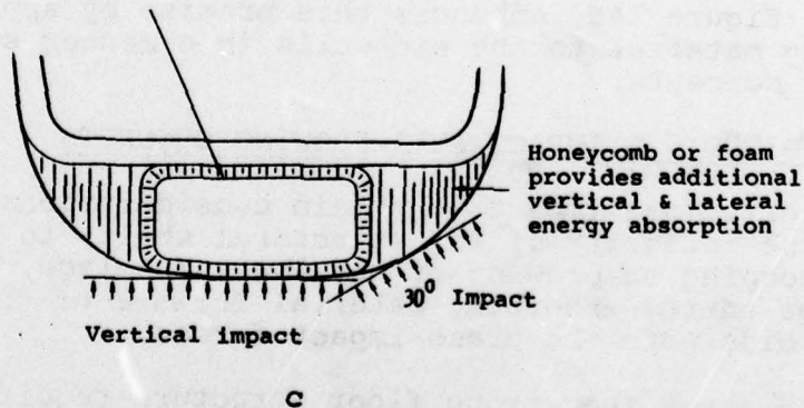
Figure 33. Energy absorption concepts - tubular construction (oblique vertical impact).
