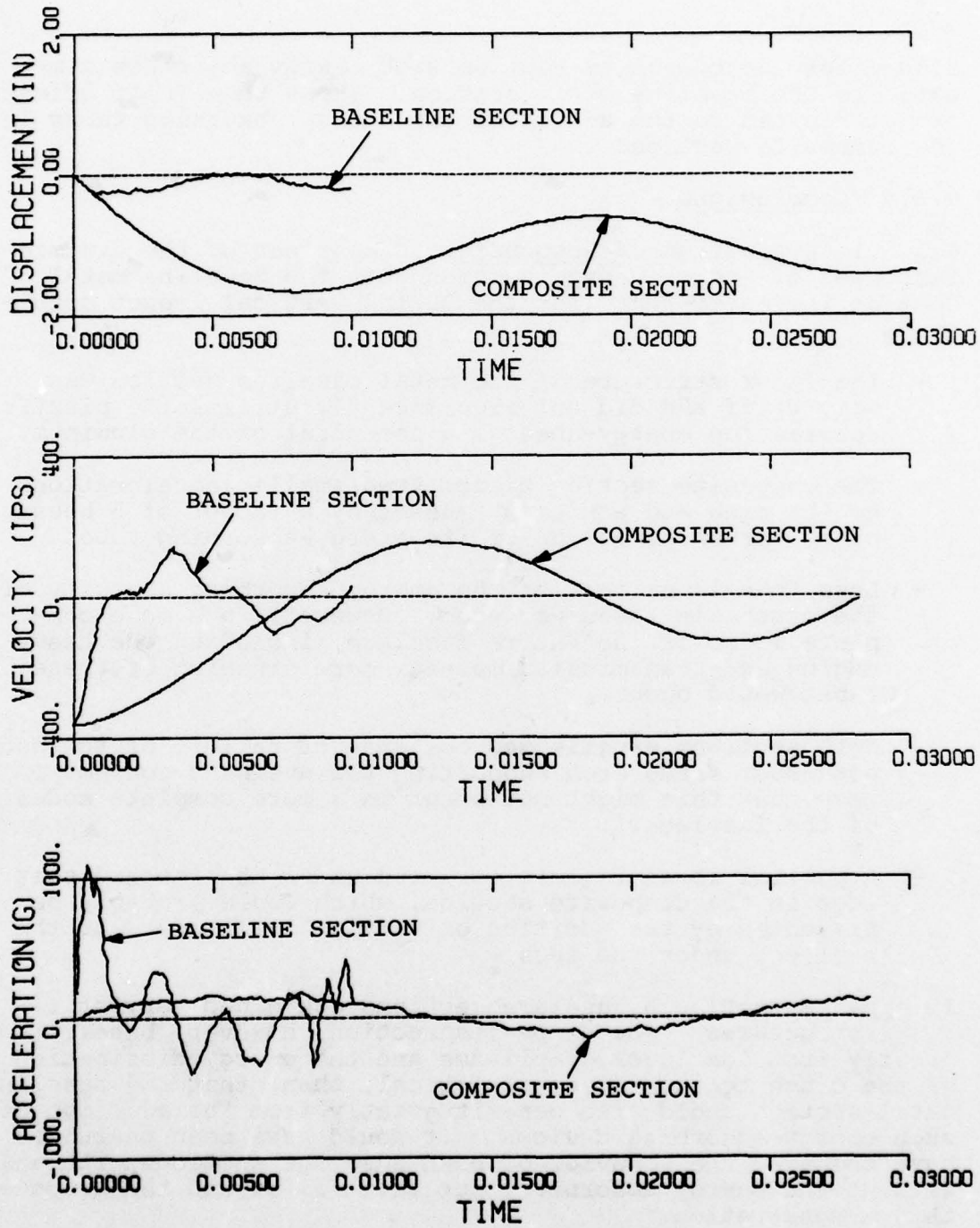
Figure 61. Comparison of vertical motion histories of the crew masses.
