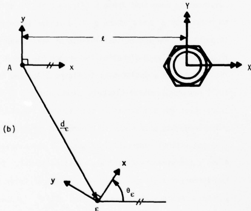
Figure 2-3: Relative Task with Horizontal Initial Position
