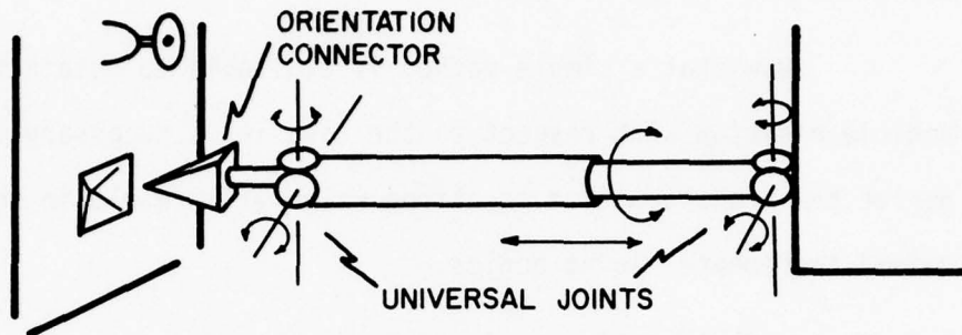
Figure 2-10: Orientation Manipulator for Tasks with Built-In Sockets
