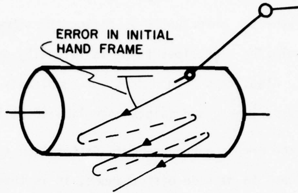
Figure 2-8: Scraping Cylinder with Error in Initial Hand Position
