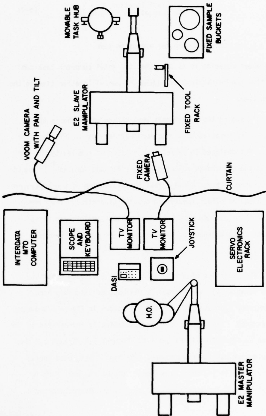
Figure 5-3: Schematic of Experimental Layout
