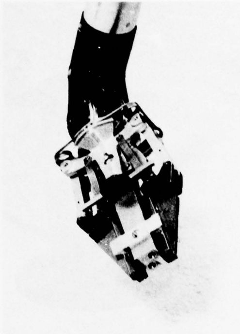
Figure 5-6: Proper Seating of Tool Handle in End Effector
