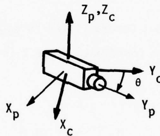
Figure E-2: Camera Panned Through Angle \theta
