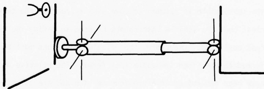
Figure 2-11: Orientation Manipulator with Magnetic Coupler for Tasks without Built-In Sockets
