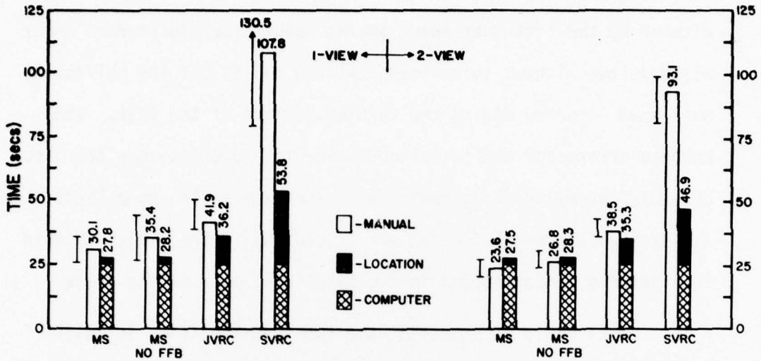
Figure 5-19: Average Valve Operation Time (Each bar represents the average time for one subject to open or close a valve. The capped lines represent the total range of the subject.)
