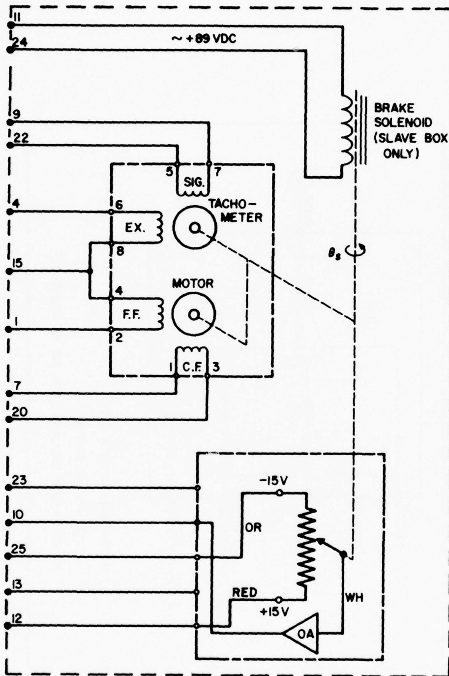
Figure D-7: Gearbox Schematic
