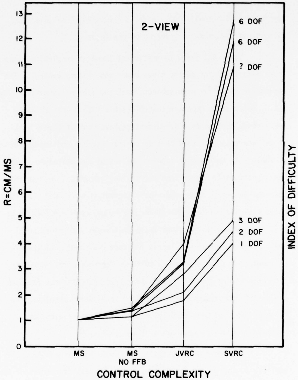
Figure 5-25: Control Mode Ratios and Index of Difficulty Versus Control Complexity for Two Views
