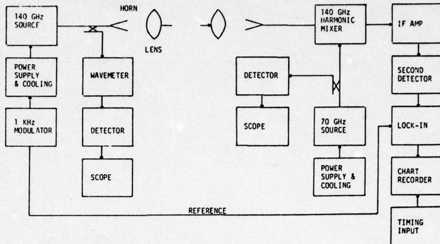
Figure 11. 140 gigahertz system diagram.
