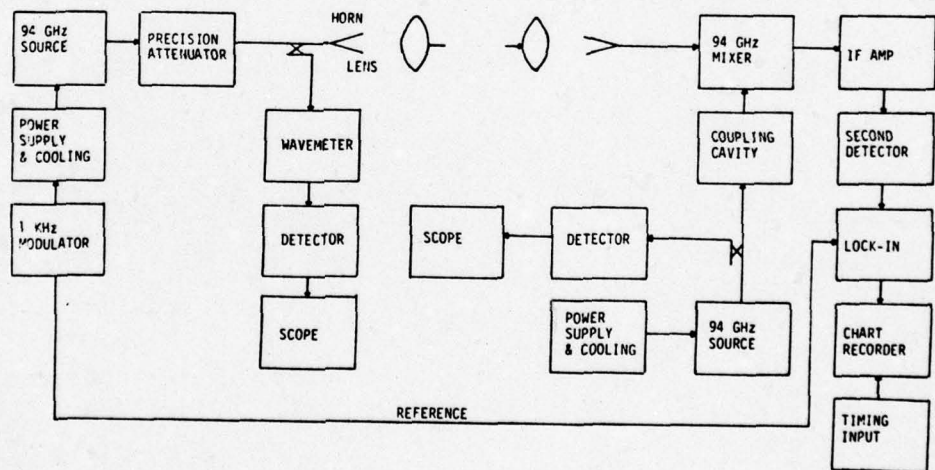
Figure 10. 94 gigahertz system block diagram.
