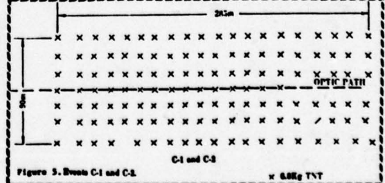
Figure 5. Events C-1 and C-2.
