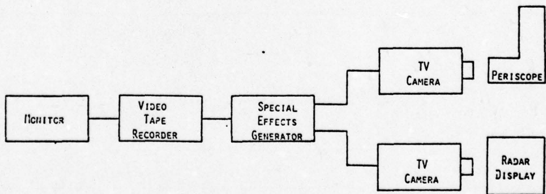
FIGURE 4. SCHEMATIC DRAWING OF EO/RADAR MONITORING AND RECORDING SYSTEM
