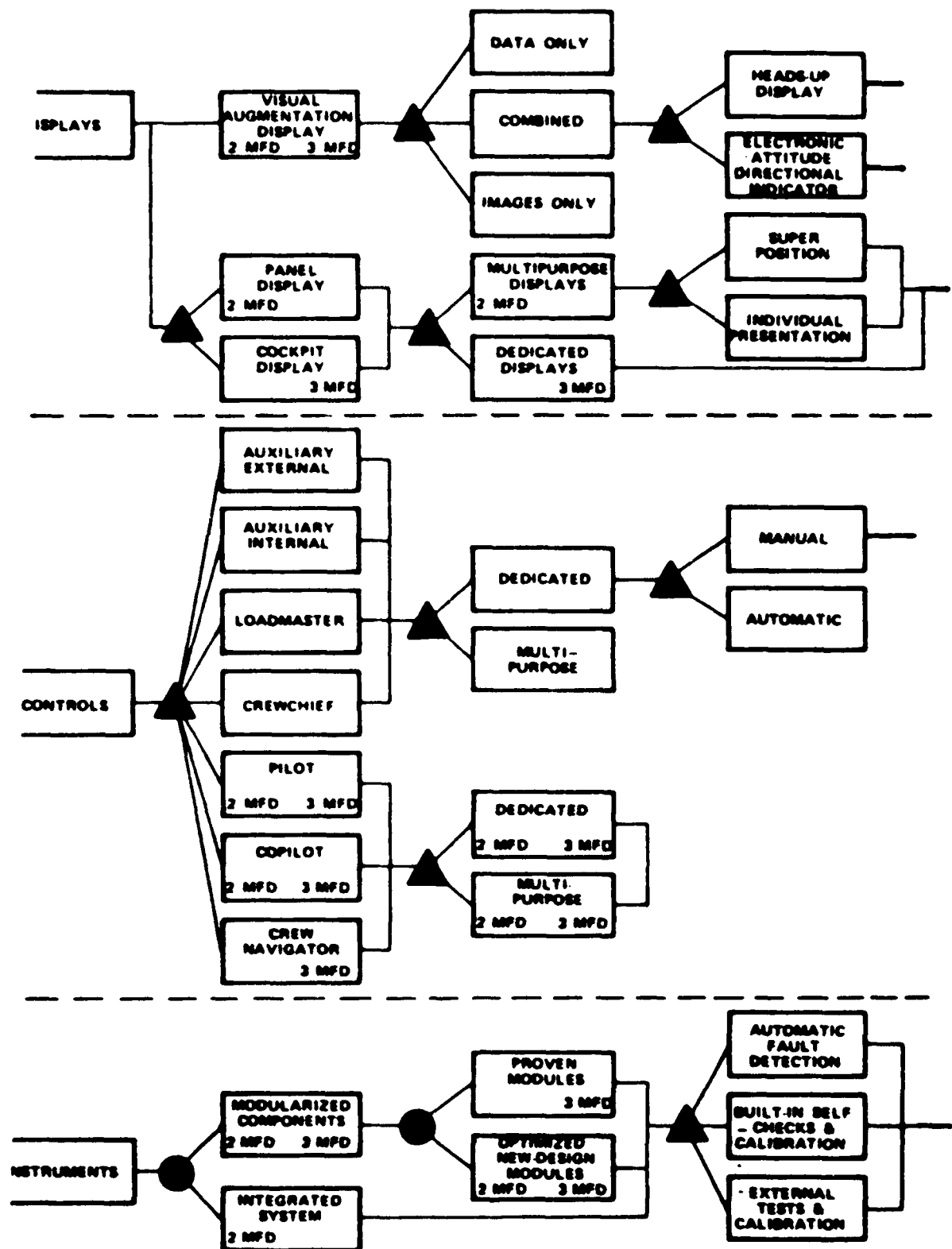
Figure 7 AVIONICS OPTIONS
