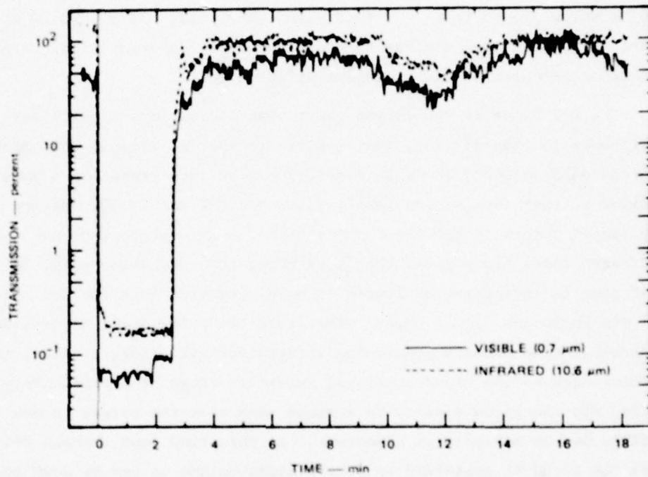
FIGURE 8 EVENT C-2 TWO-WAVELENGTH TRANSMISSION
