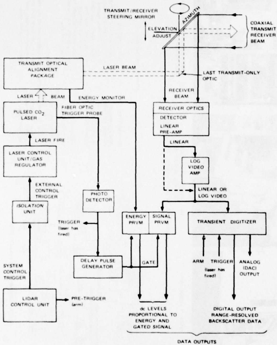
FIGURE 2 ASL LIDAR FUNCTIONAL DIAGRAM
