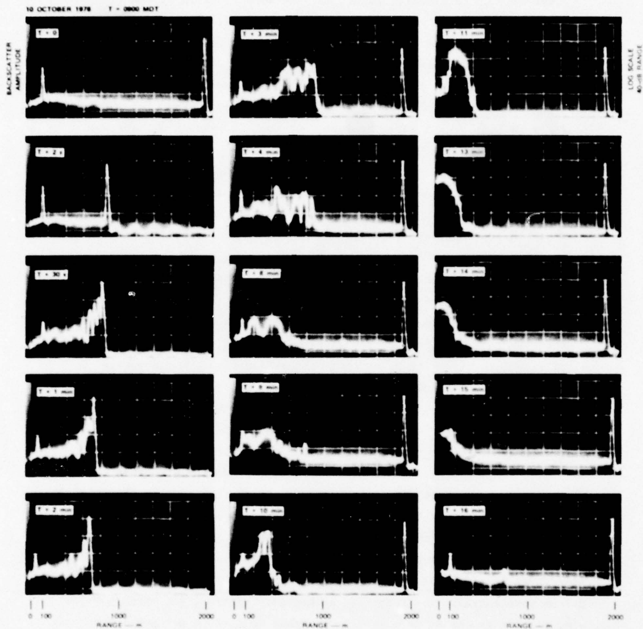
FIGURE 7 EVENT C-2 10.6- \mu m BACKSCATTER DATA
