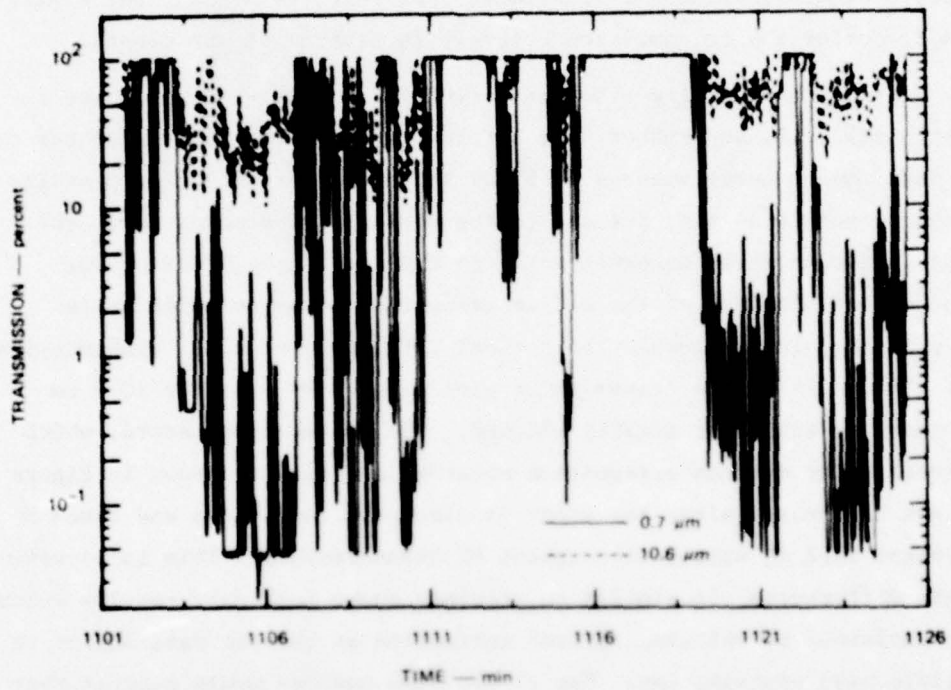
FIGURE 11 EVENT G-1 10.6-μm BACKSCATTER DATA AND TWO-WAVELENGTH TRANSMISSION
