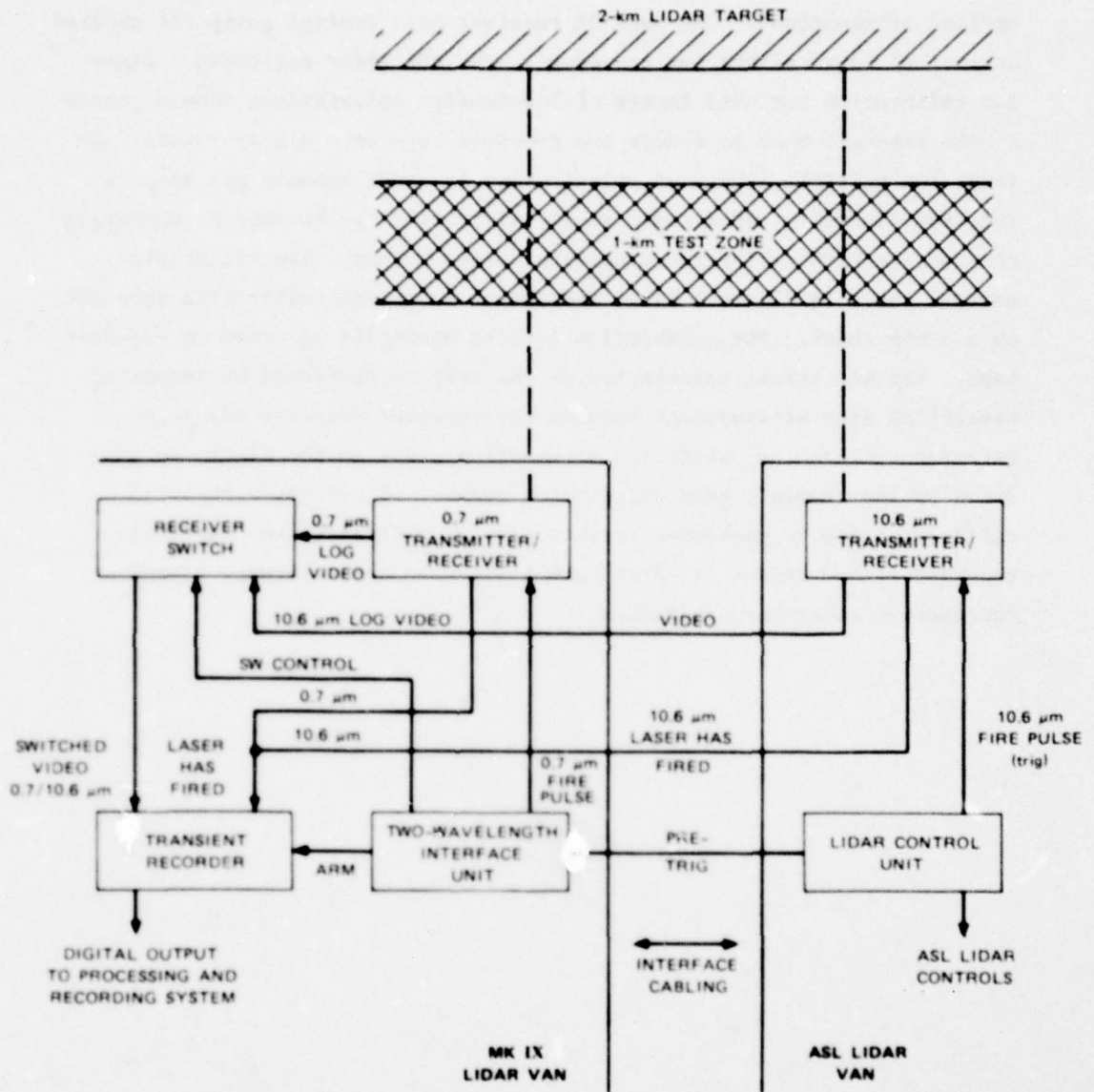
FIGURE 4 TWO-WAVELENGTH INTERFACE BLOCK DIAGRAM
