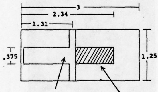
Figure 6.4 Side View of Short Transformer in Large Filter
