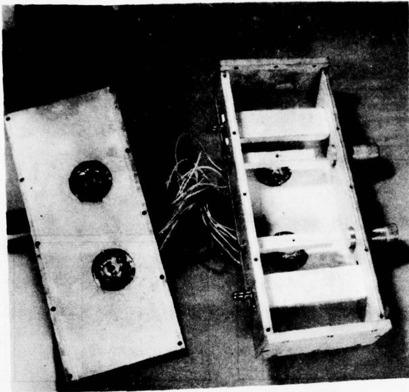
Figure 6.5 Inside View of Large Comb Line Filter
