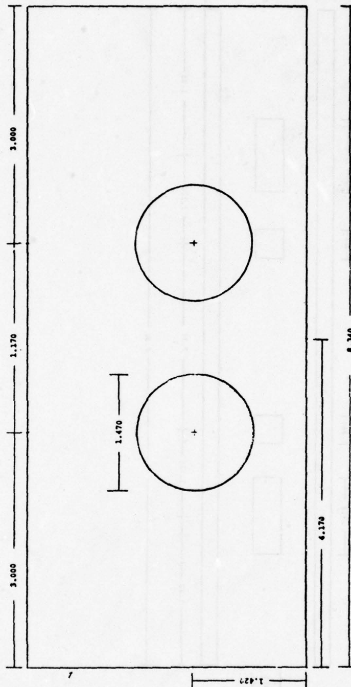
Figure 6.1 Top Plate of Large Comb Line Filter
