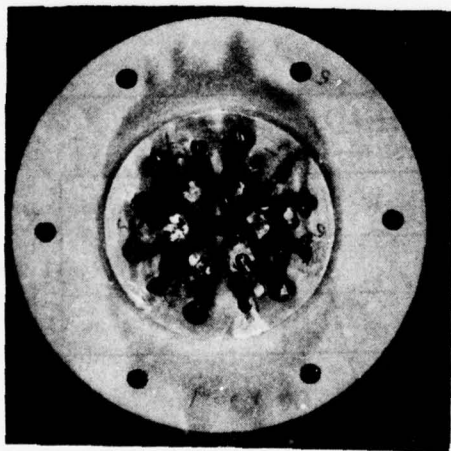
Figure 6.6 Tuning Plate for Large Comb Line Filter
