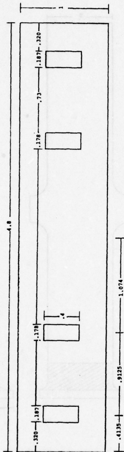
Figure 6.10 End Dimensions for Small Comb Line Filter
