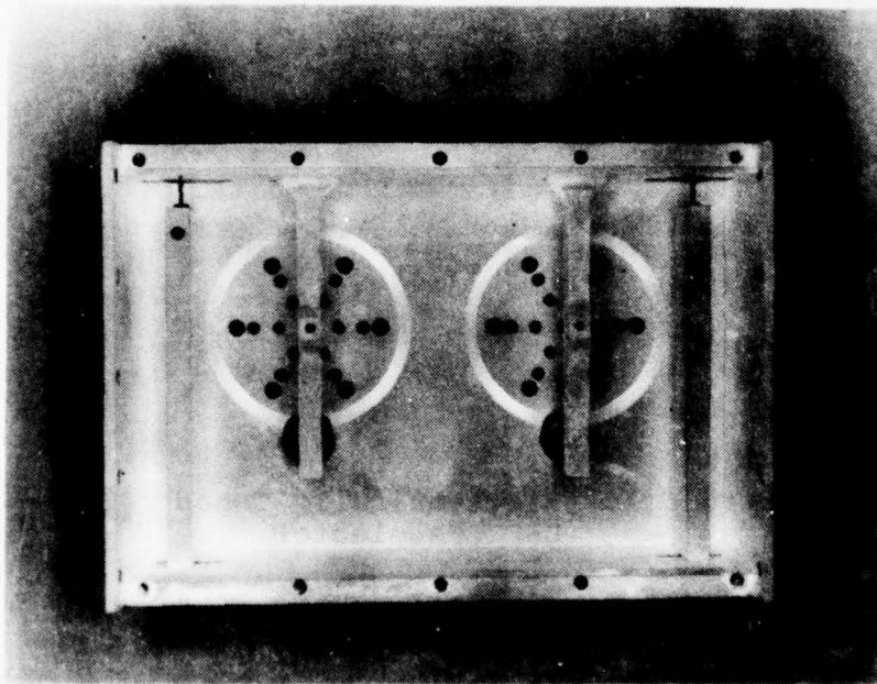
Figure 6.12 Small Comb Line Filter
