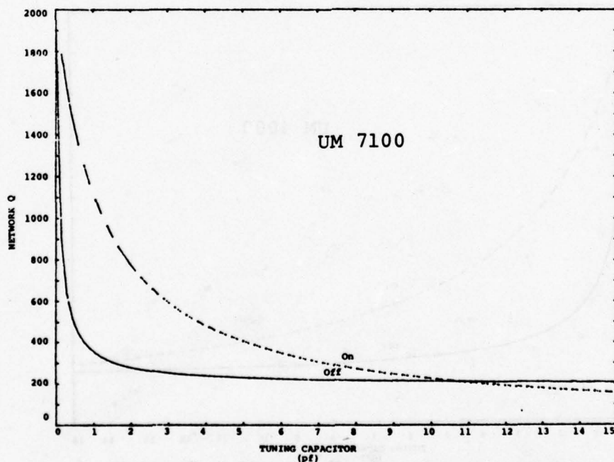
Network Q Versus Tuning Capacitance
