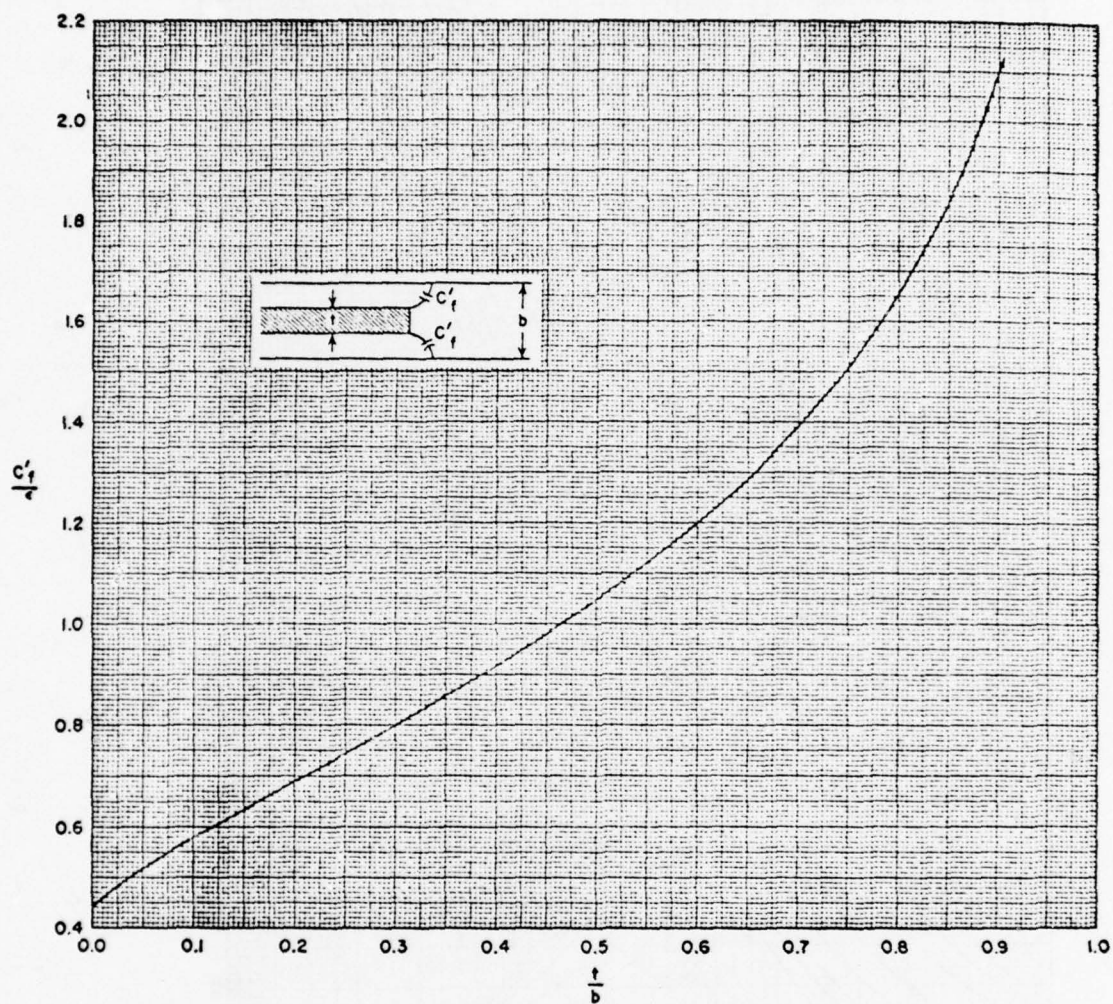
FIGURE 3.4 Fringing Capacitance
