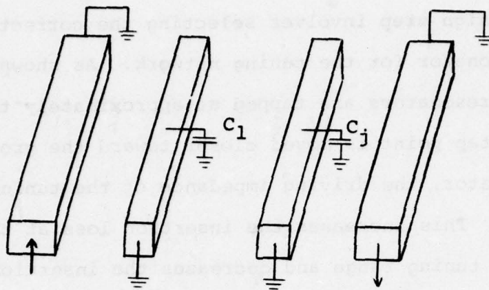
FIGURE 5.4 Comb Line Filter with Center Tapped Resonators
