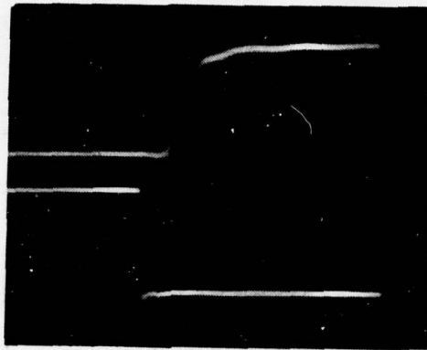
Figure 7.10a Tuning Speed from Diode Off to On (2us/div)
