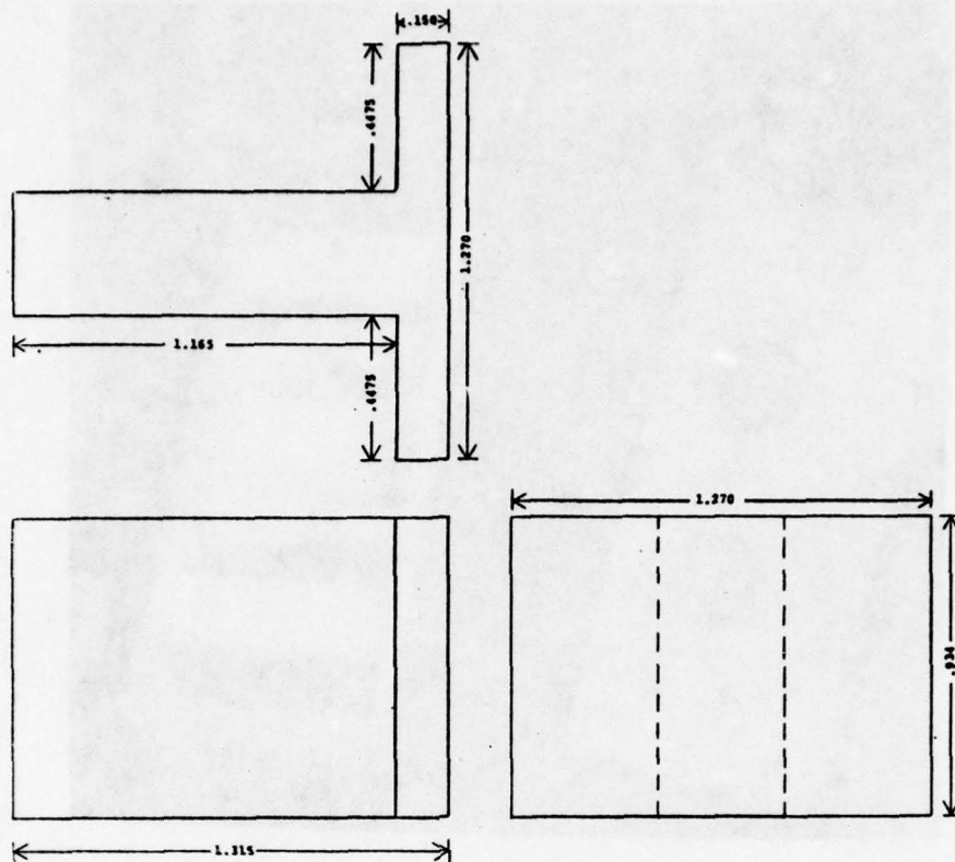
Figure 6.3 Reduce Length Transformer for Large Filter
