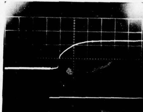
Figure 7.10a Tuning Speed from Diode Off to On (2us/div)
