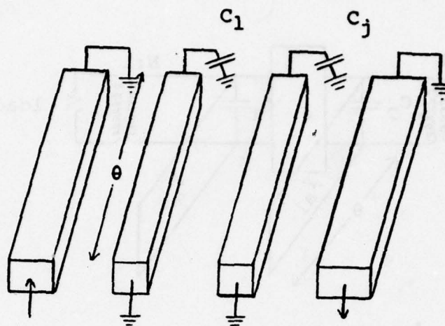
FIGURE 5.1 General Comb Line Filter
