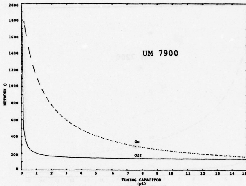
Network Q Versus Tuning Capacitance
