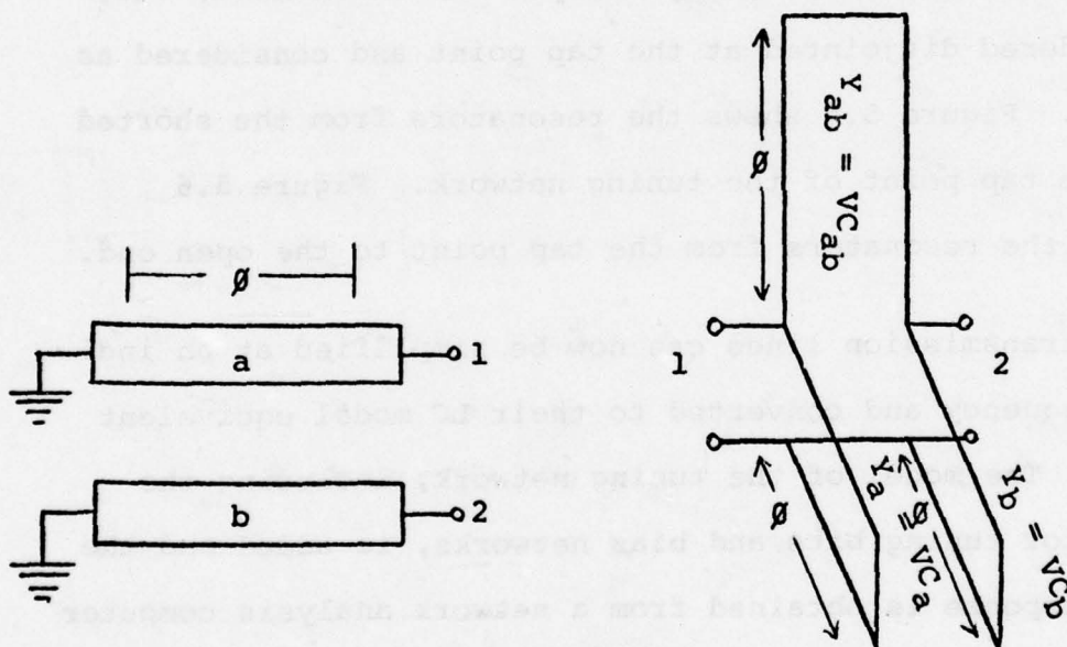
FIGURE 5.5 Transmission Line Pair with Shorted Ends
