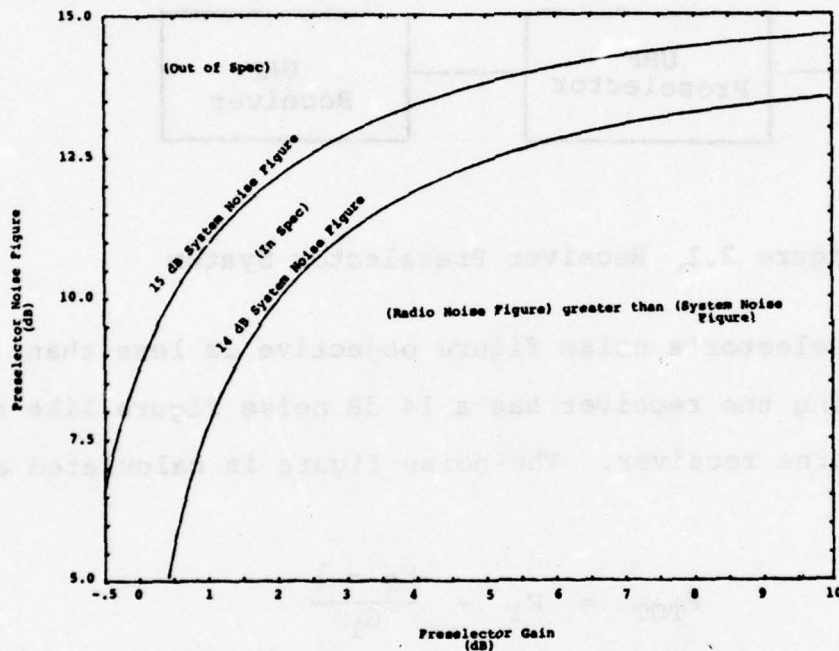
Figure 2.2 Preselector Noise Figure Versus Preselector Gain
