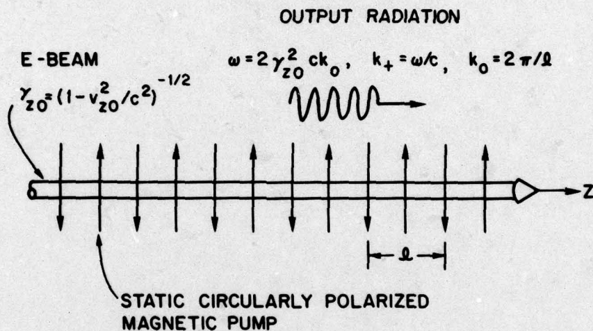
Figure 1 — Schematic of the free electron laser model. The adiabatic build-up of the pump field is not shown, and occurs to the left of the figures where the unmodulated beam enters.
