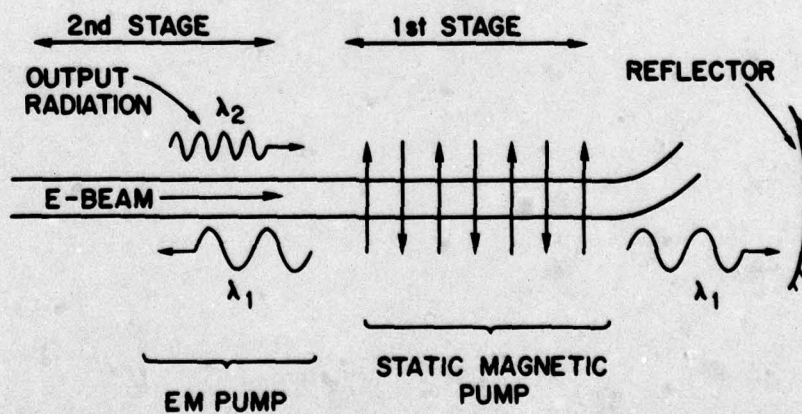
Figure 2 — Schematic of the two-stage free electron laser concept. The electron beam enters at left. Radiation scattered at wavelength \lambda_1 from the static magnetic pump of wavelength \ell in the first stage is reflected to act as an electromagnetic pump in the second stage. The final scattered radiation is at wavelength \lambda_2 \approx 1/(8\gamma_z^4) .
