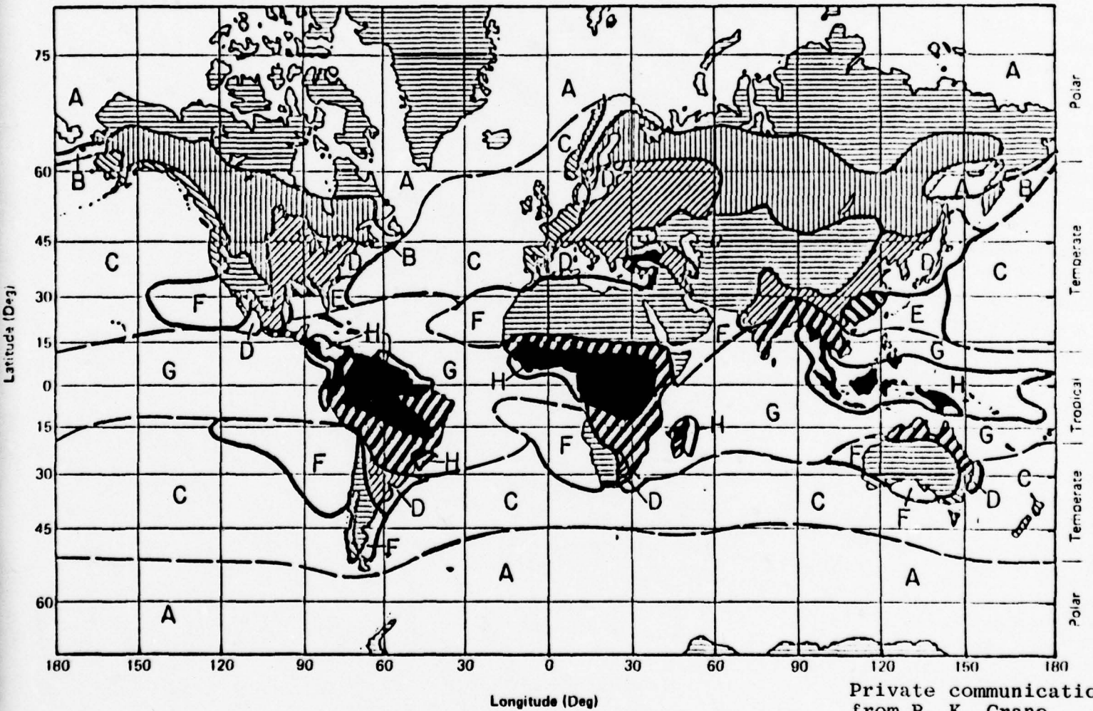
Fig. 1. Rain rate climate regions
