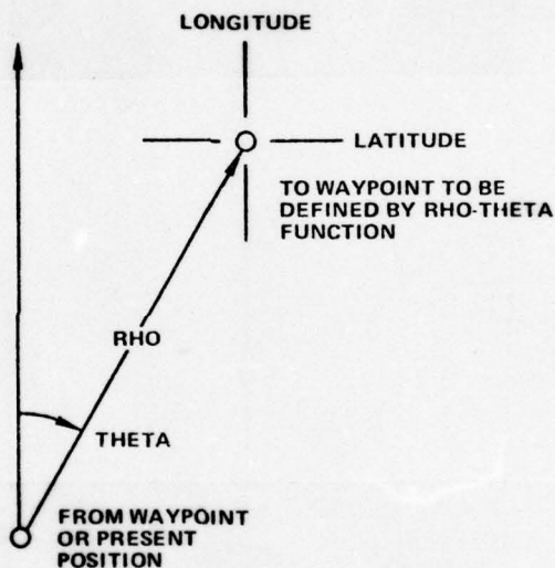
Figure A.5 Rho/Theta Steering Geometry
