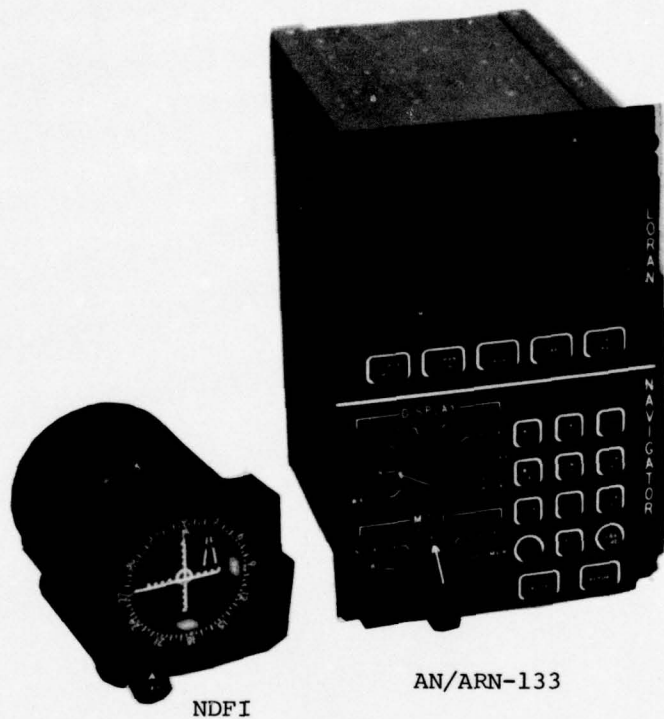
Figure A.6 TDL-AN/ARN-133 and NDFI Equipment Installed in USCG HH52 Aircraft
