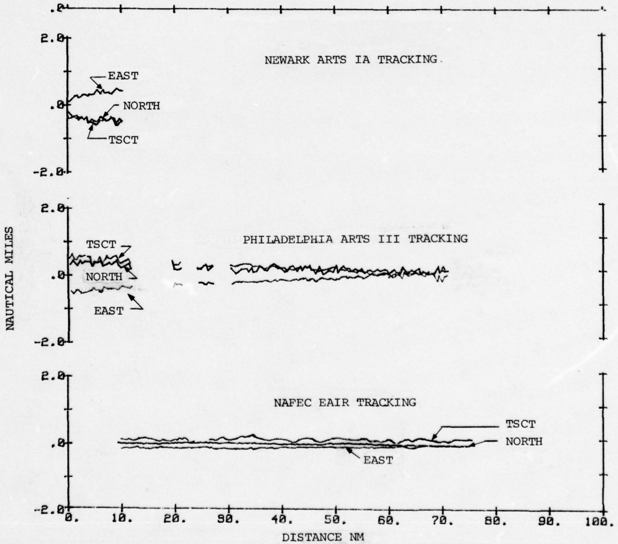
Figure 5.4 Comparison of ARTS IA, III and EAIR Accuracy
