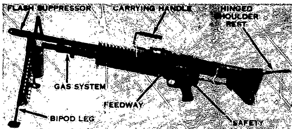
Figure 12. Machinegun, 7.62mm, M60 on bipod mount.
