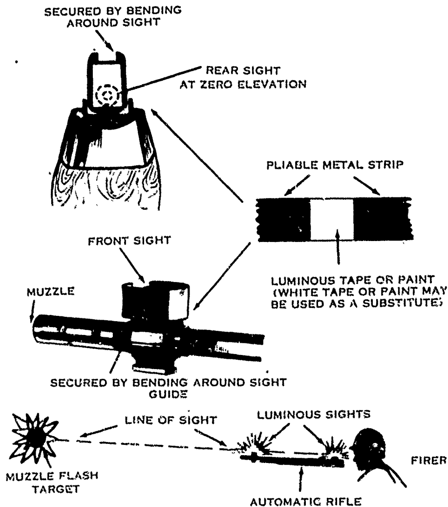
Figure 46. Field Expedient Night Sight and Sight Picture for the Automatic Rifle.
