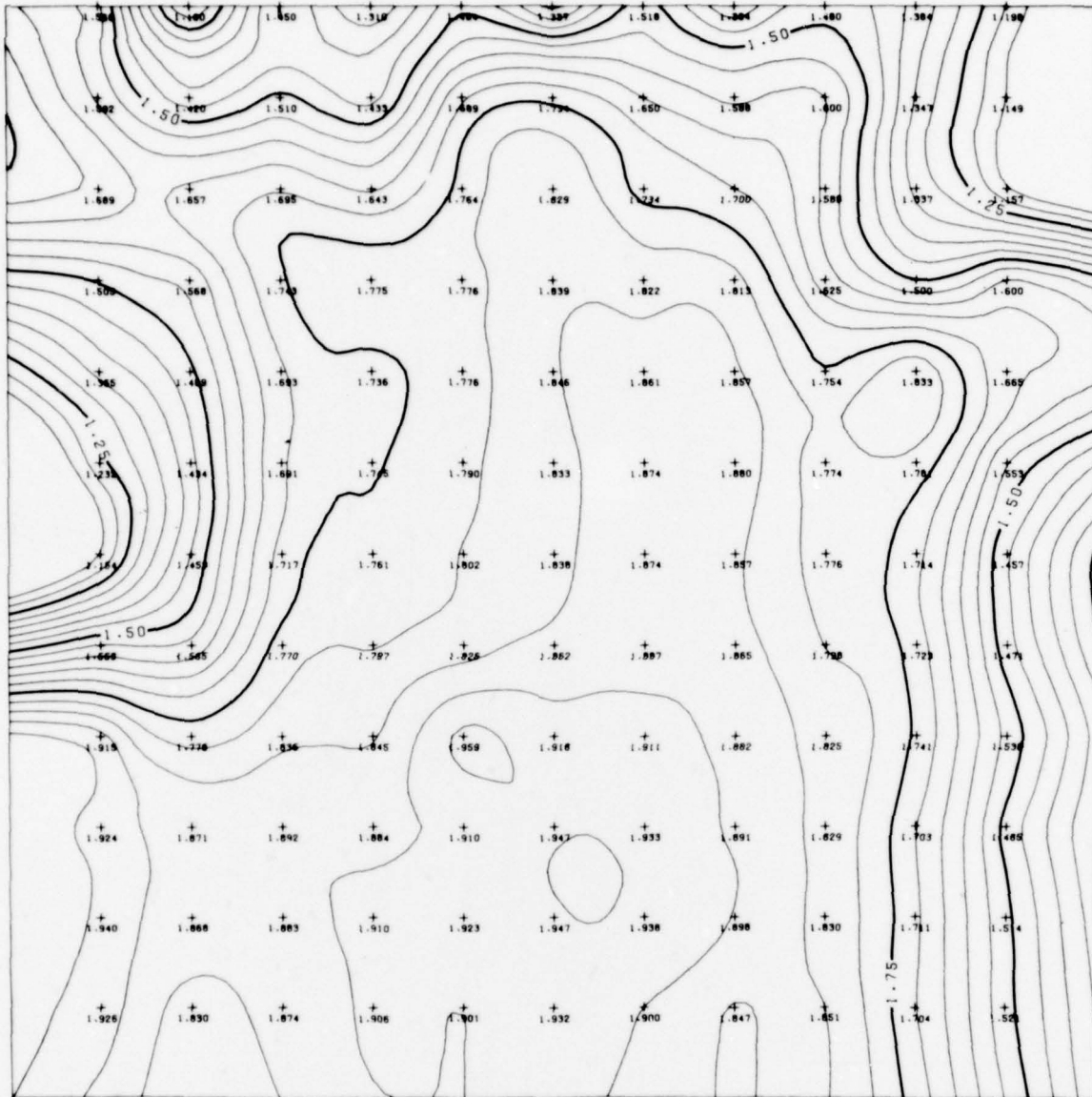
Figure 7. Haveg 41 Contours from Plenum A, Test 1, Motor L
